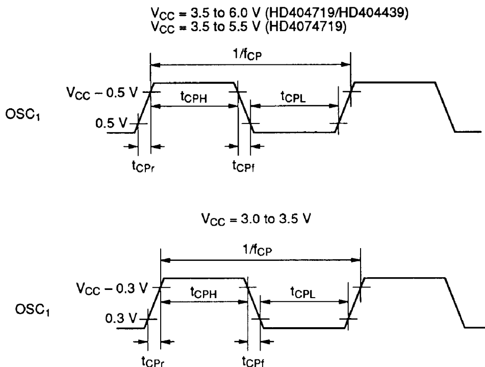
Figure 70 Oscillator Waveforms
