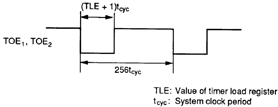
Figure 30 Variable-Duty Pulse Output Waveform
