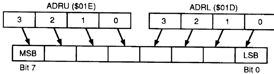
Figure 51 A/D Data Register
