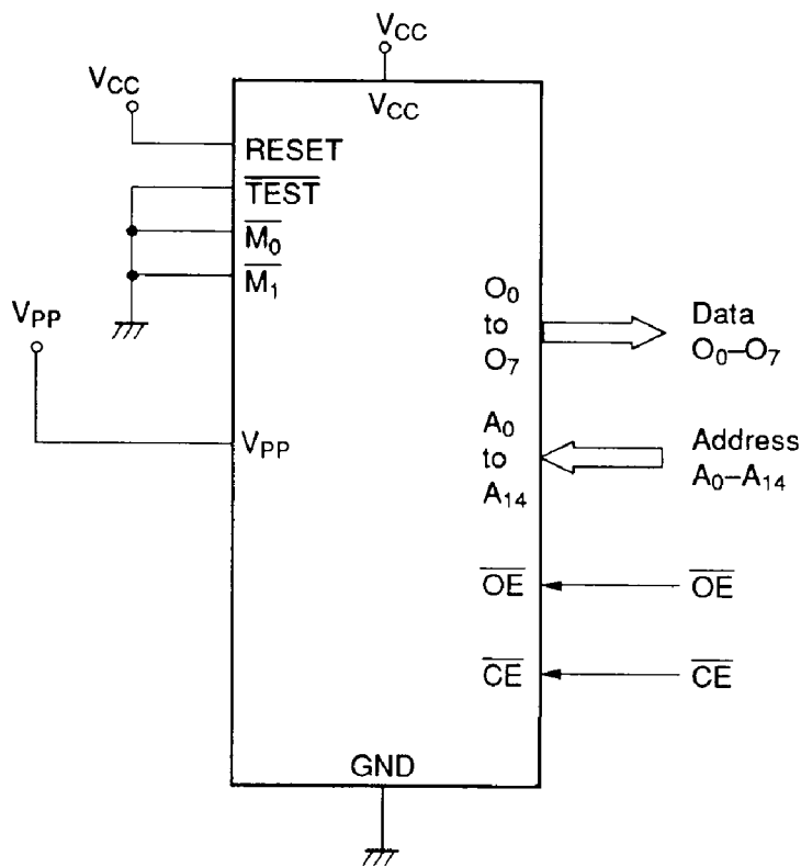
Figure 58 Connections for PROM Mode
