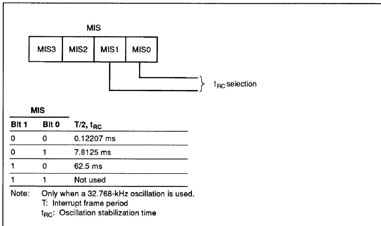
Figure 15 Miscellaneous Register
