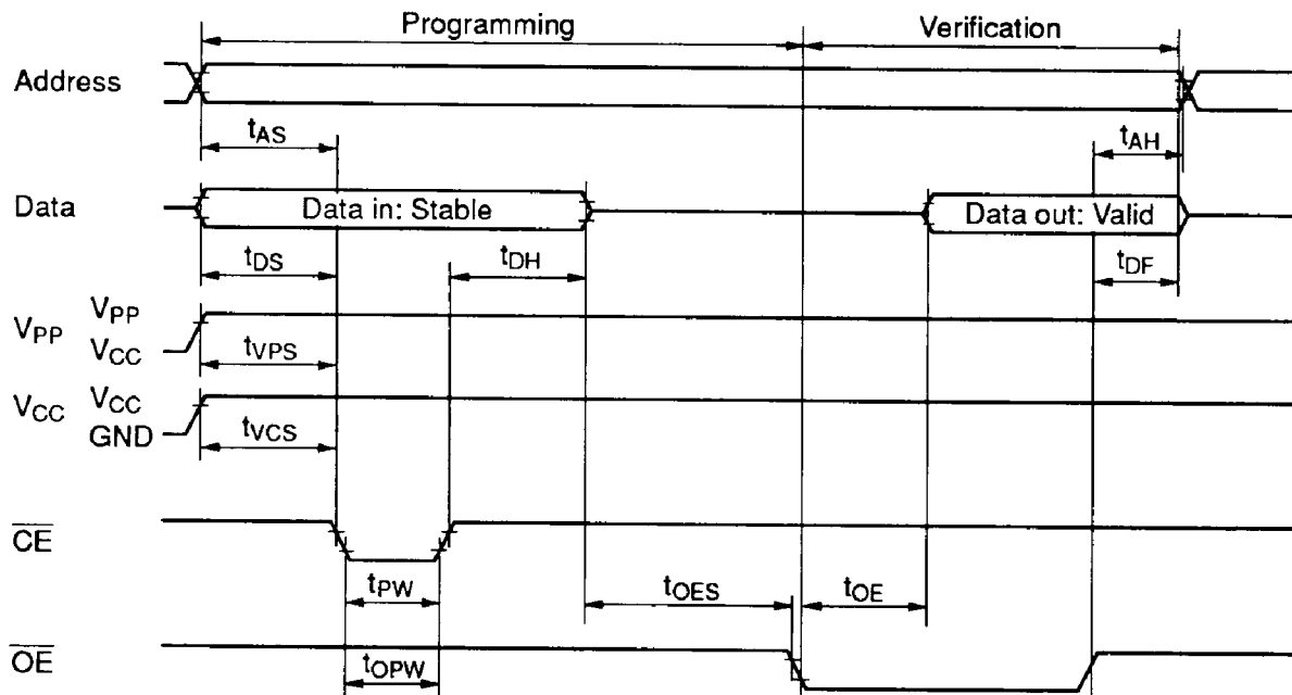
Figure 61 PROM Programming/Verification Timing
