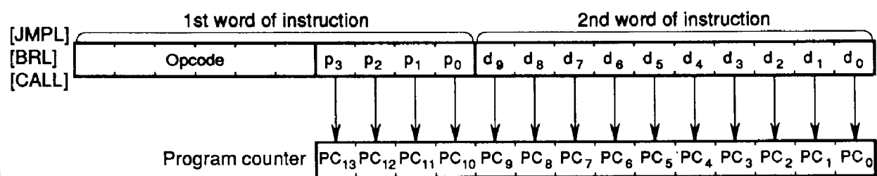
Direct Addressing
