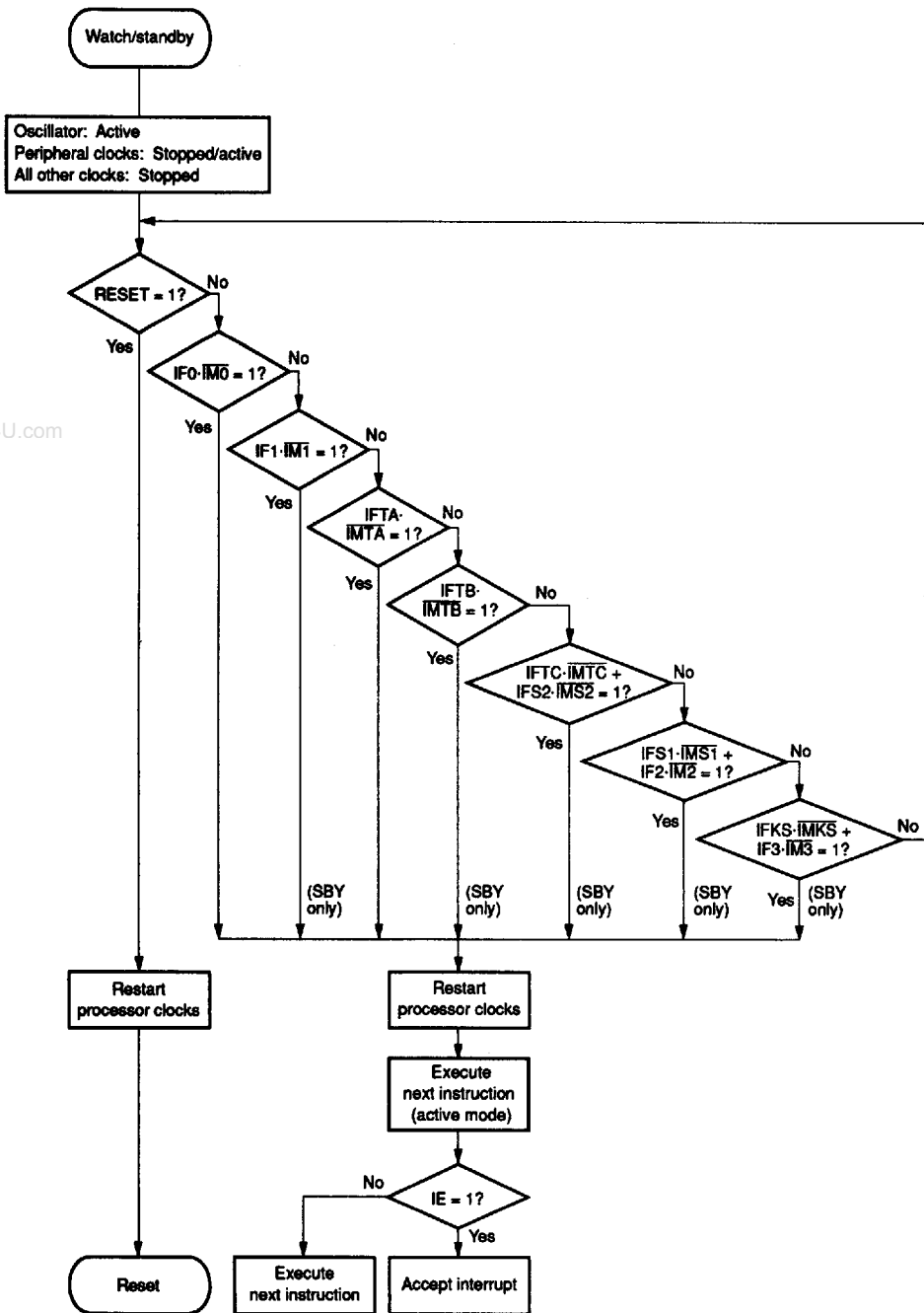
Figure 15 Flowchart of Watch and Standby Modes
