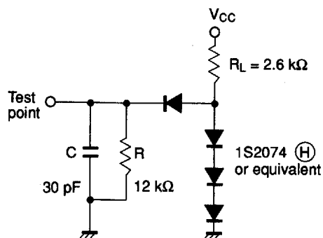
Figure 62 Timing Load Circuit
