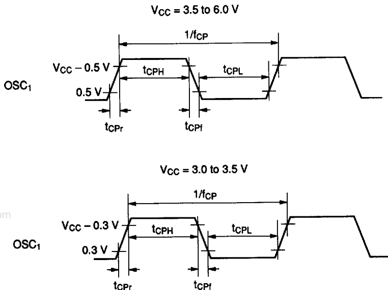
Figure 58 Oscillator Timing
