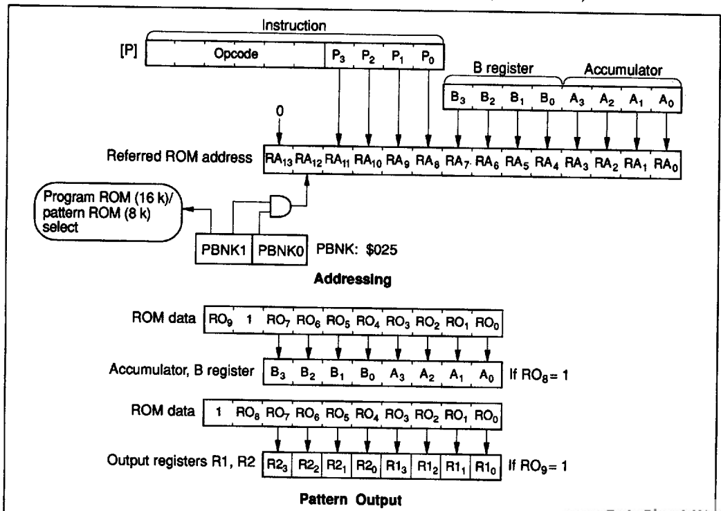
Figure 54-2 P Instruction (HD404720, HD4047420)
