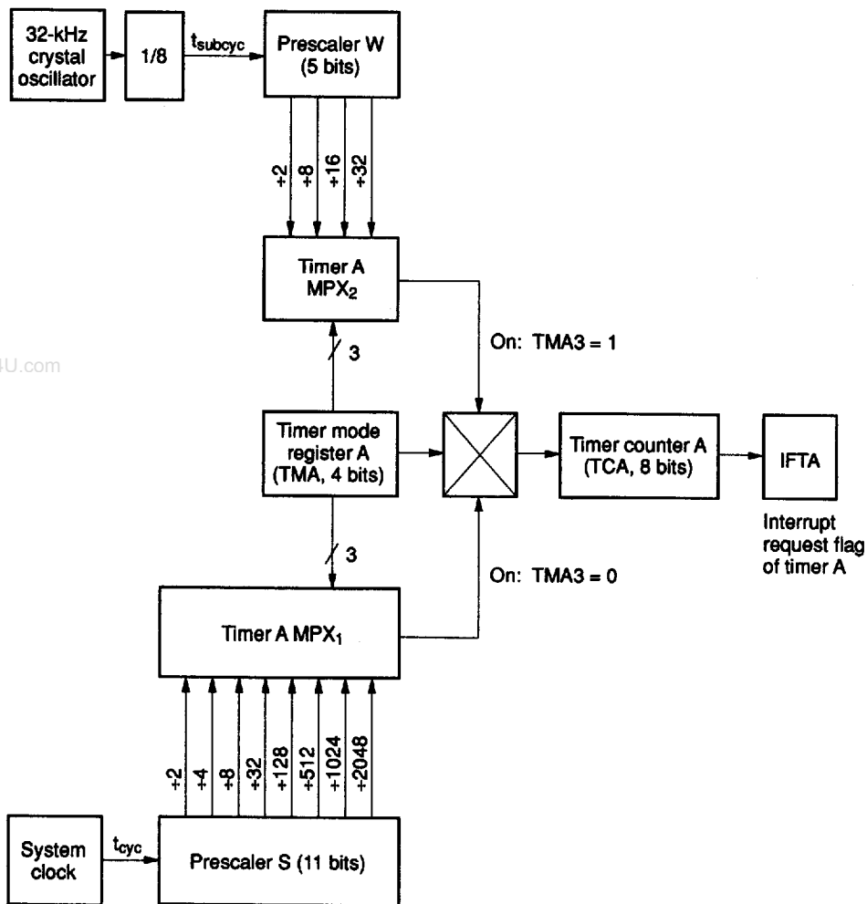
Figure 26 Block Diagram of Timer A
