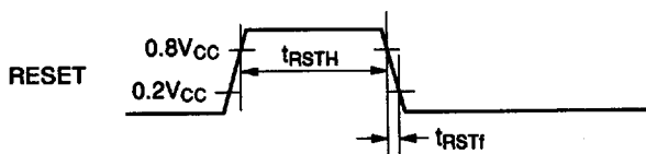
Figure 60 Reset Timing
