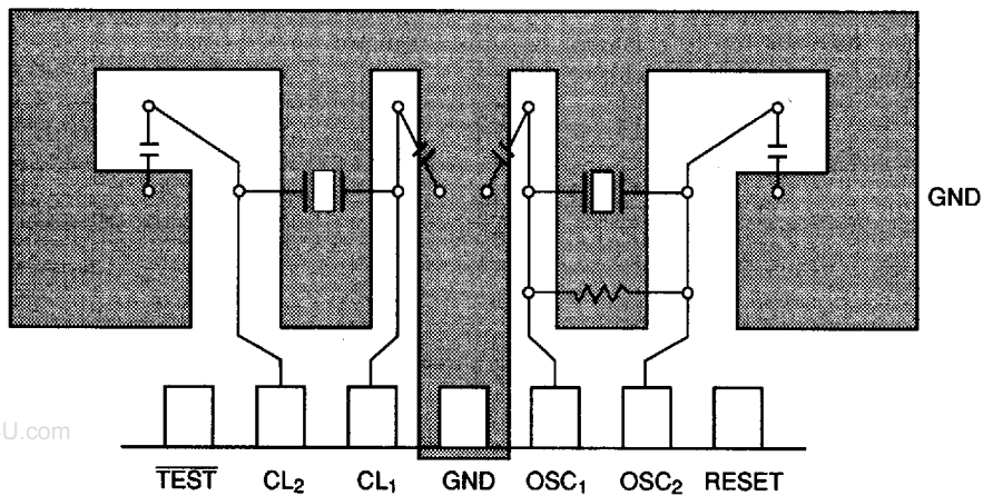
Figure 23 Typical Layout of Crystal or Ceramic Oscillator
