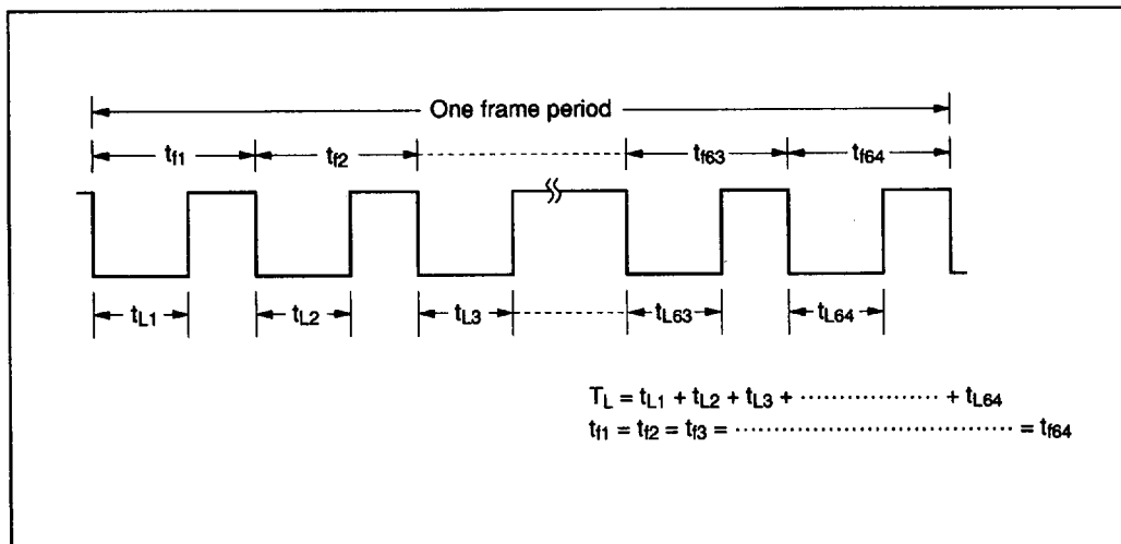
Figure 49 PWM Waveform
