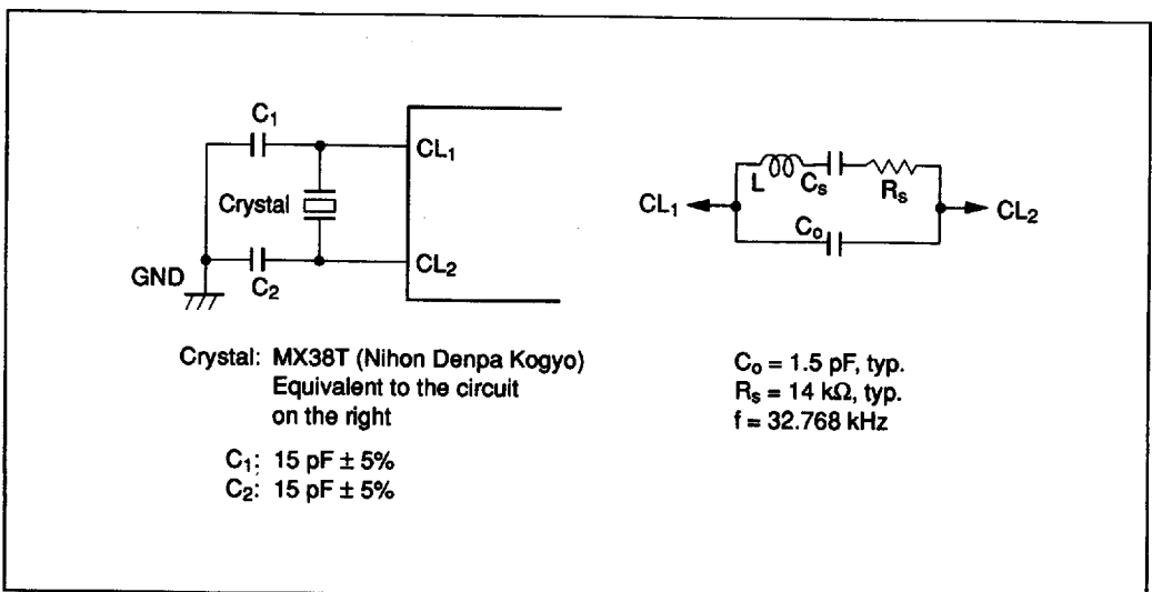
Figure 57 Oscillation Circuits (2)
