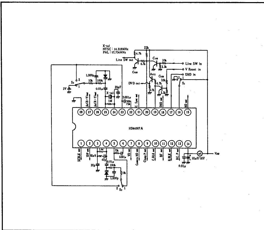
Figure 9 Test Circuit
