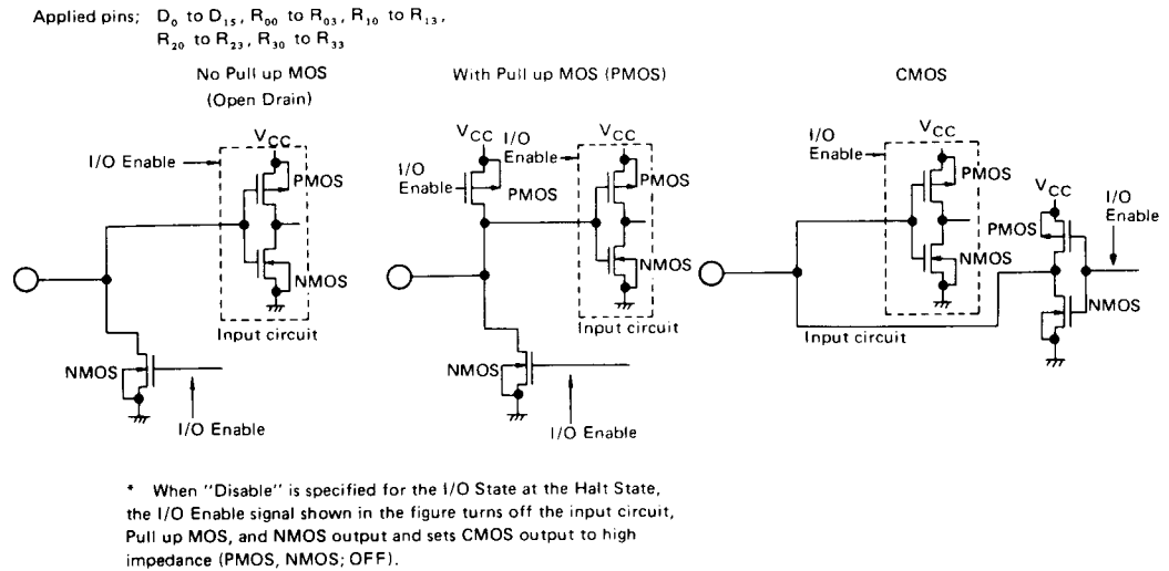
Figure 18 I/O Configuration
