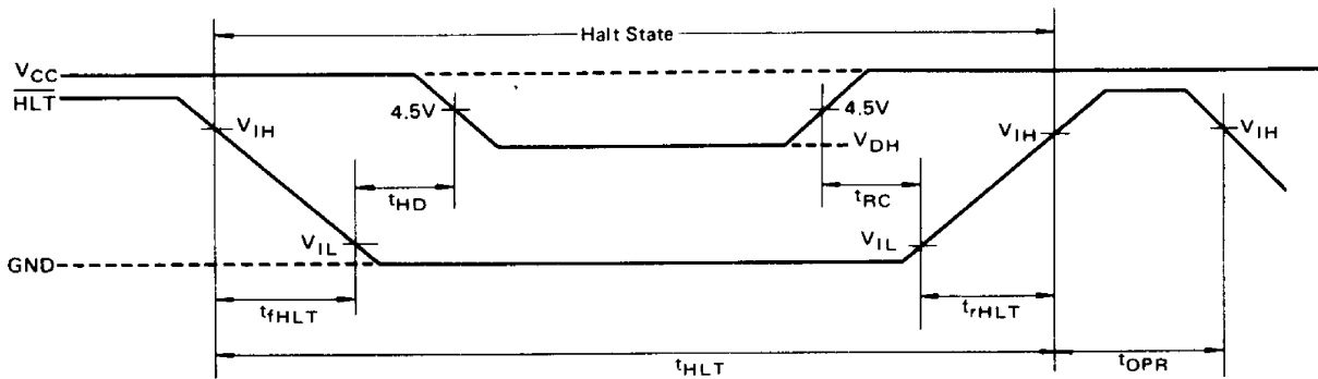
Figure 24 Halt Timing
