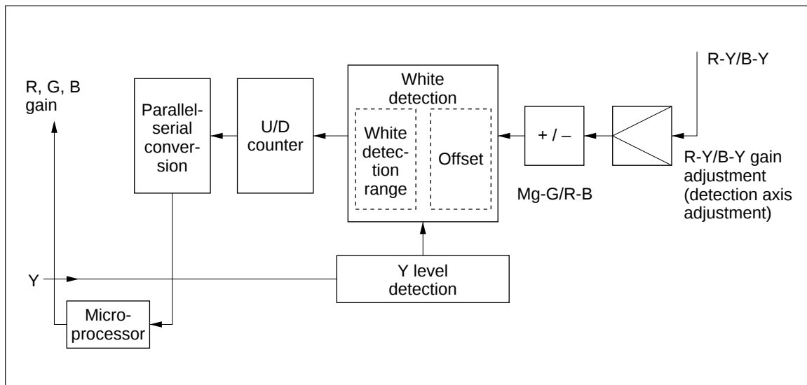
White Balance Detection Block Diagram
