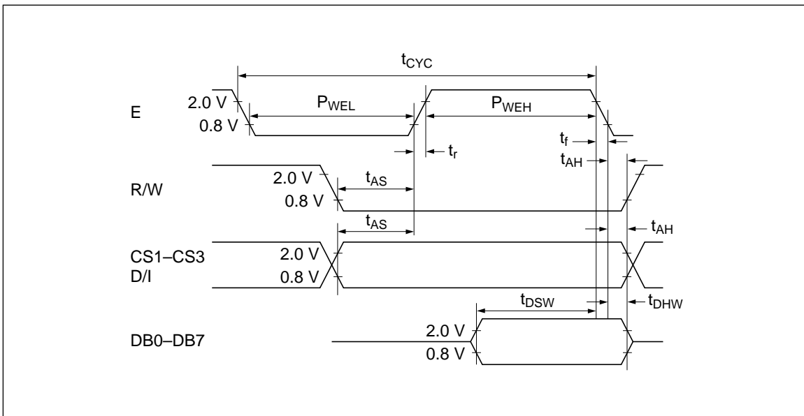
Figure 10 MPU Write Timing
