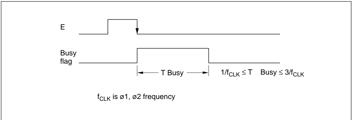
Figure 2 Busy Flag
