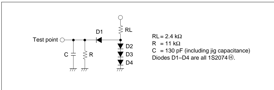
Figure 12 DB0-DB7: Load Circuit
