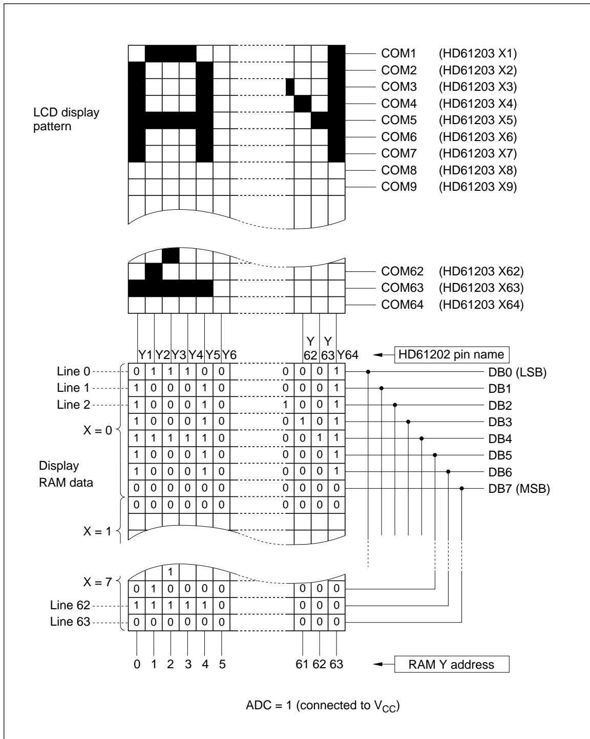
Figure 3 Relation between RAM Data and Display
