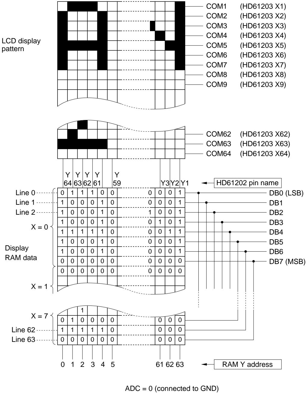
Figure 3 Relation between RAM Data and Display (cont)
