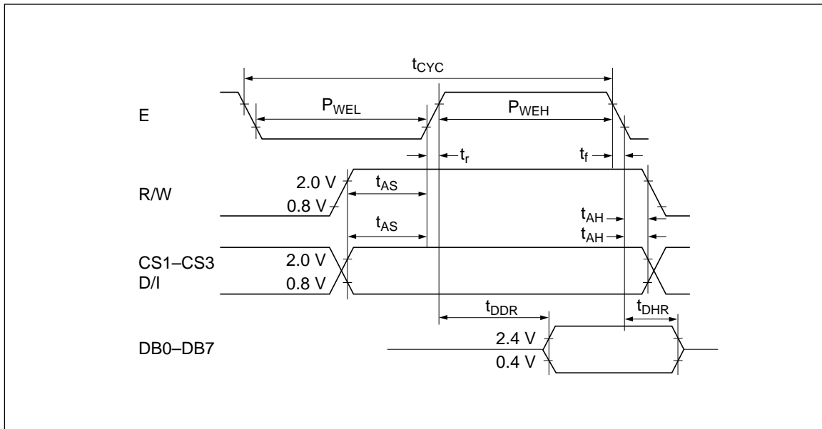
Figure 11 MPU Read Timing
