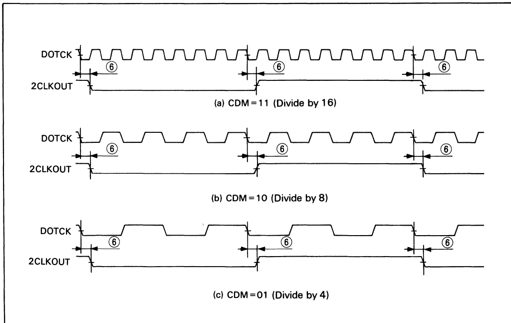
Figure 19. 2CLKOUT
