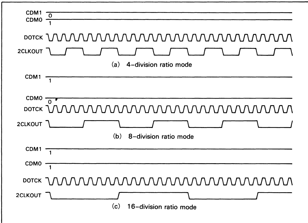
Figure 4. DOTCK Division
