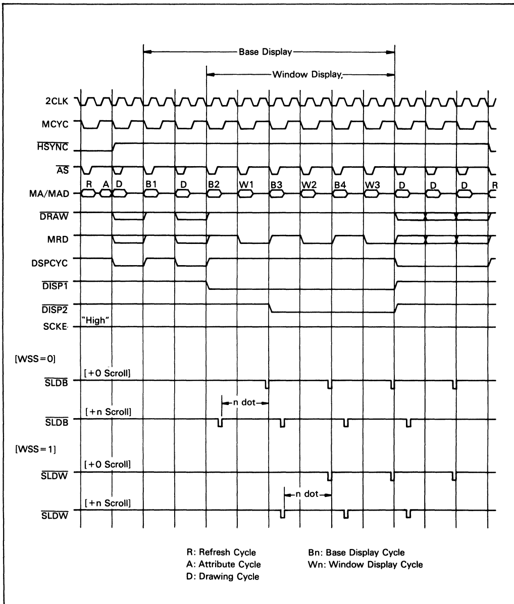
Figure 11. \overline{SLDB} and \overline{SLDW} Timing (Dual Access Mode 1)
