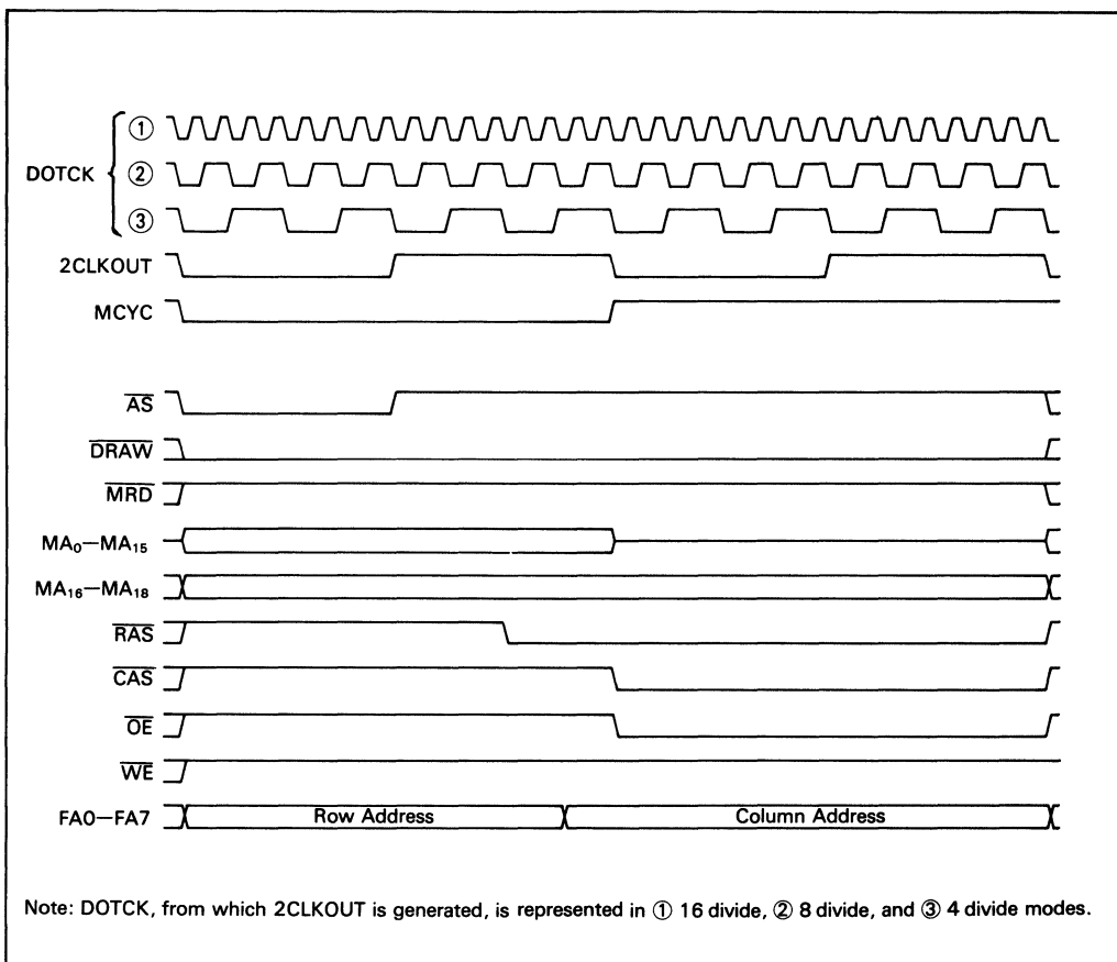
Figure 6. Read Cycle Timing
