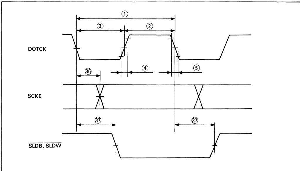
Figure 18. Clock
