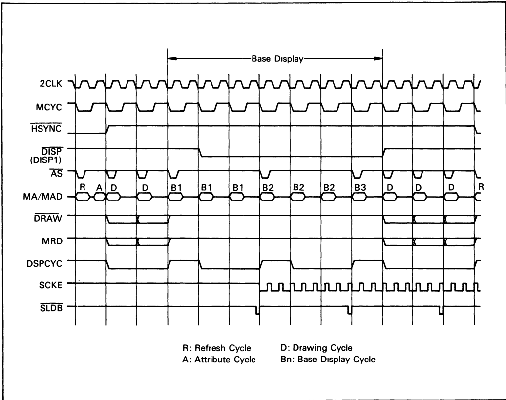
Figure 12. Zoom Display Timing (Single Access Mode, Triple Zoom)
