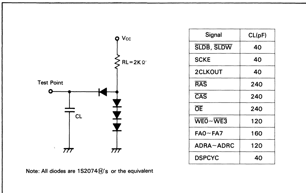
Figure 24. Test Load Circuit
