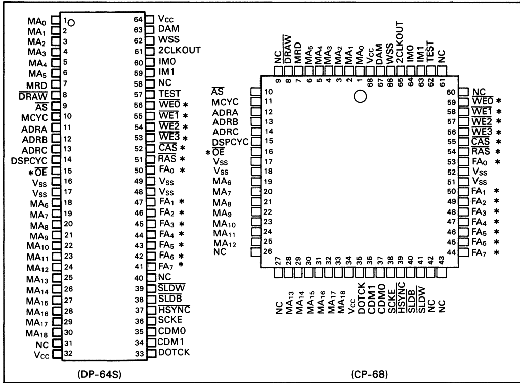
Figure 1. Pin arrangement
