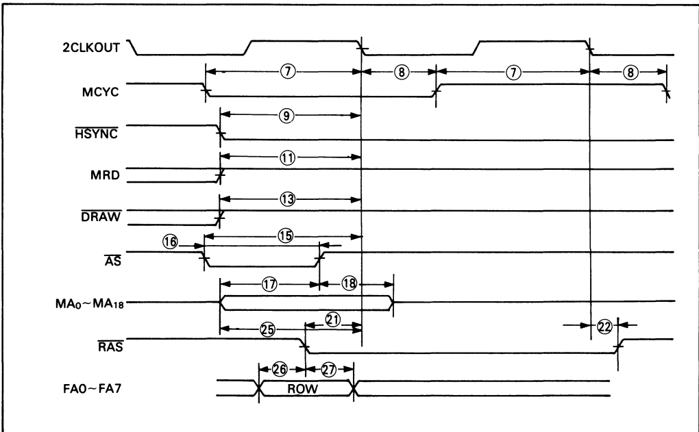
Figure 22. Refresh Cycle
