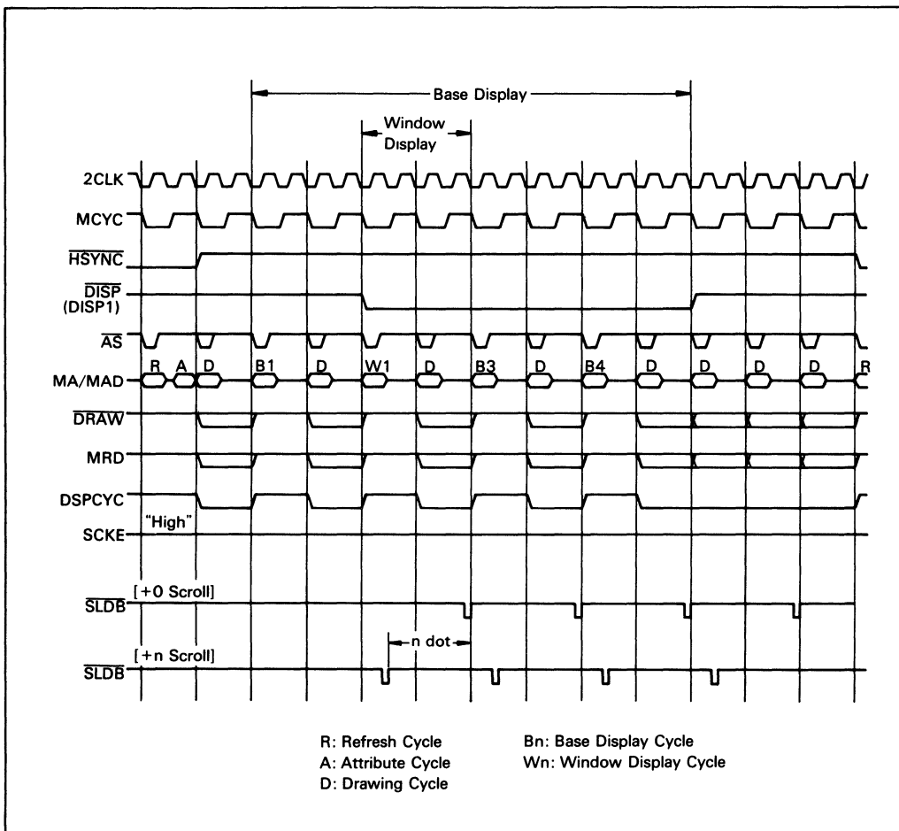
Figure 10. SLDB Timing (Dual Access Mode 0)
