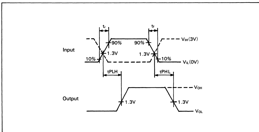
Figure 25. Input/Output waveforms
