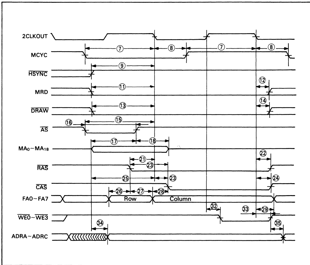
Figure 21. Memory Write Cycle
