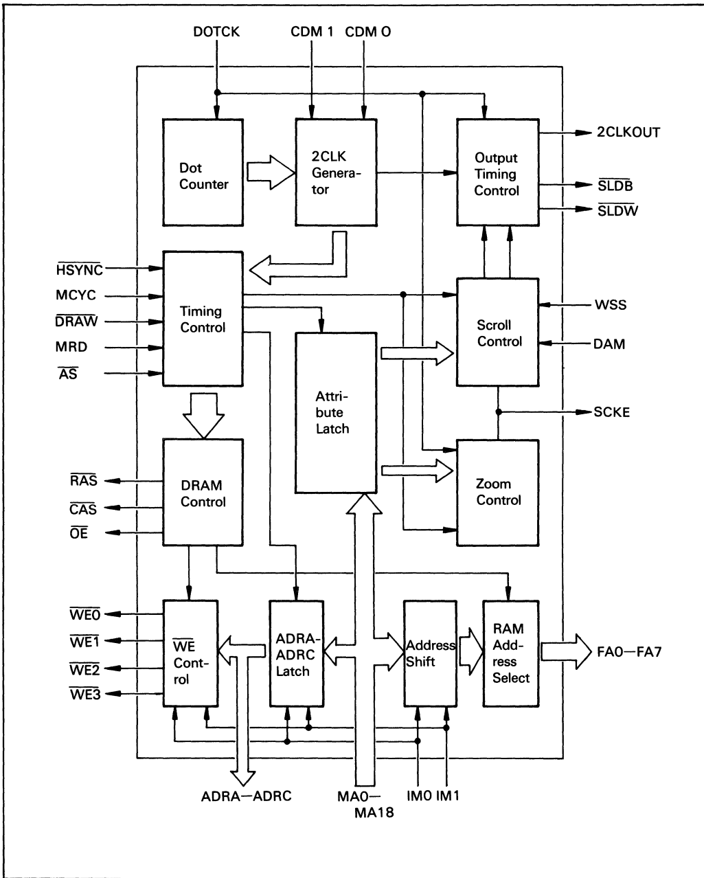
Figure 2. GMIC Block Diagram
