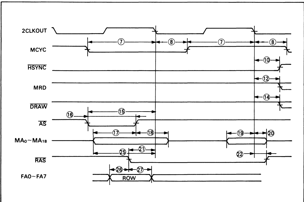
Figure 23. Attribute Cycle
