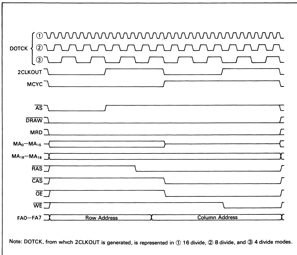
Figure 7. Write Cycle Timing
