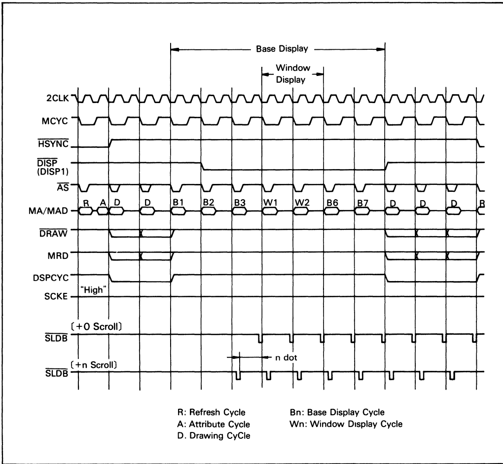
Figure 9. SLDB Timing (Single Access Mode)
