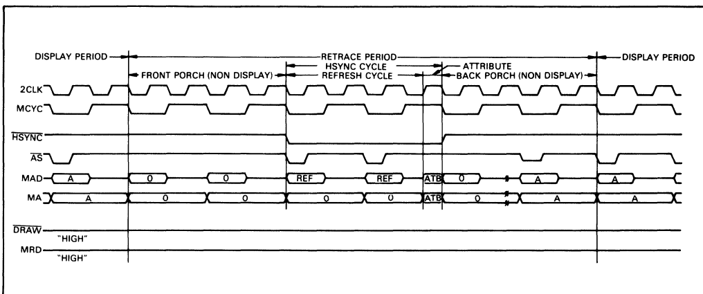
Figure 16. DRAM Refresh and Attribute Control Data Output (Single Access Mode)
