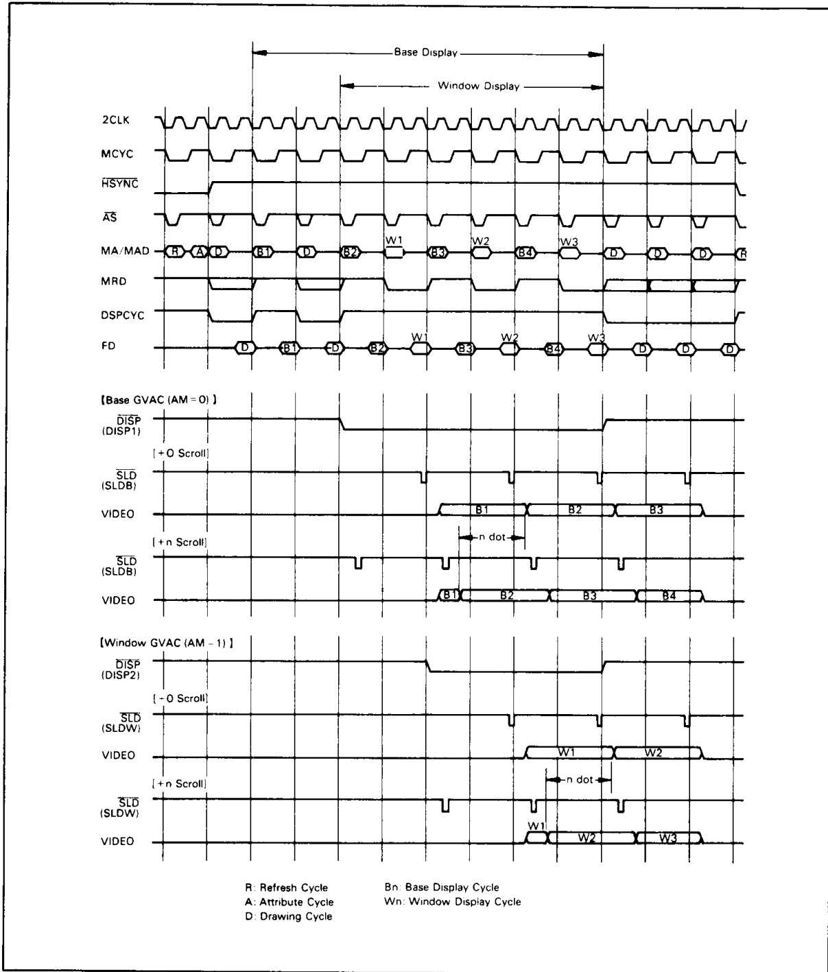
Figure 11. Video Output Timing (Dual Access Mode 1)
