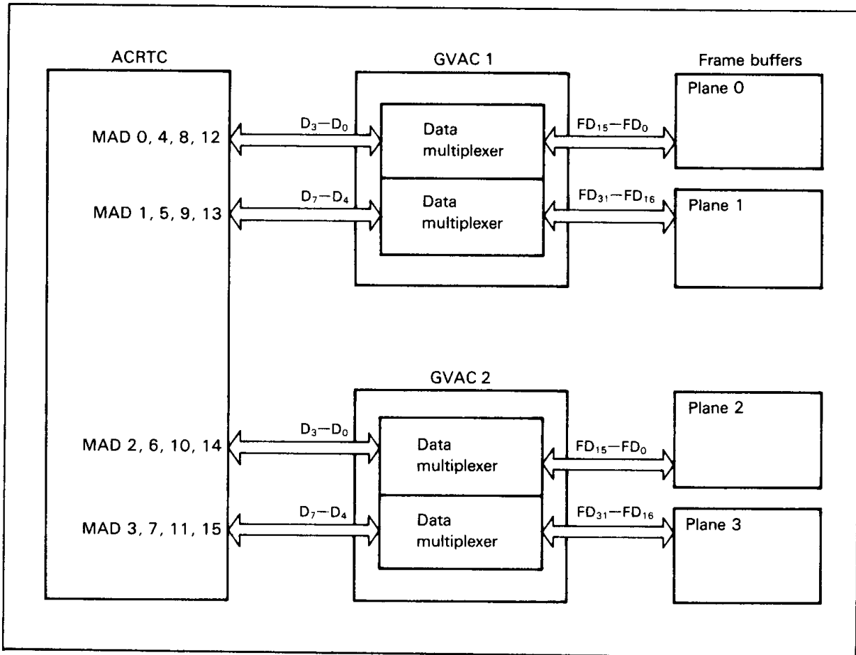
Figure 6. FD Pin Connection (MOD1, MOD0 = 00)
