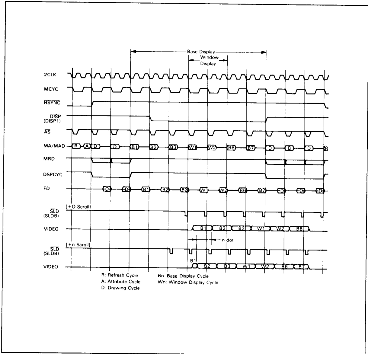
Figure 9. Video Output Timing (Single Access Mode)
