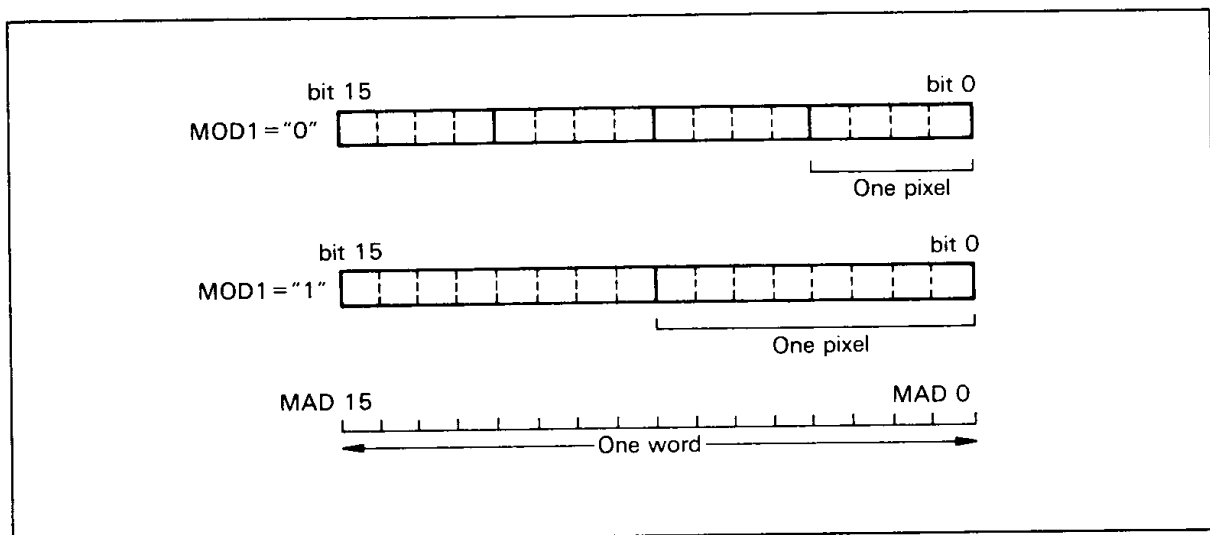
Figure 7. Pixel Data and MOD1
