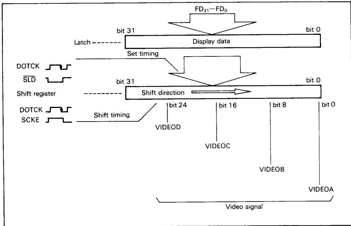
Figure 8. Video Signal Generation
