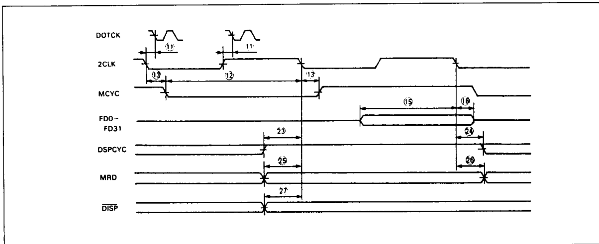
Figure 21. Display Cycle
