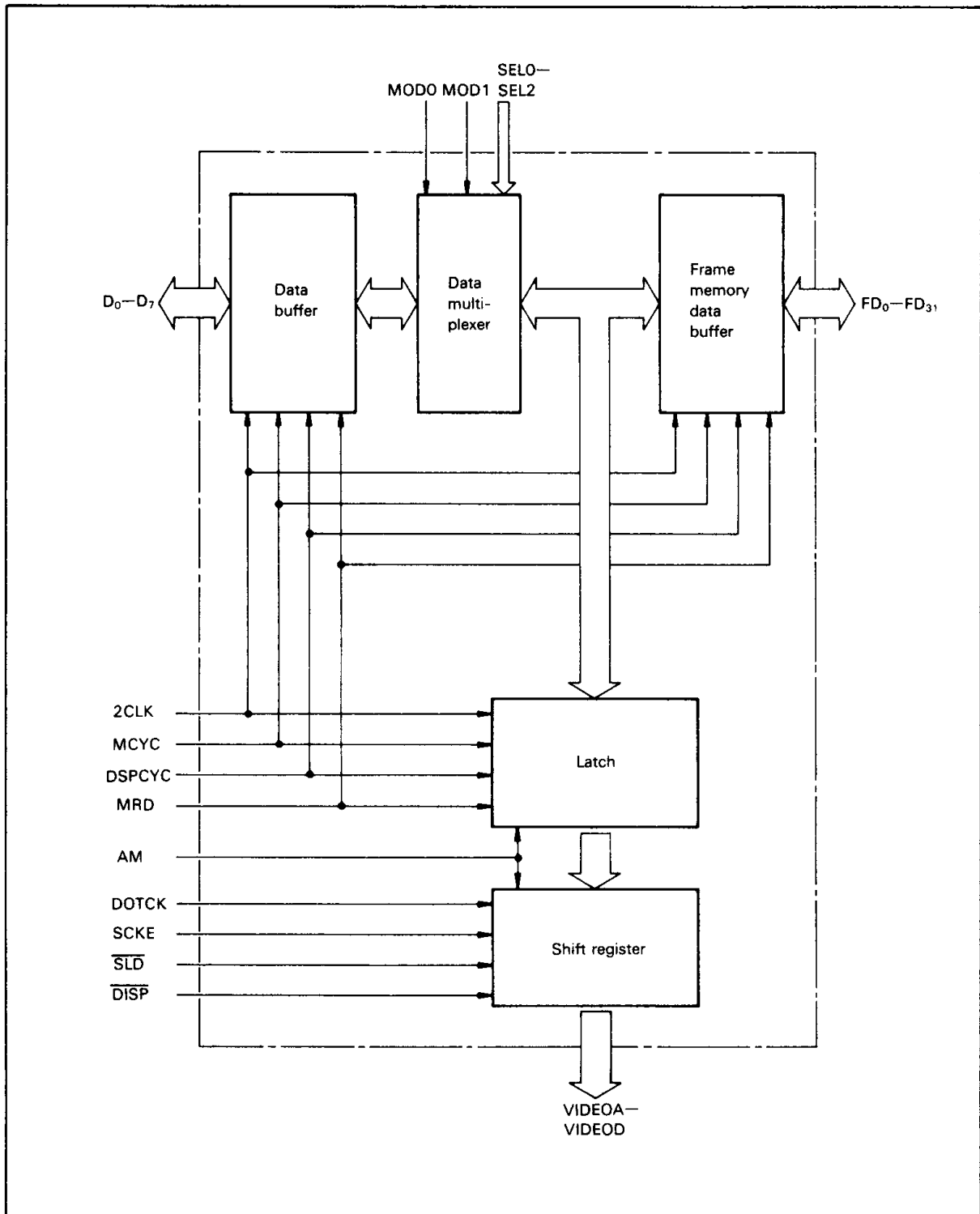
Figure 2. GVAC Block Diagram
