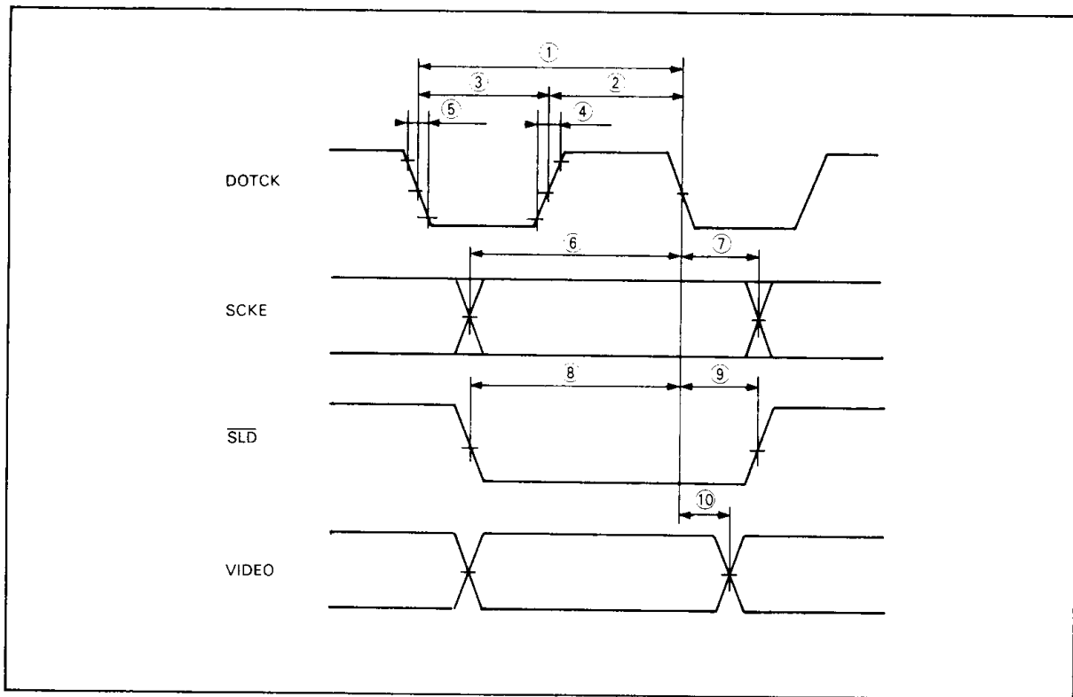
Figure 18. Dot Clock
