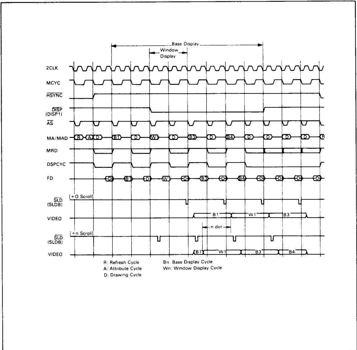
Figure 10. Video Output Timing (Dual Access Mode 0)
