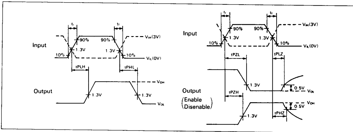
Figure 23. Input/Output Waveforms
