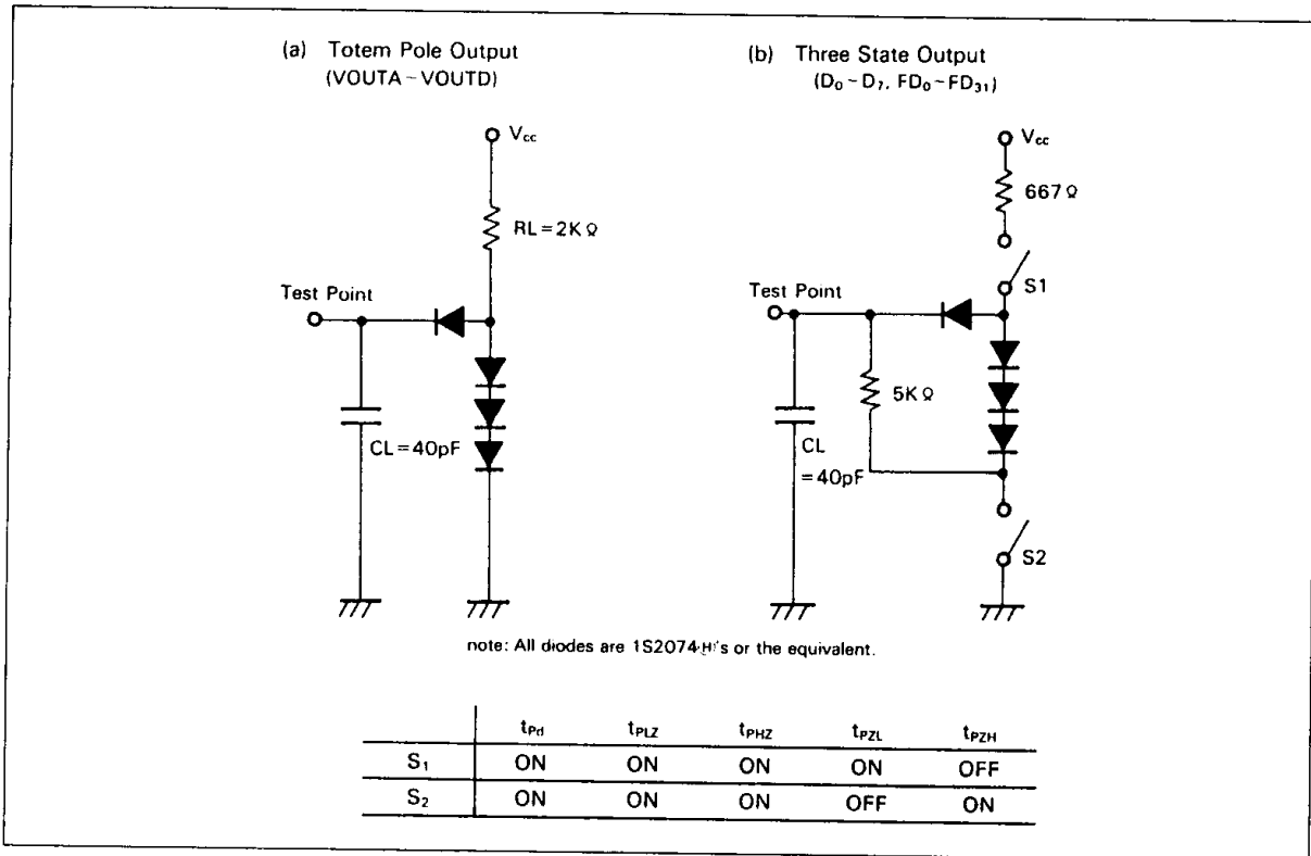
Figure 22. Test Load Circuit
