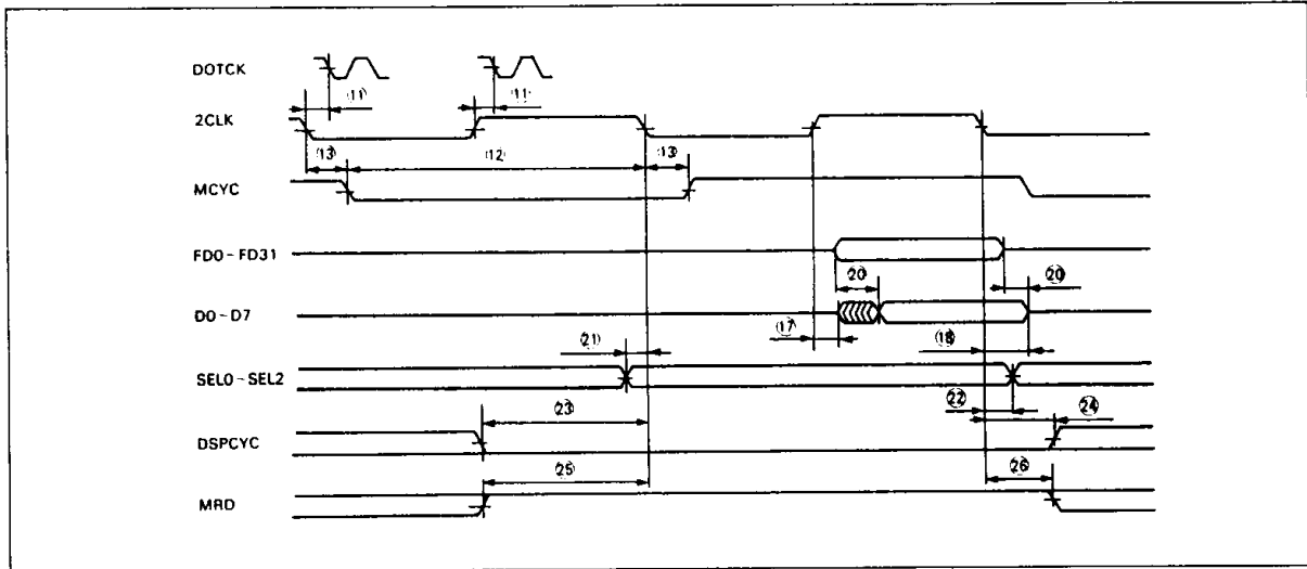
Figure 19. Drawing Read Cycle
