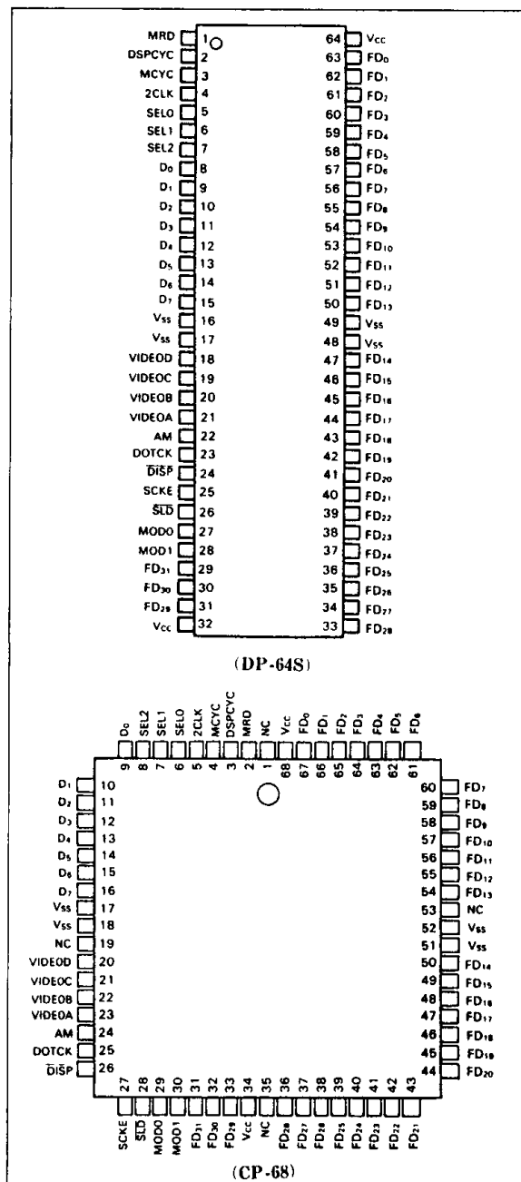
Figure 1. Pin Arrangement
