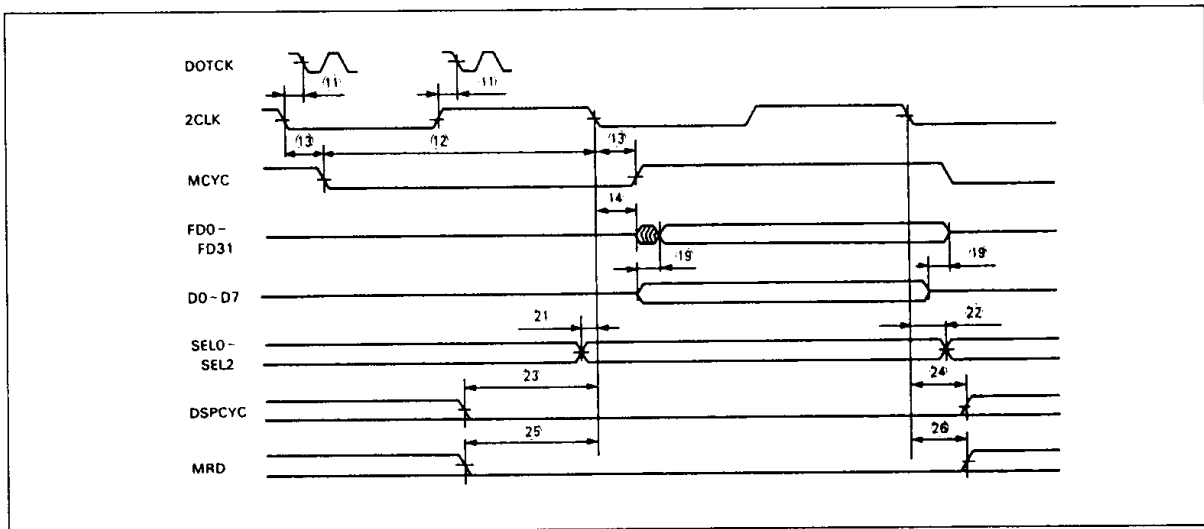
Figure 20. Drawing Write Cycle
