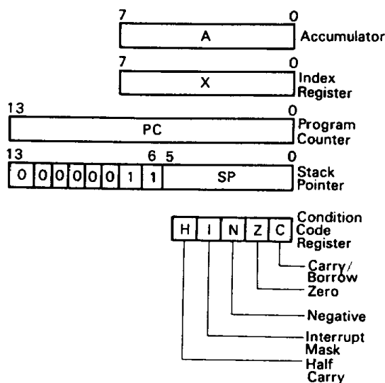
Figure 8 Programming Model
