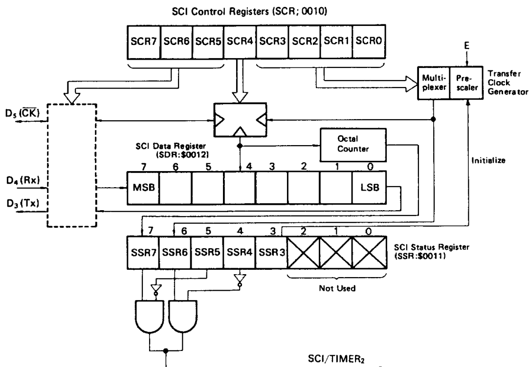
Figure 12 SCL Block Diagram
