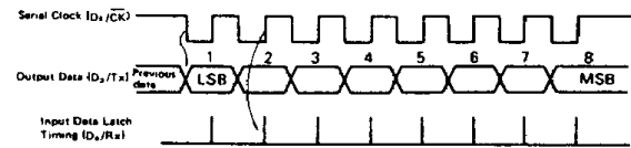
Figure 13 SCI Timing
