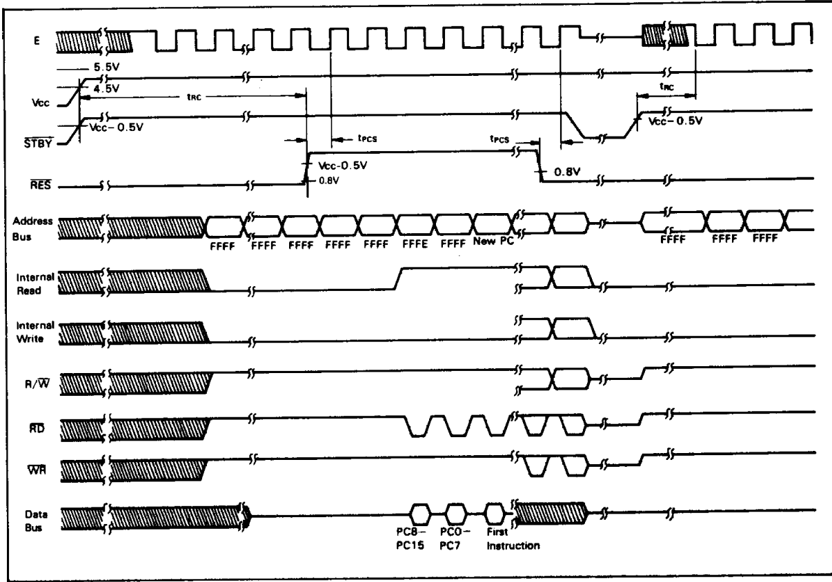
Figure 53. Reset Timing
