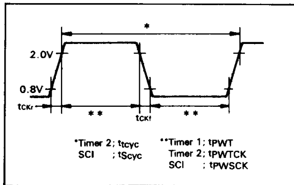
Figure 48. Timer 1 · 2, SCI Input Clock Timing
