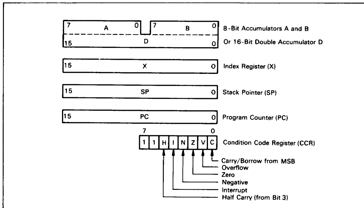
Figure 2. CPU Registers
