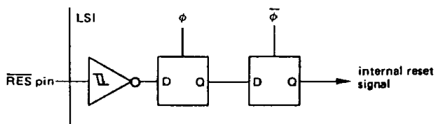
Figure 59 \overline{\text{RES}} circuit
