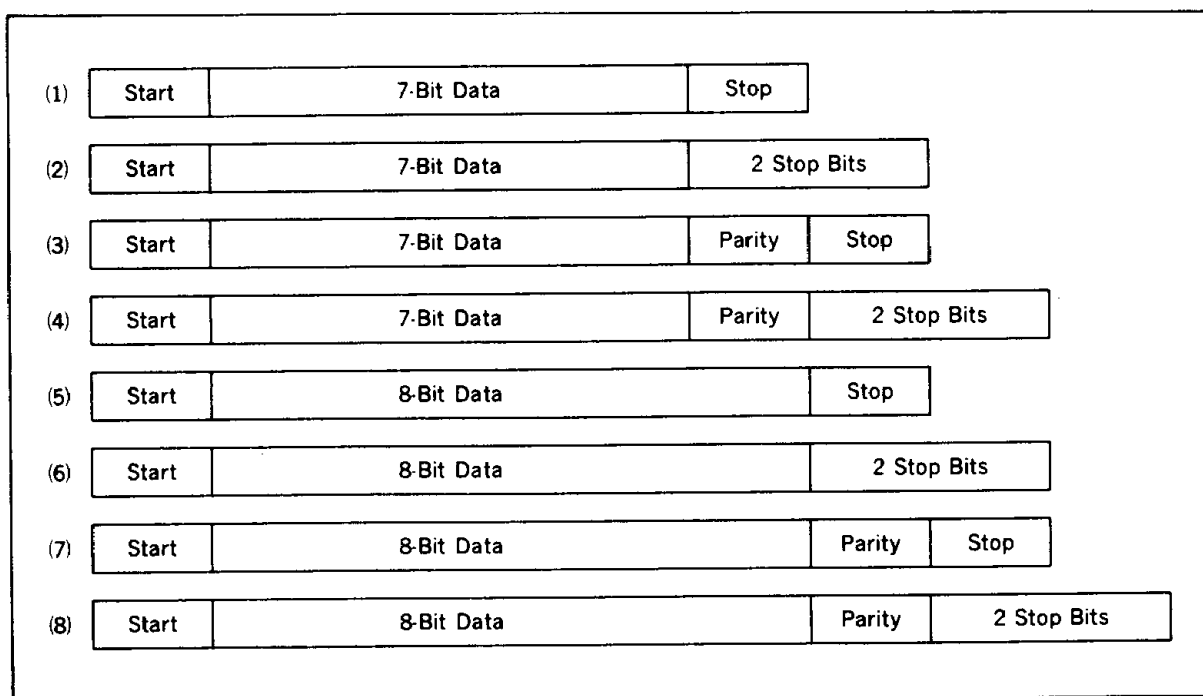
Figure 32. Asynchronous Formats
