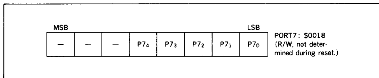
Figure 25. Port 7 Register
