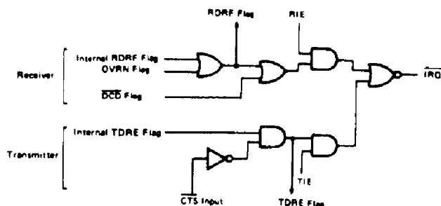
Figure 14 \overline{\text{IRQ}} Internal Circuit
