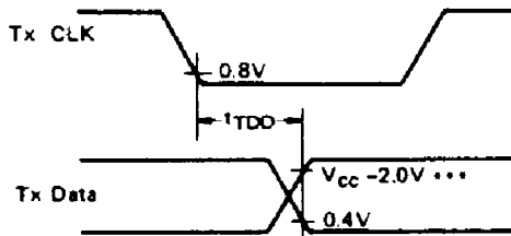
Figure 3 Transmit Data Output Delay
