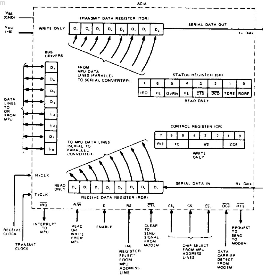
Figure 13 Internal Structure of ACIA
