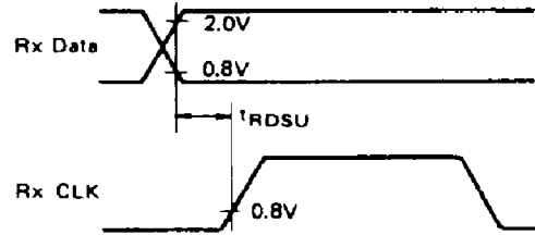
Figure 4 Receive Data Setup Time (÷1 Mode)
