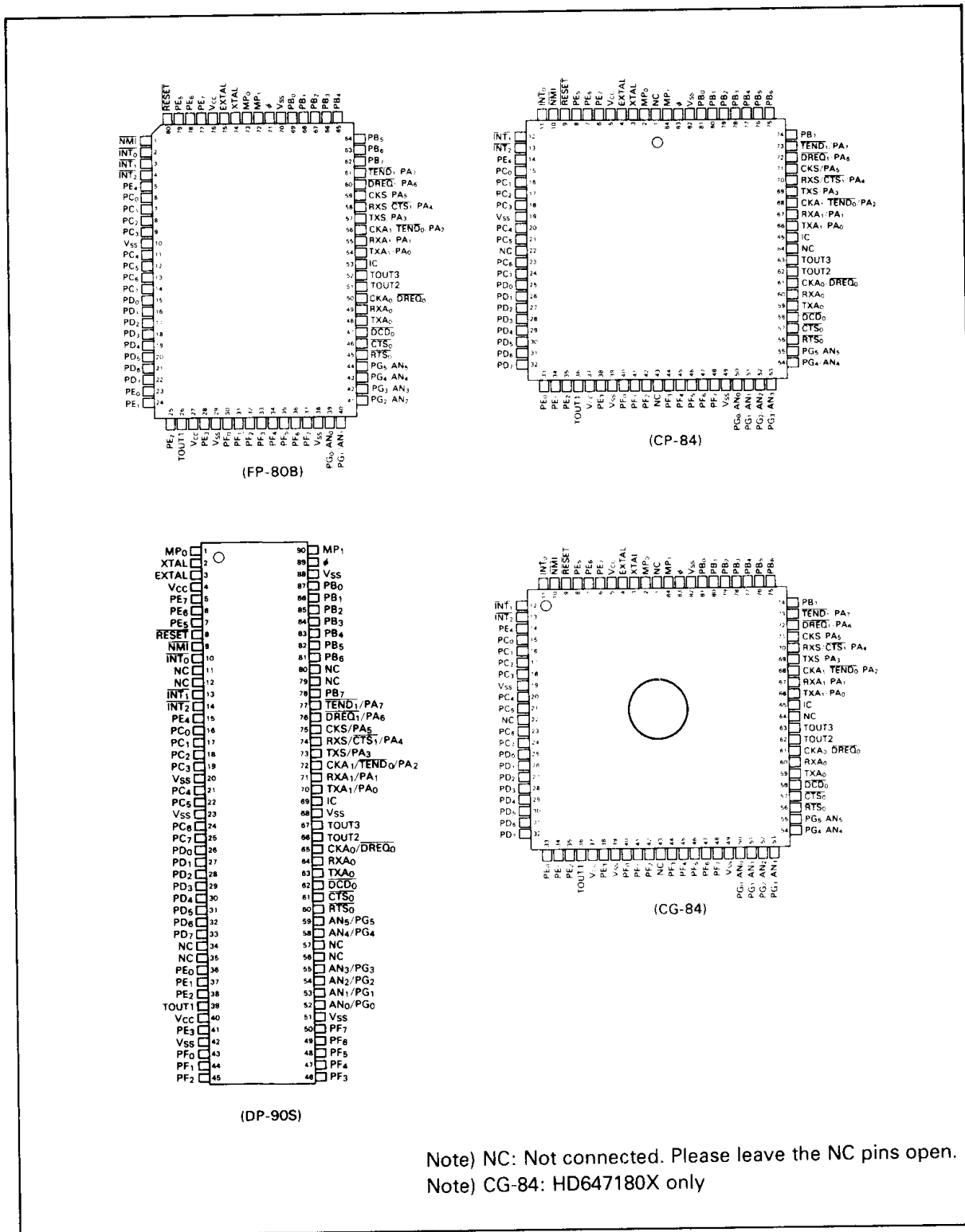
Figure 1. Pin Assignment
