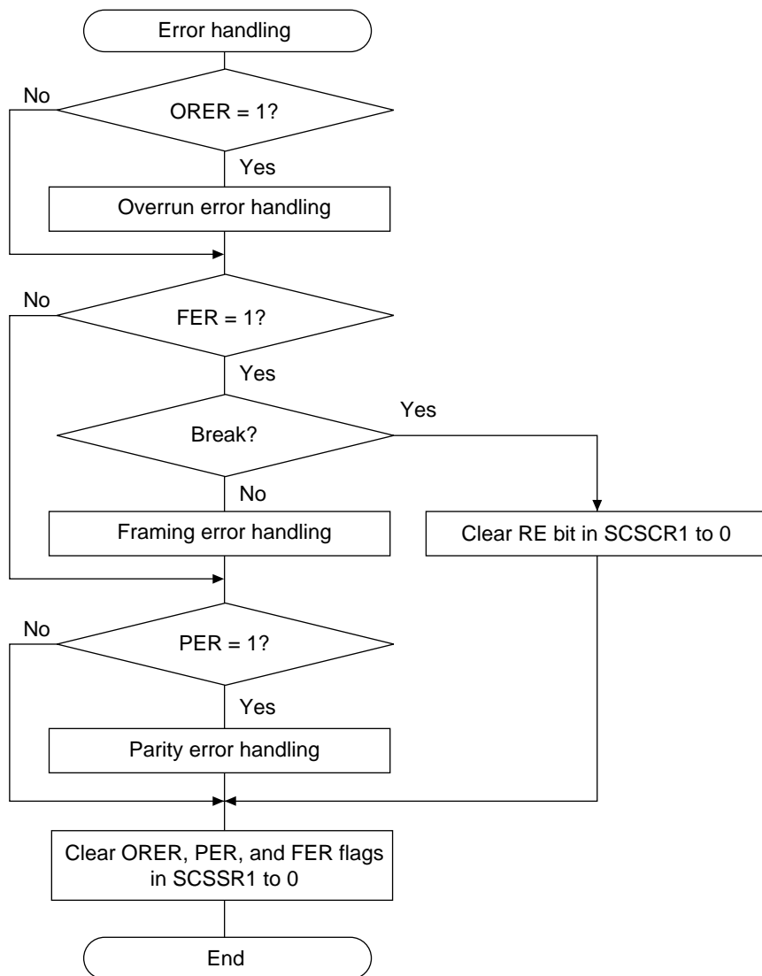
Figure 15.10 Sample Serial Reception Flowchart (2)
