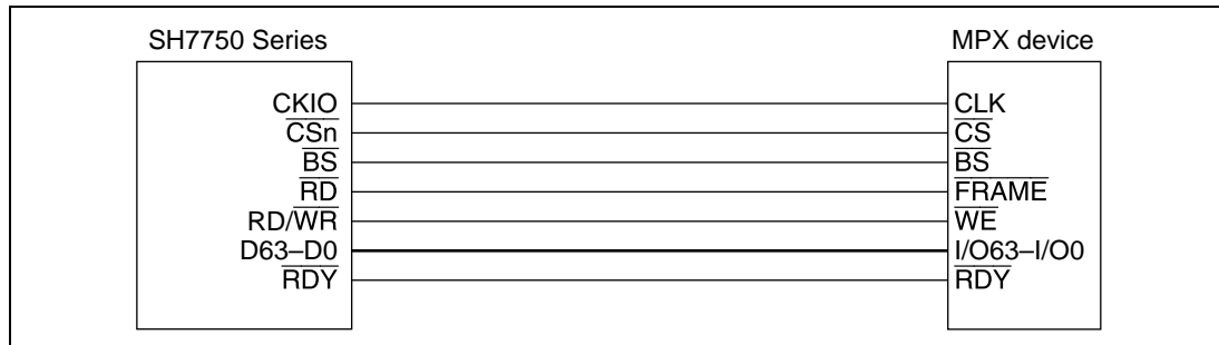
Figure 13.56 Example of 64-Bit Data Width MPX Connection
