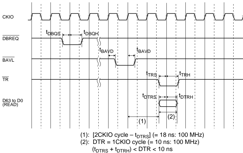
Figure 22.66(b) \overline{\text{DBREQ}}/\overline{\text{TR}} Input Timing and \overline{\text{BAVL}} Output Timing
