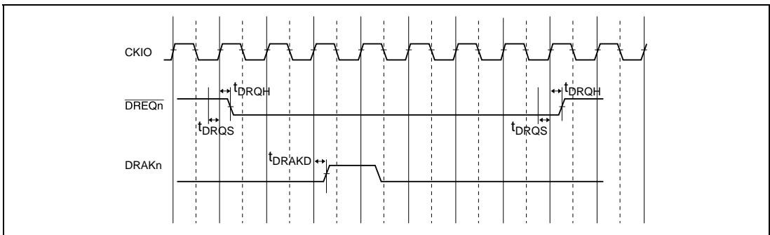
Figure 22.66(a) \overline{DREQ} /DRAK Timing
