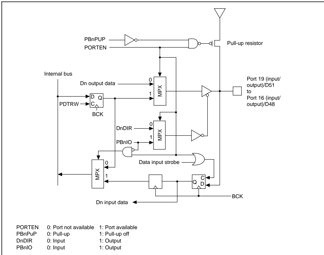
Figure 18.2 4-Bit Port
