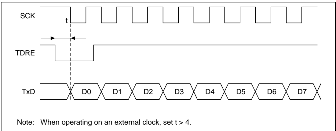
Figure 15.25 Example of Synchronous Transmission by DMAC
