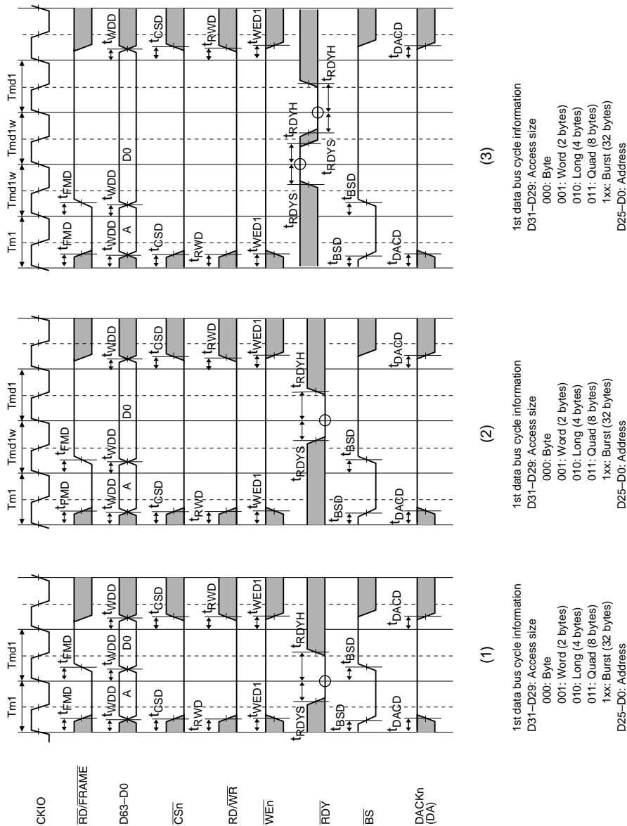
Figure 23.54 MPX Basic Bus Cycle: Write
