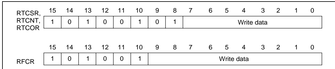
Figure 13.5 Writing to RTCSR, RTCNT, RTCOR, and RFCR
