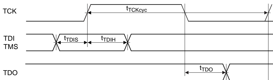
Figure 23.67 H-UDI Data Transfer Timing
