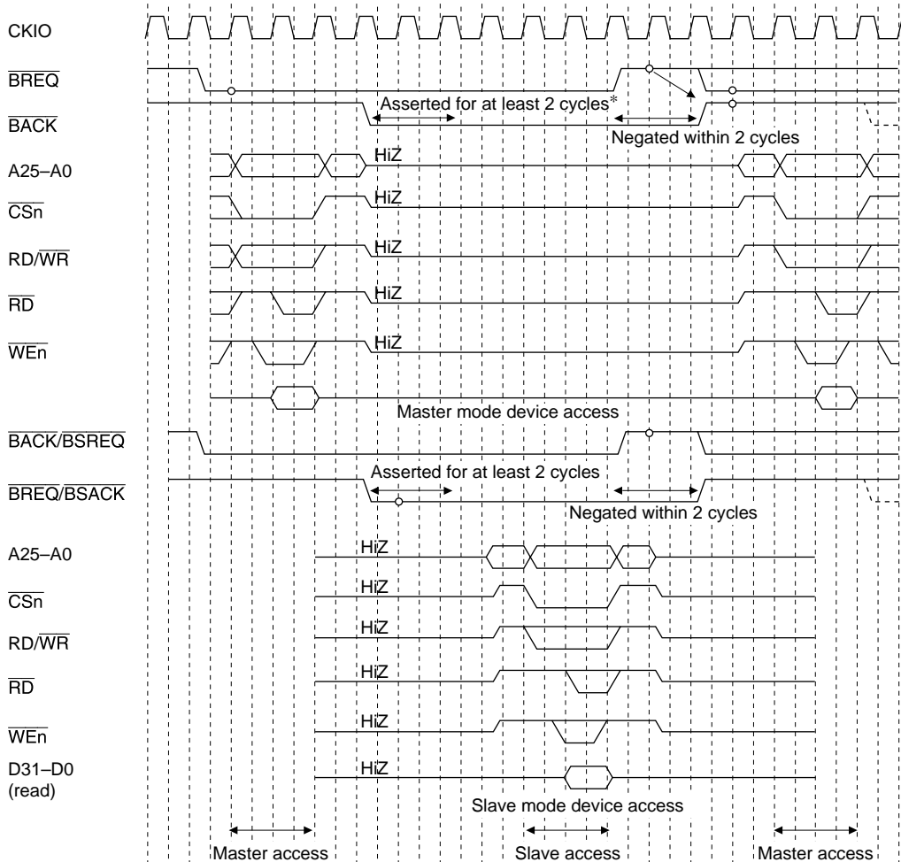
Figure 13.73 Arbitration Sequence
