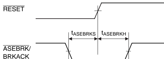
Figure 23.66 RESET Hold Timing
