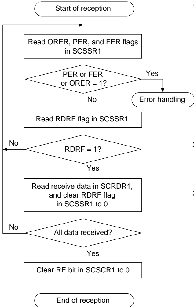
Figure 15.10 Sample Serial Reception Flowchart (1)
