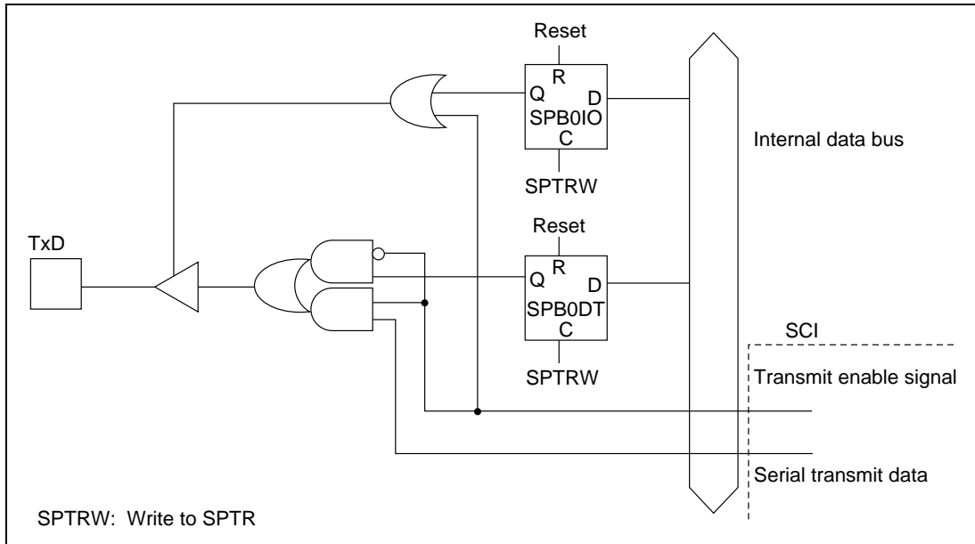
Figure 18.4 TxD Pin
