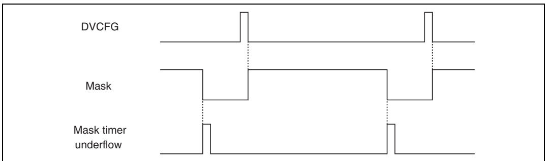
Figure 26.67 Mask Signal
