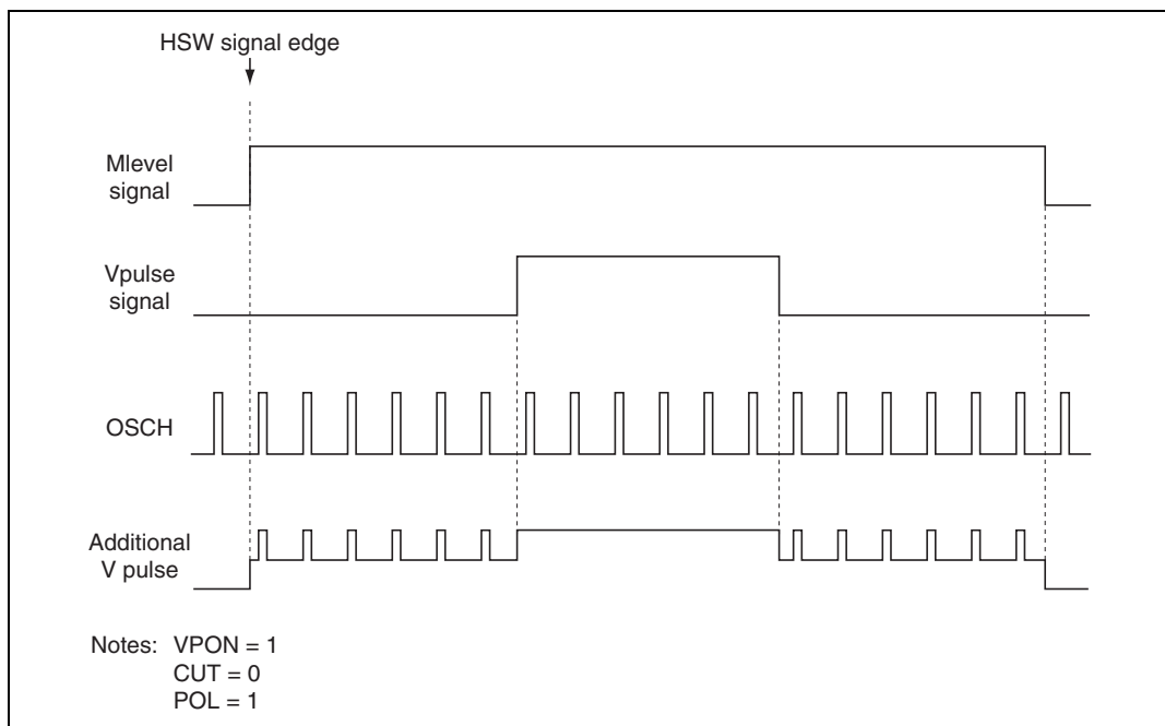
Figure 26.45 Additional V Pulse when Positive Polarity Is Specified
