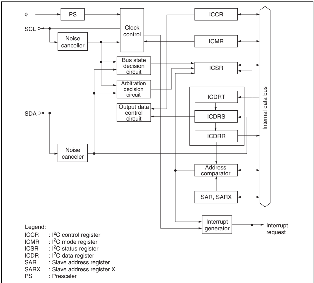
Figure 23.1 Block Diagram of I 2 C Bus Interface
