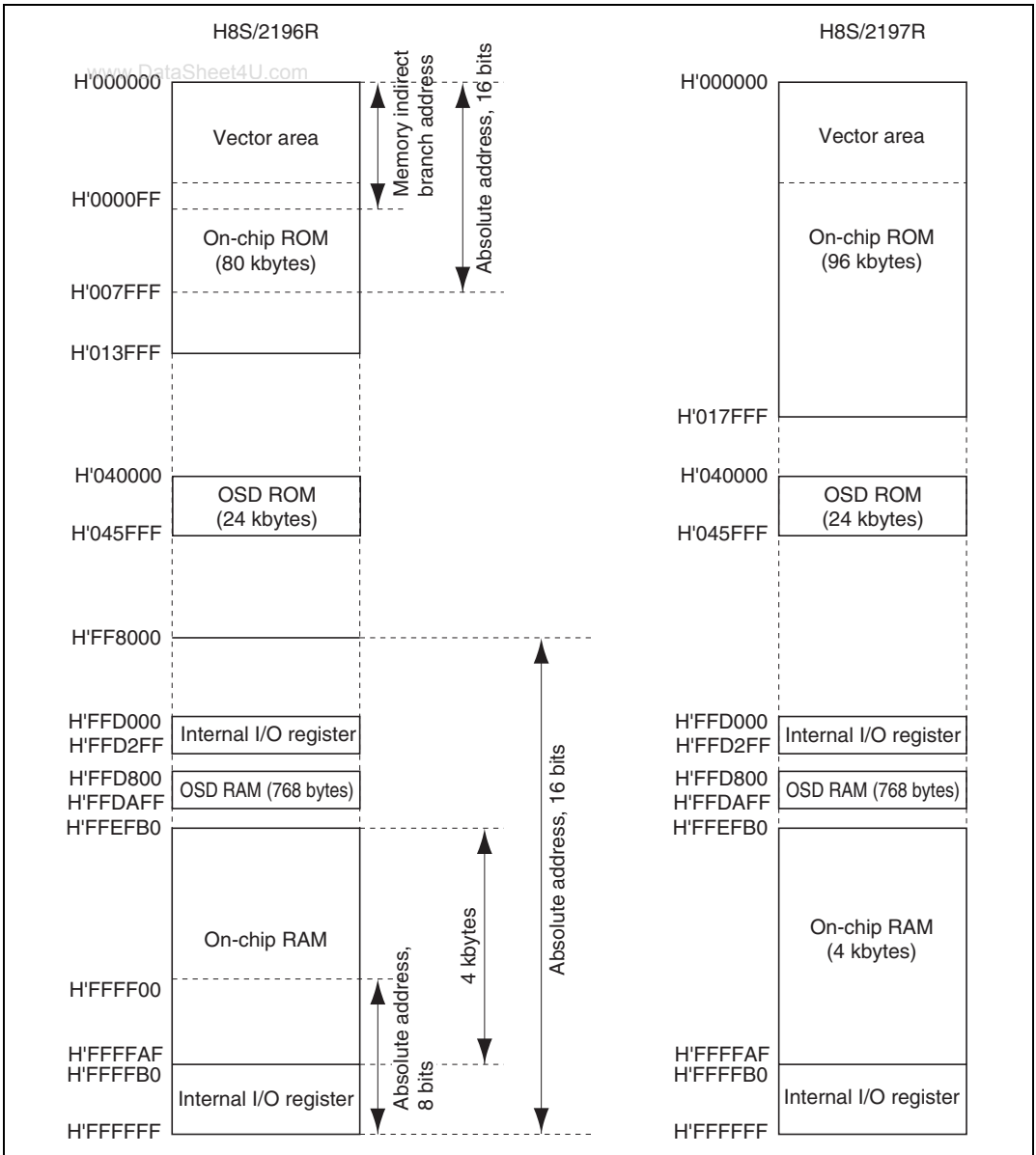
Figure 3.1 Address Map (1)
