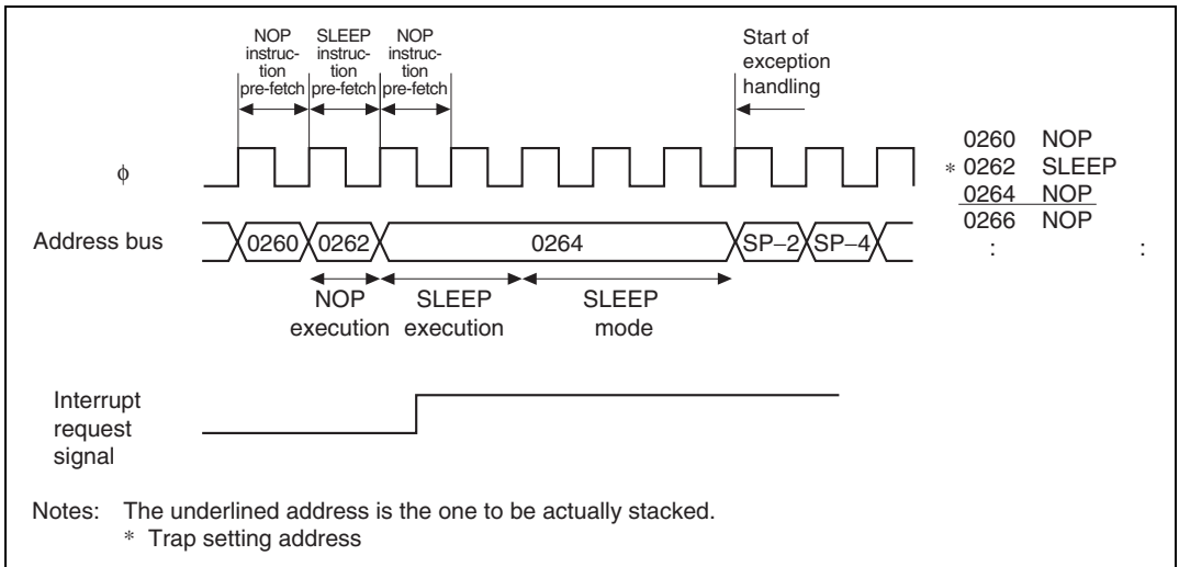
Figure 25.17 SLEEP Instruction (2)
