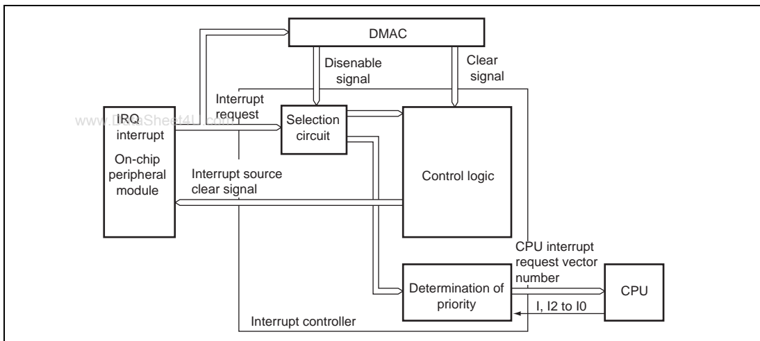
Figure 5.7 Interrupt Control for DMAC
