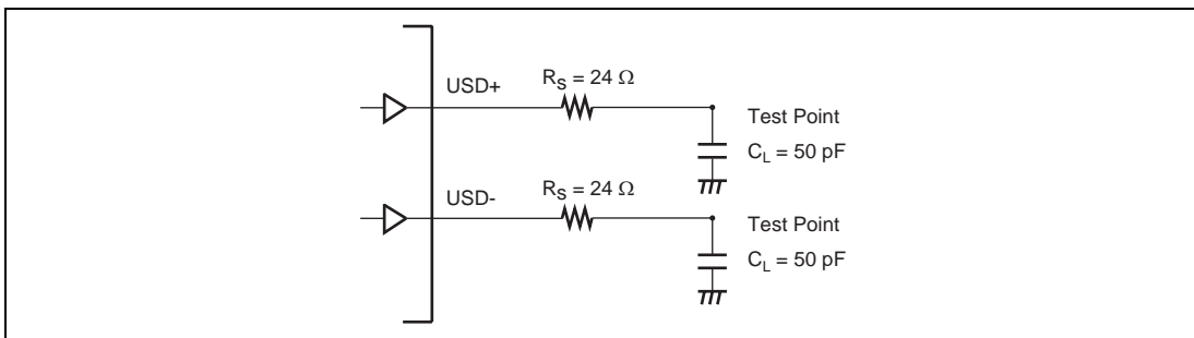
Figure 22.22 Test Load Circuit
