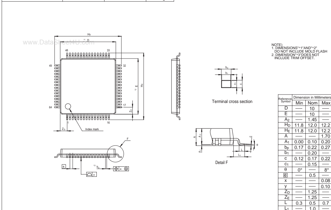
Figure C.3 FP-64E and FP-64EV Package Dimensions
