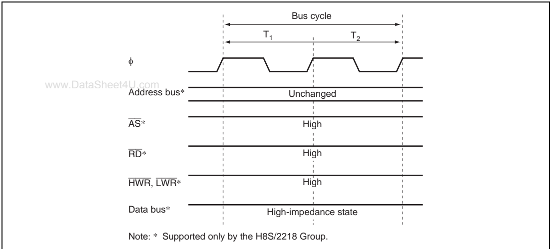
Figure 6.7 Pin States during On-Chip Peripheral Module Access
