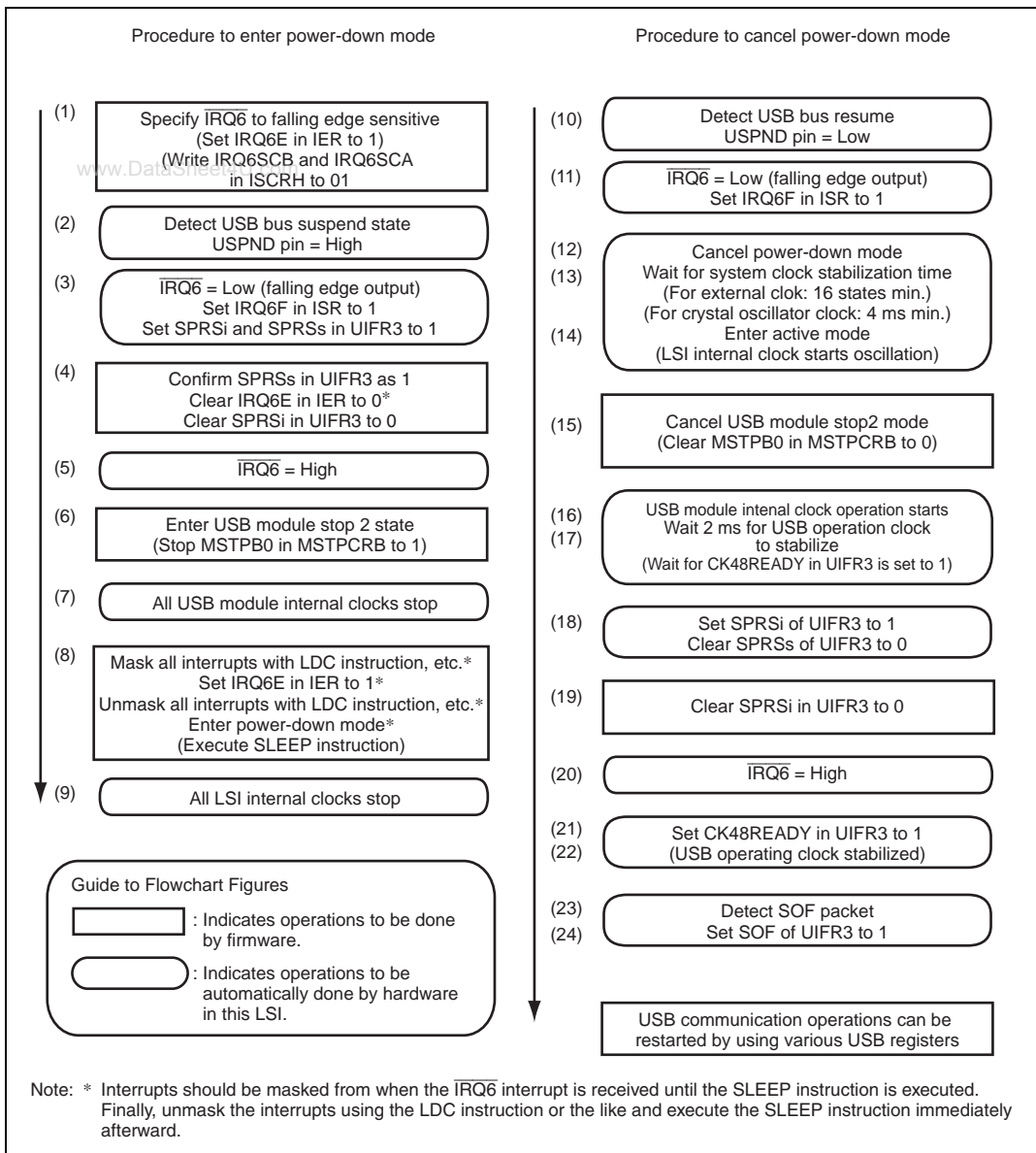
Figure 14.28 Flowchart
