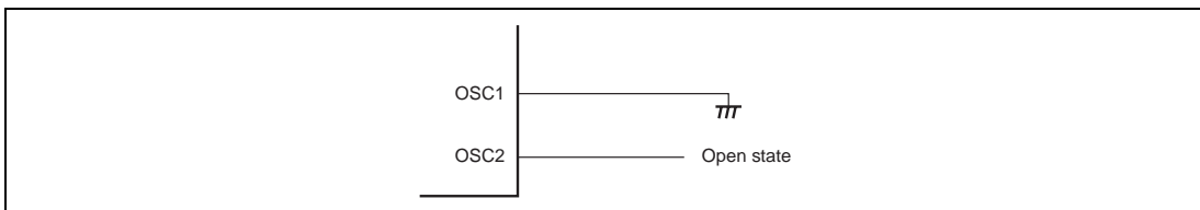
Figure 19.8 Pin Handling when Subclock Not Required
