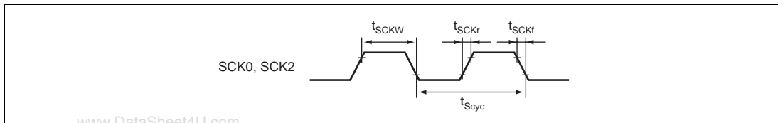
Figure 22.15 SCK Clock Input Timing
