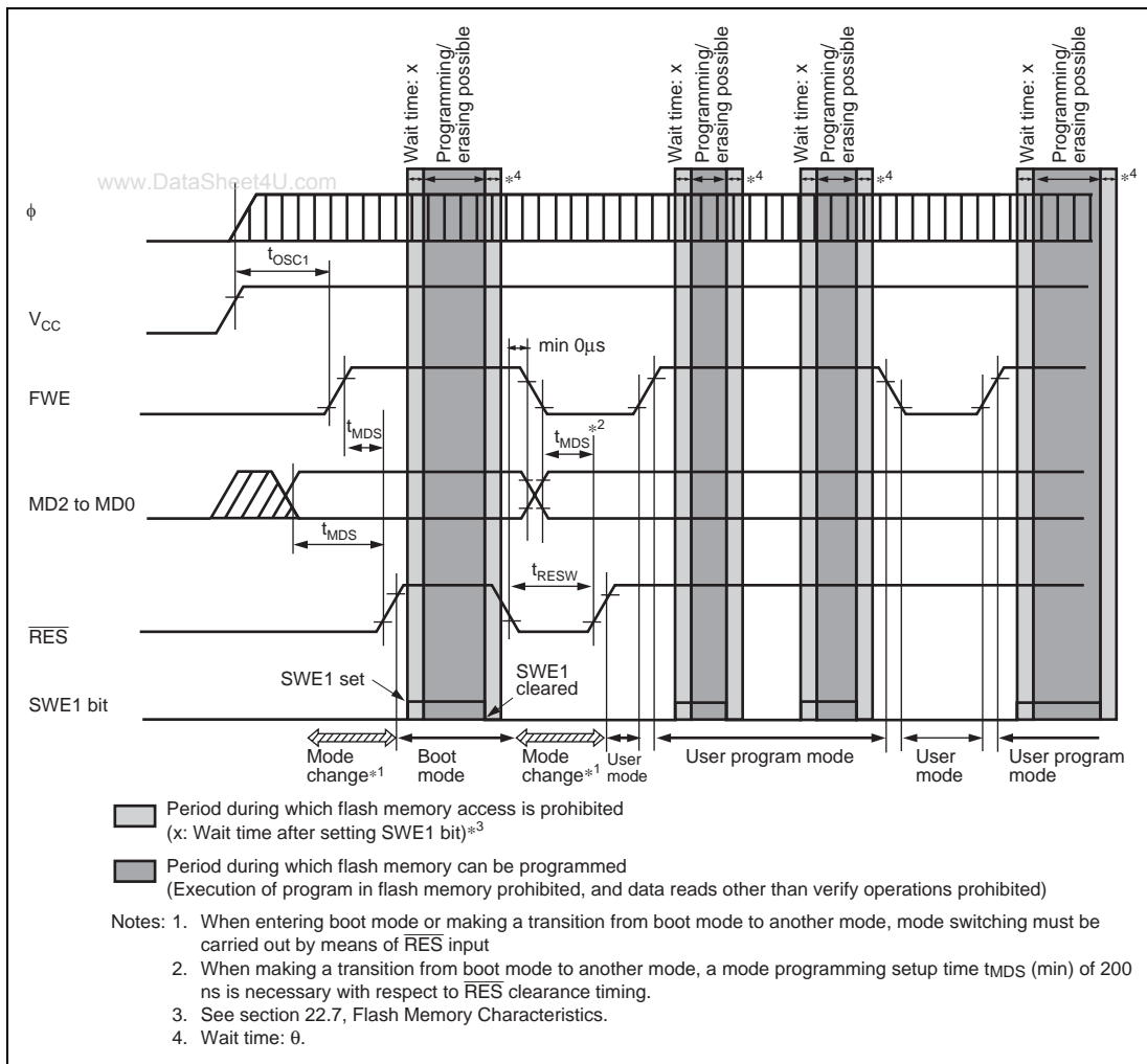
Figure 17.17 Mode Transition Timing (Example: Boot Mode → User Mode ↔ User Program Mode)
