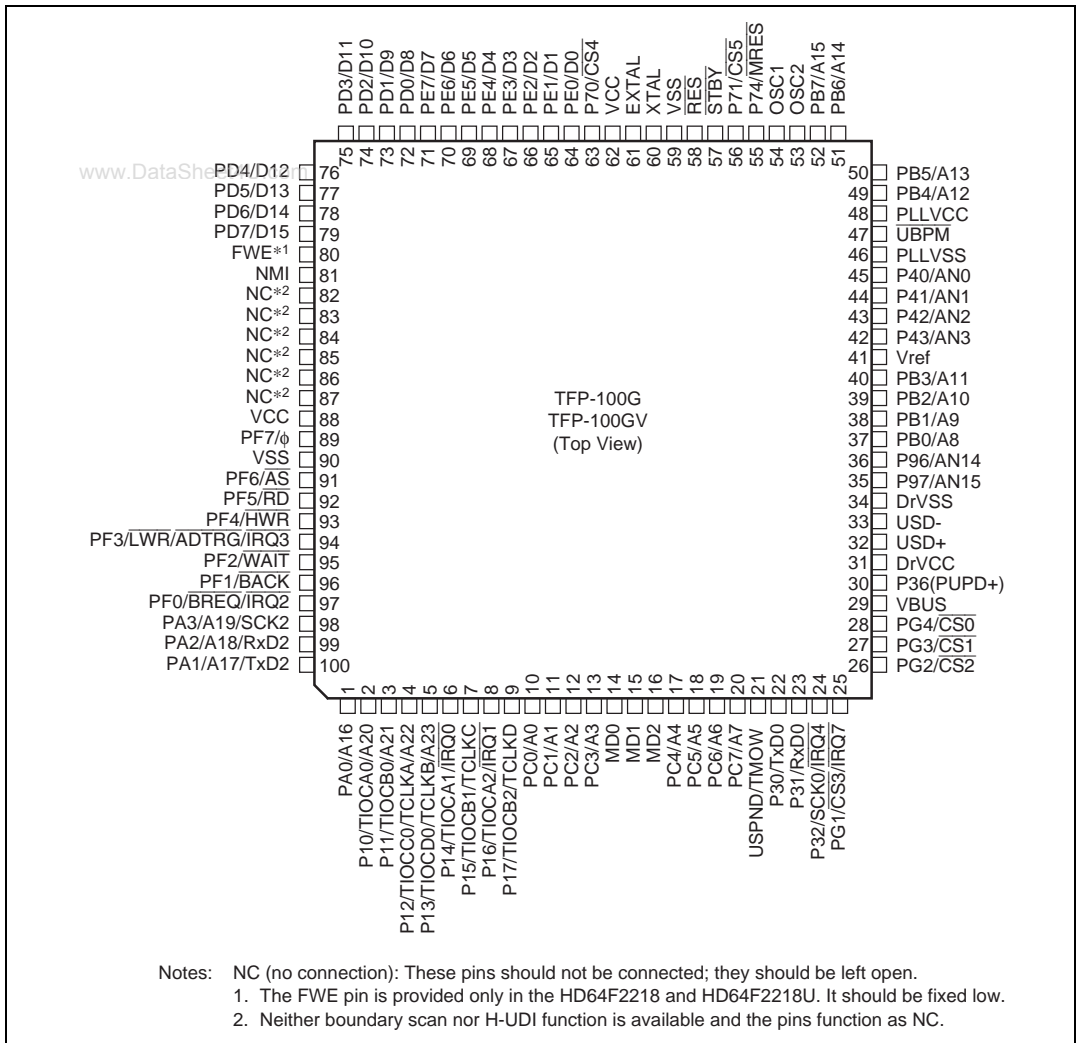
Figure 1.7 Pin Arrangements of HD6432217 (TFP-100G, TFP-100GV)
