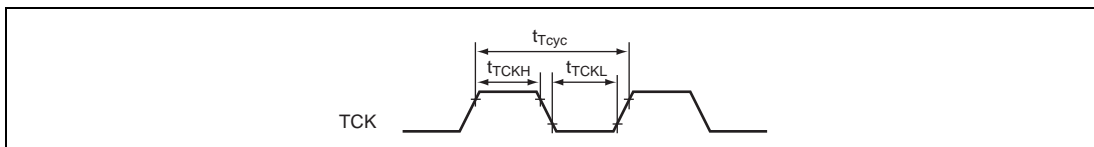
Figure 22.18 Boundary Scan TCK Input Timing
