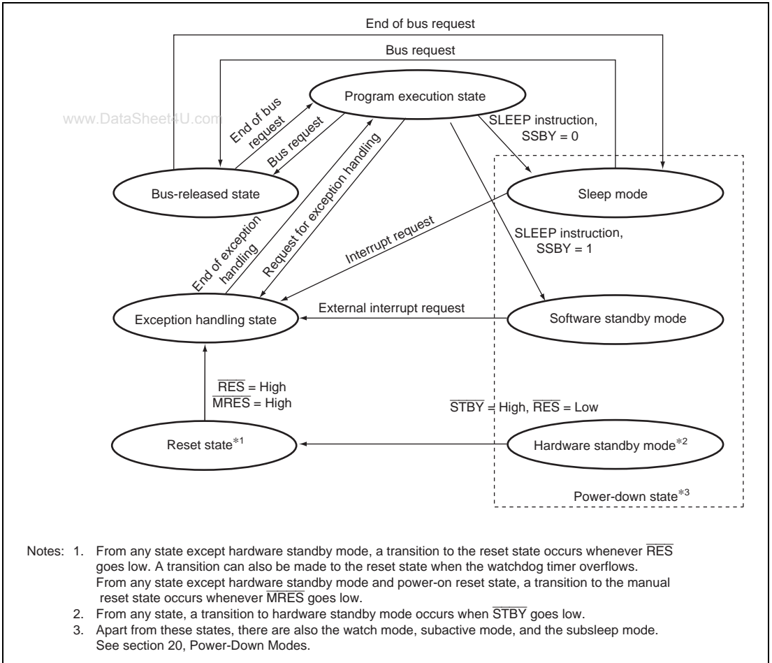
Figure 2.13 State Transitions
