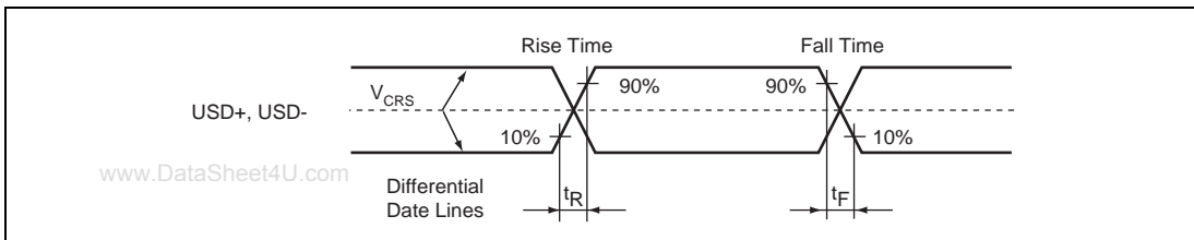
Figure 22.21 Data Signal Timing
