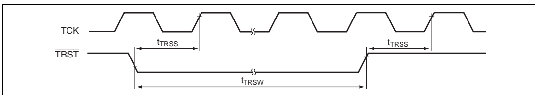
Figure 22.19 Boundary Scan TRST Input Timing (At Reset Hold)
