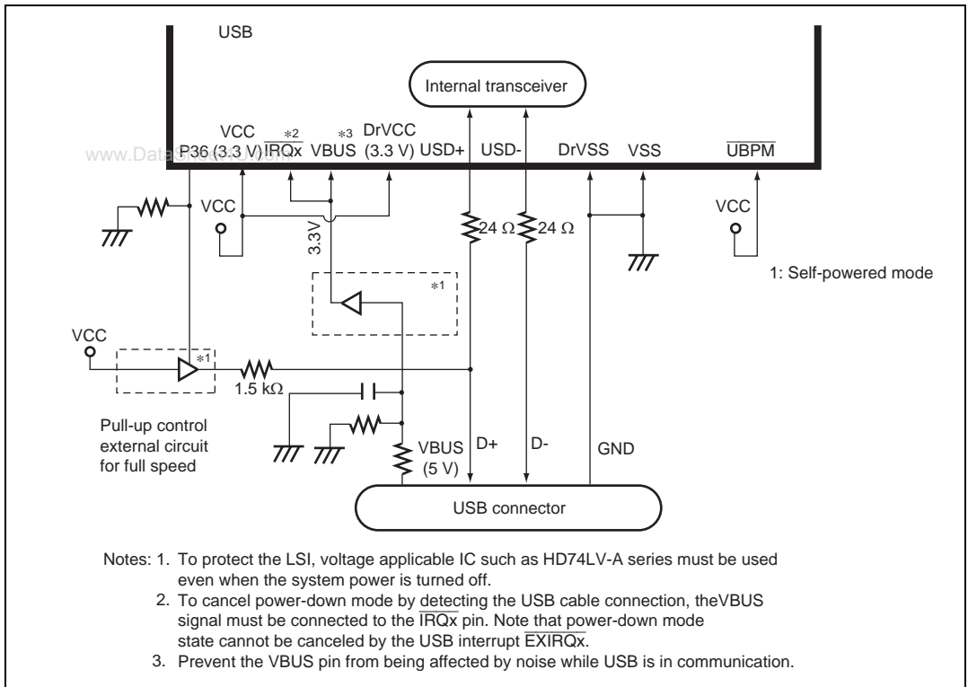
Figure 14.27 USB External Circuit in Self-Powered Mode
