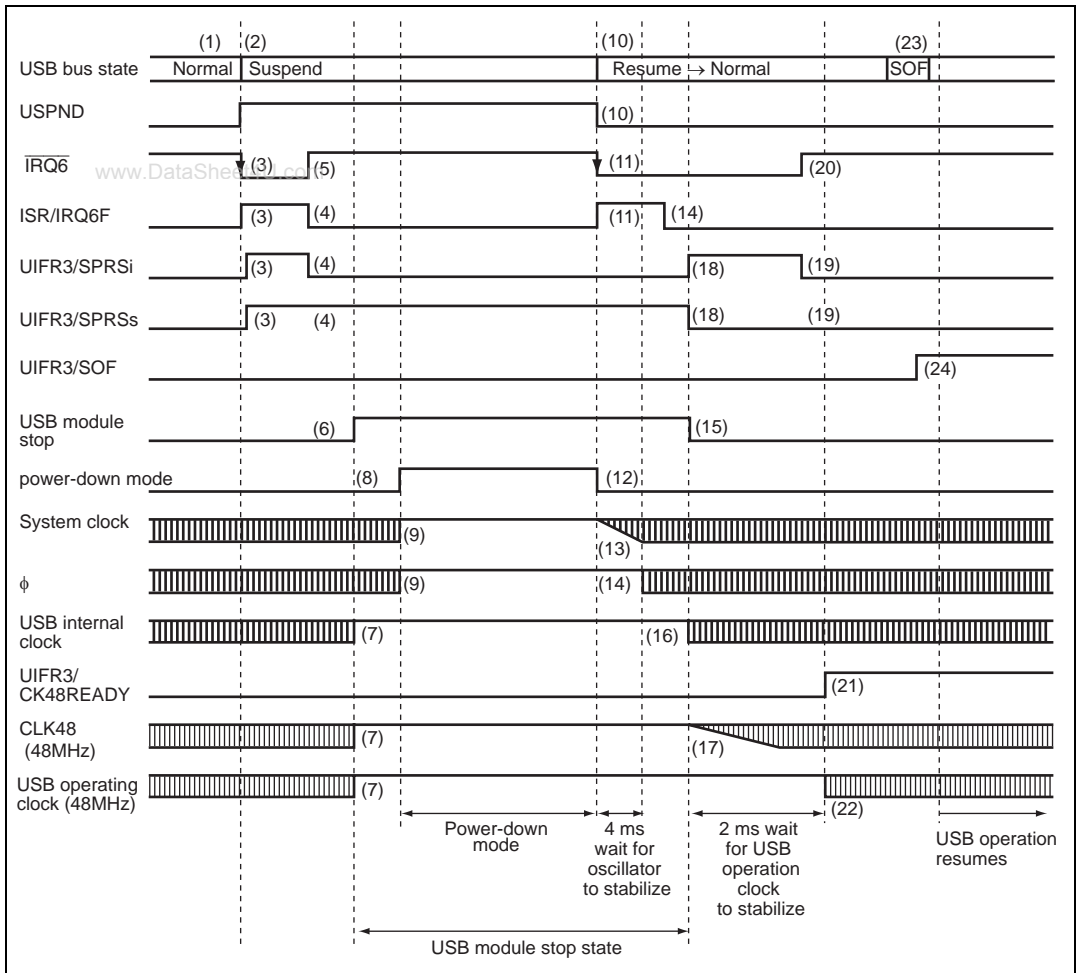
Figure 14.29 Timing Chart
