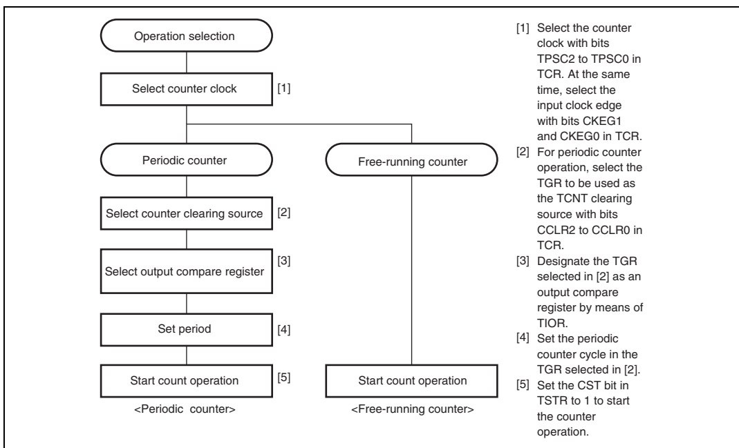
Figure 10.6 Example of Counter Operation Setting Procedure
