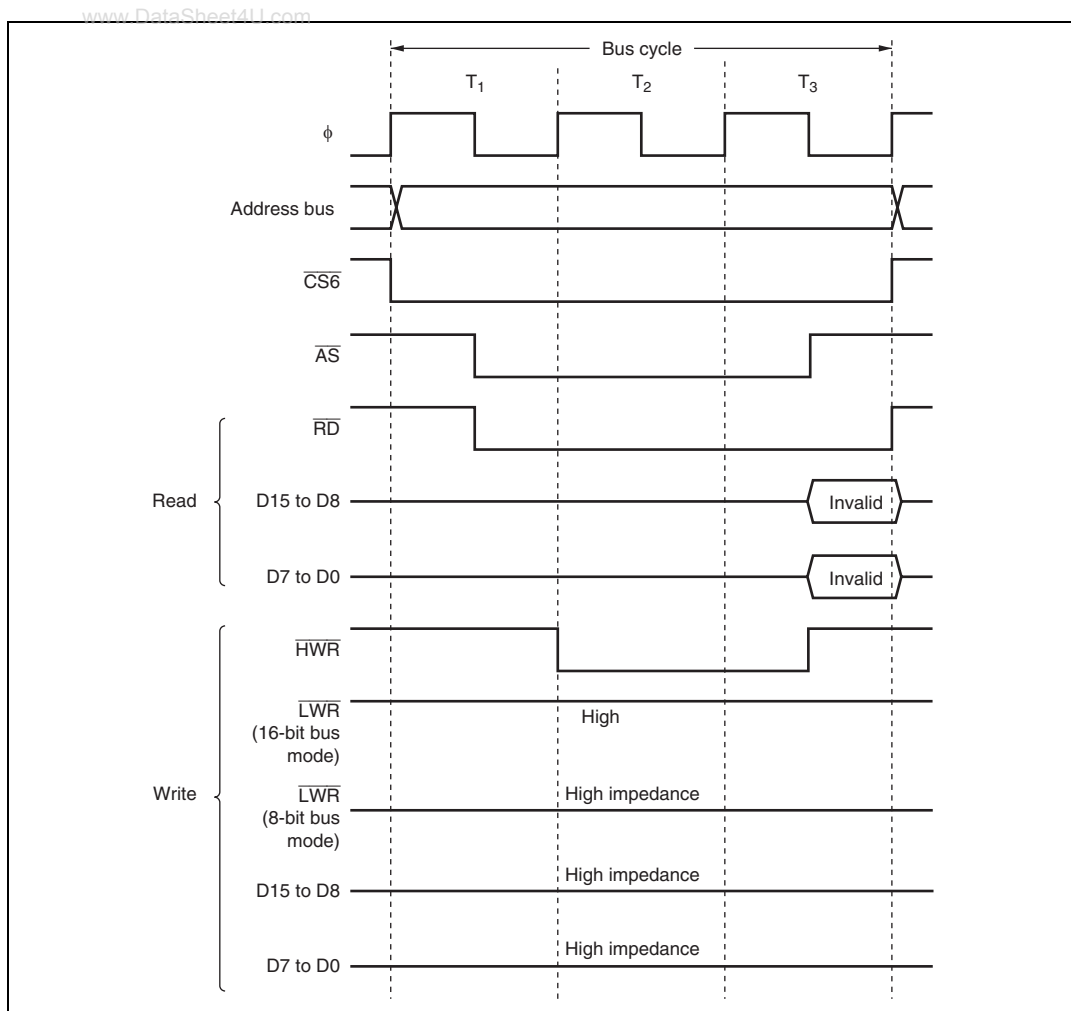
Figure 6.12 Bus Timing for Area 6
