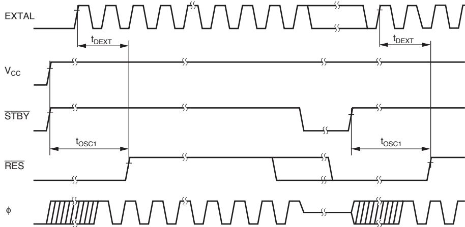
Figure 24.4 Oscillation Stabilization Timing
