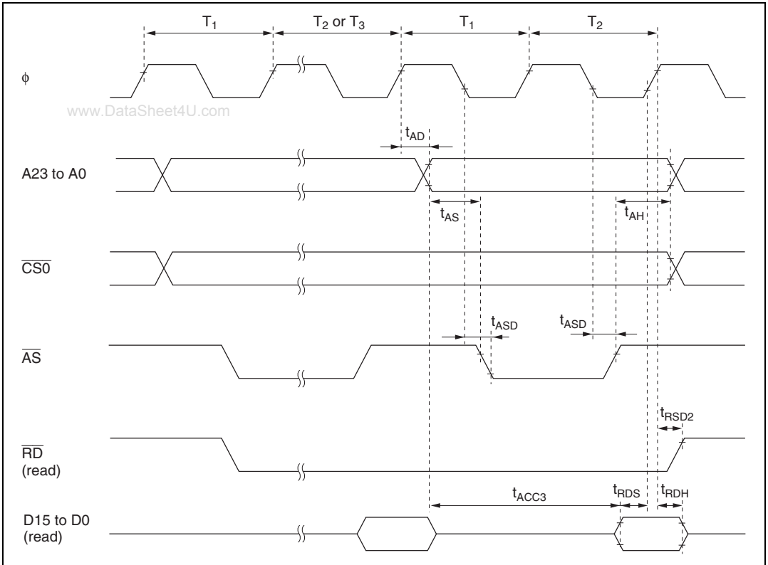
Figure 25.10 Burst ROM Access Timing (Two-State Access)
