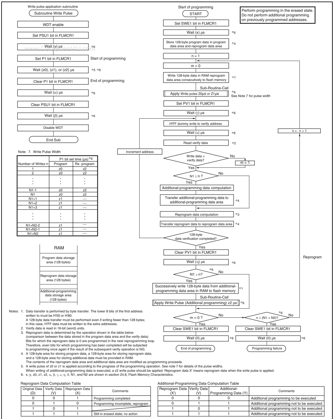
Figure 19.11 Program/Program-Verify Flowchart
