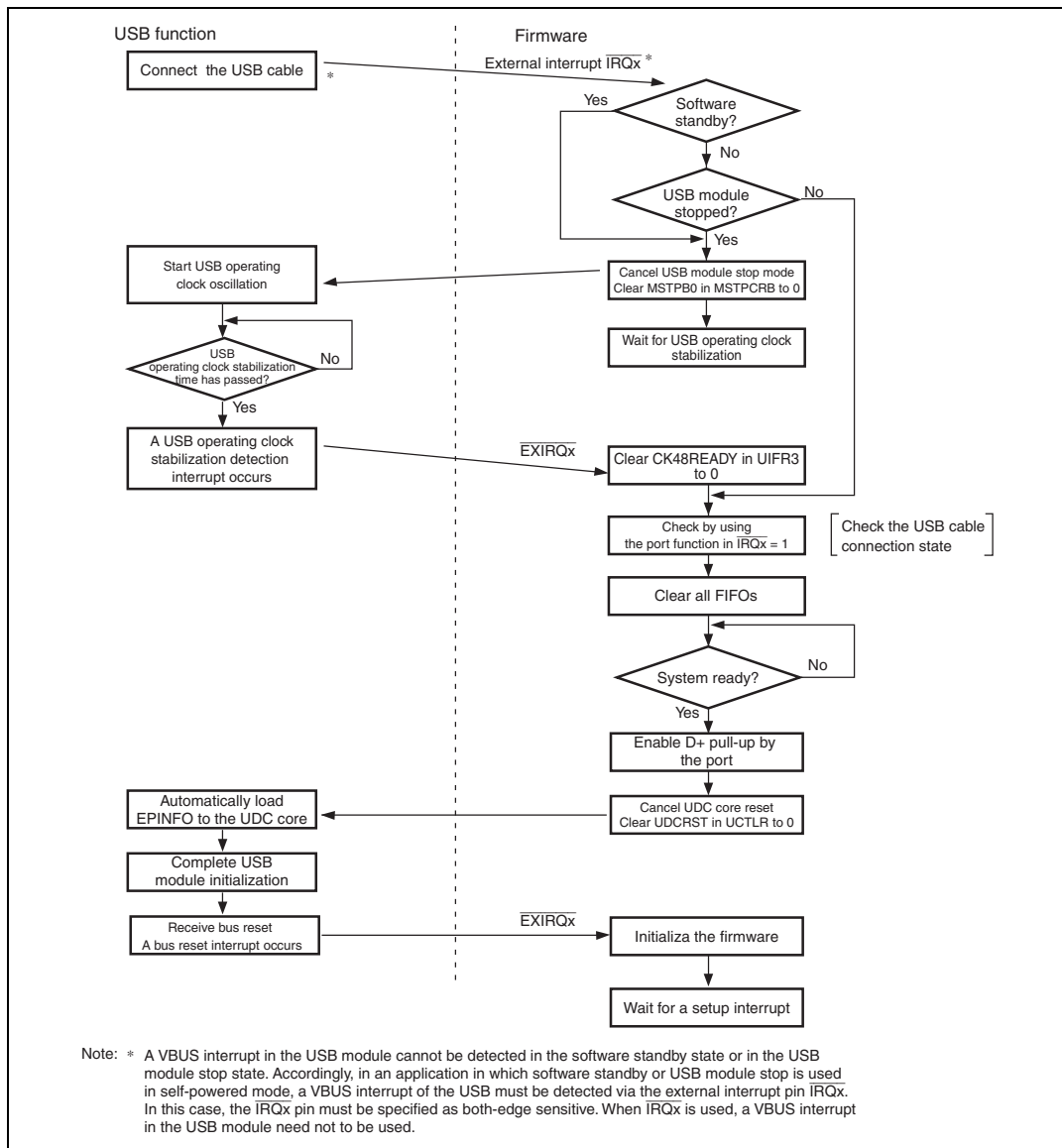
Figure 15.5 USB Cable Connection (When USB Module Stop or Software Standby Is Used)
