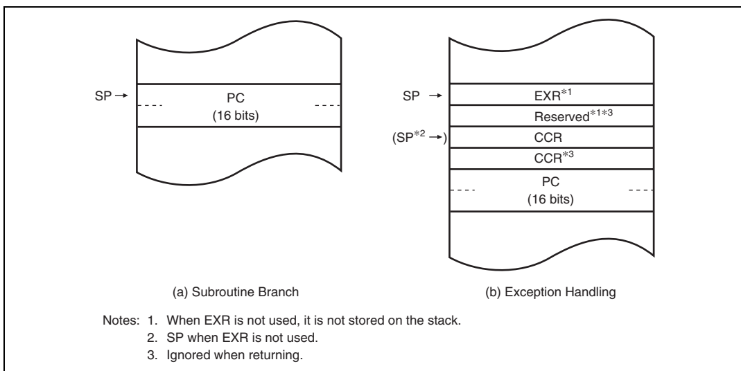
Figure 2.2 Stack Structure in Normal Mode
