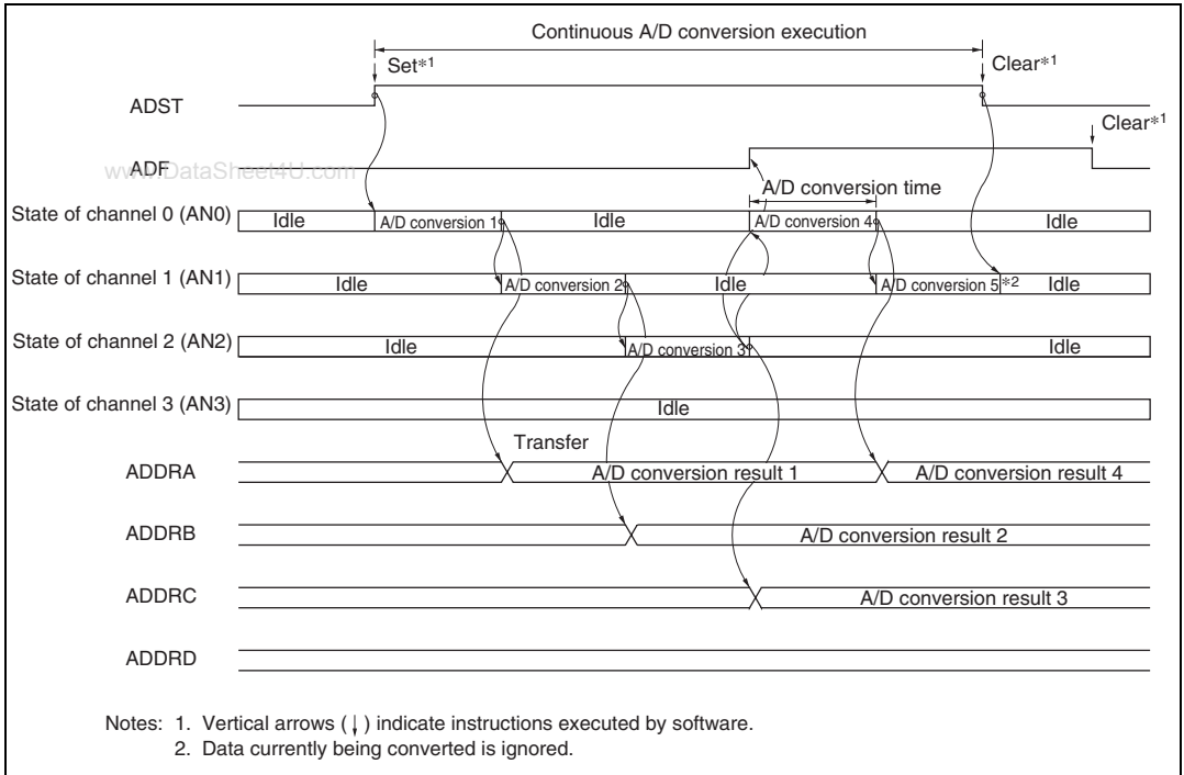
Figure 16.4 A/D Conversion Timing (Scan Mode, Channels AN0 to AN3 Selected)
