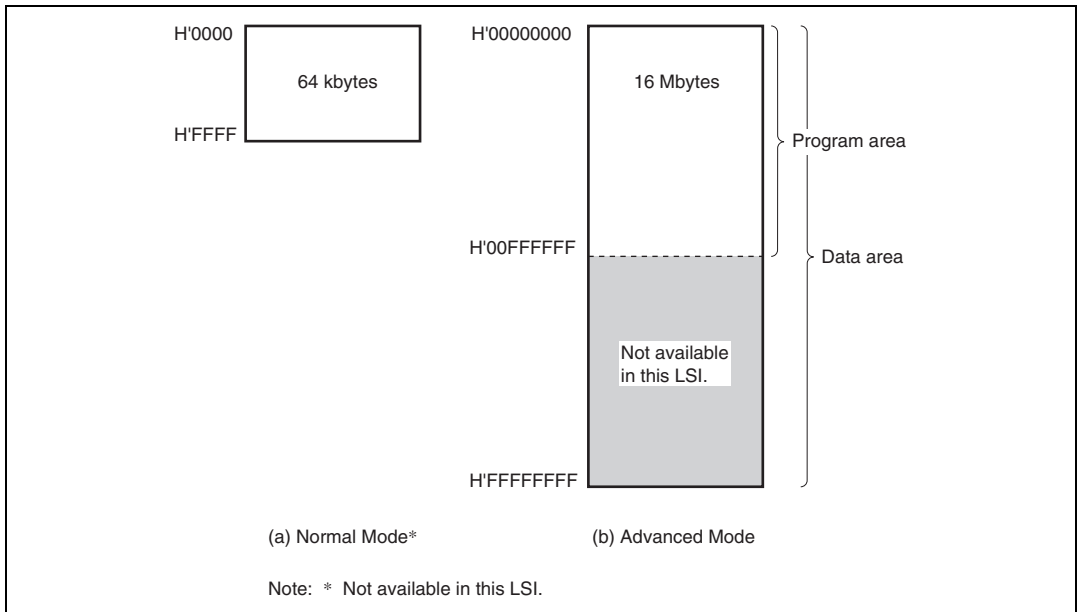
Figure 2.5 Memory Map
