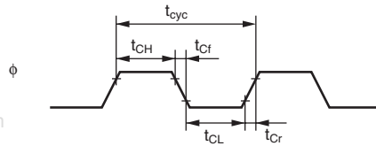
Figure 24.3 System Clock Timing
