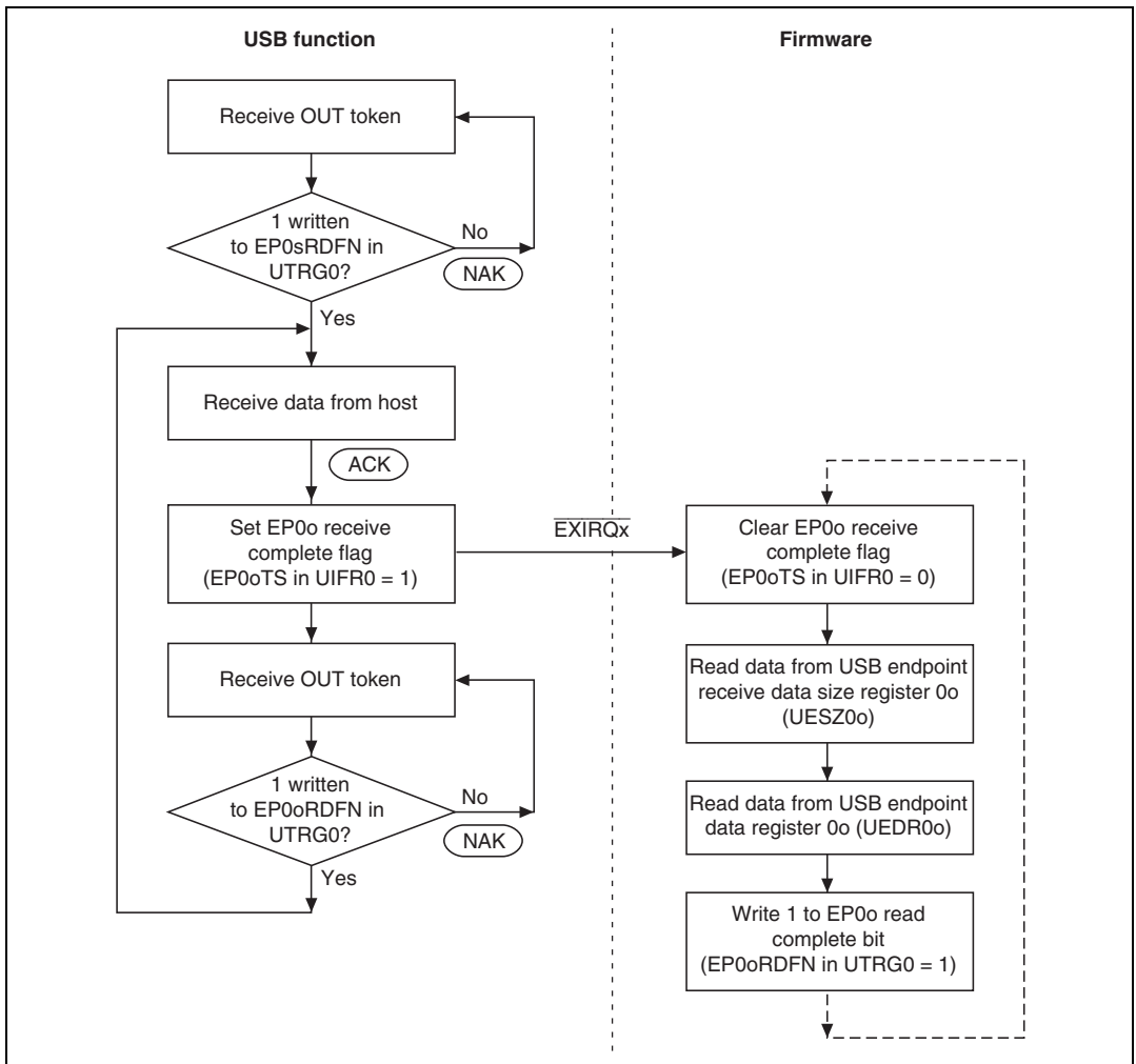
Figure 15.15 Data Stage Operation (Control-Out)
