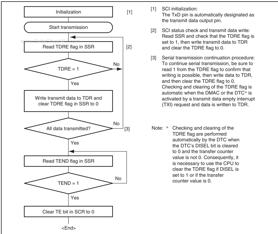
Figure 13.21 Sample Serial Transmission Data Flowchart
