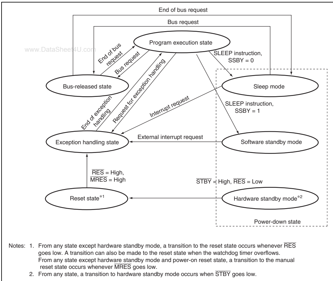
Figure 2.13 State Transitions
