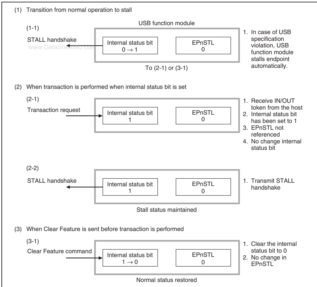
Figure 15.24 Automatic Stall by USB Function Module
