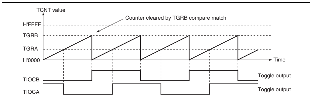
Figure 10.11 Example of Toggle Output Operation
