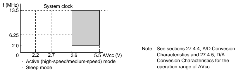
Figure 27.3 Power Supply Voltage and Operating Ranges (H8S/2238B and H8S/2236B)
