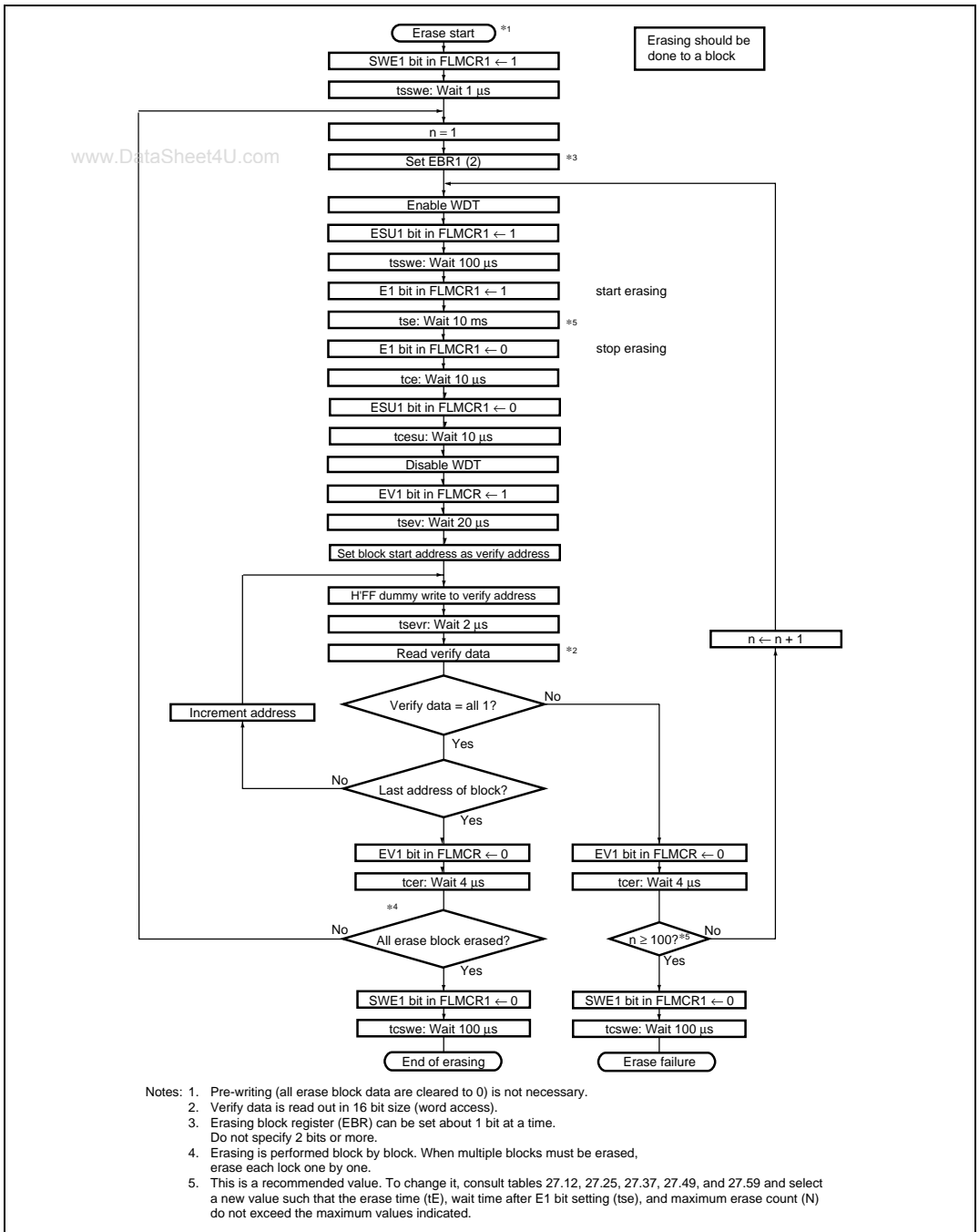
Figure 20.12 Erase/Erase-Verify Flowchart
