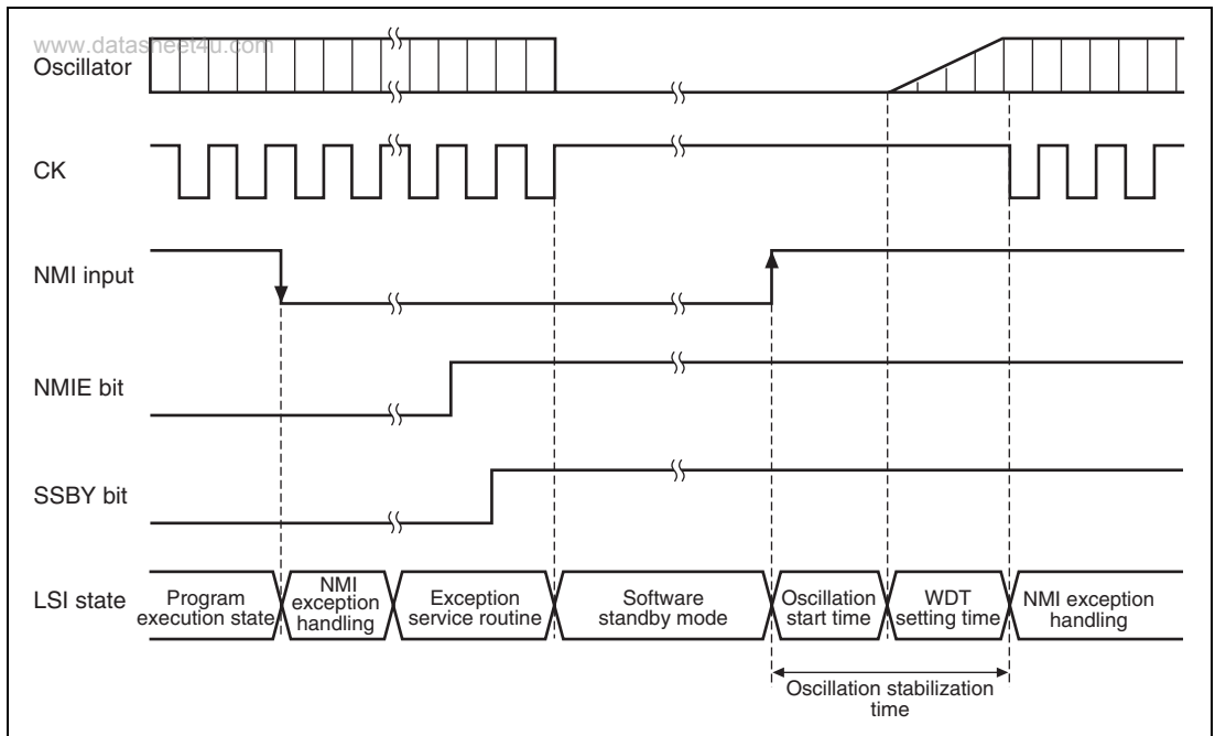
Figure 17.2 NMI Timing in Software Standby Mode
