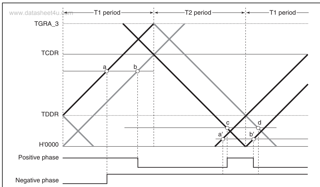
Figure 8.42 Example of Complementary PWM Mode Waveform Output (3)
