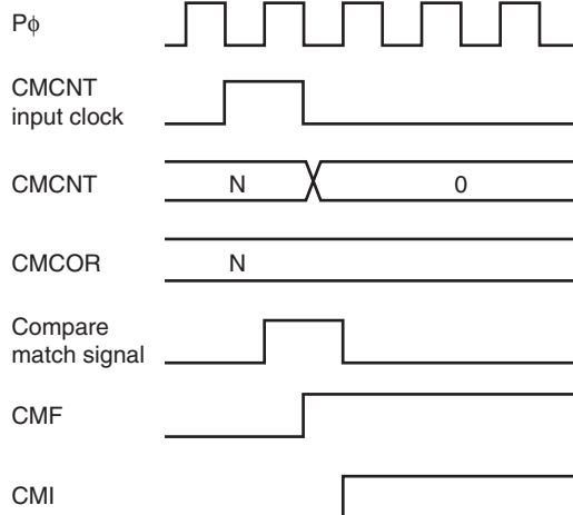
Figure 12.4 CMF Set Timing
