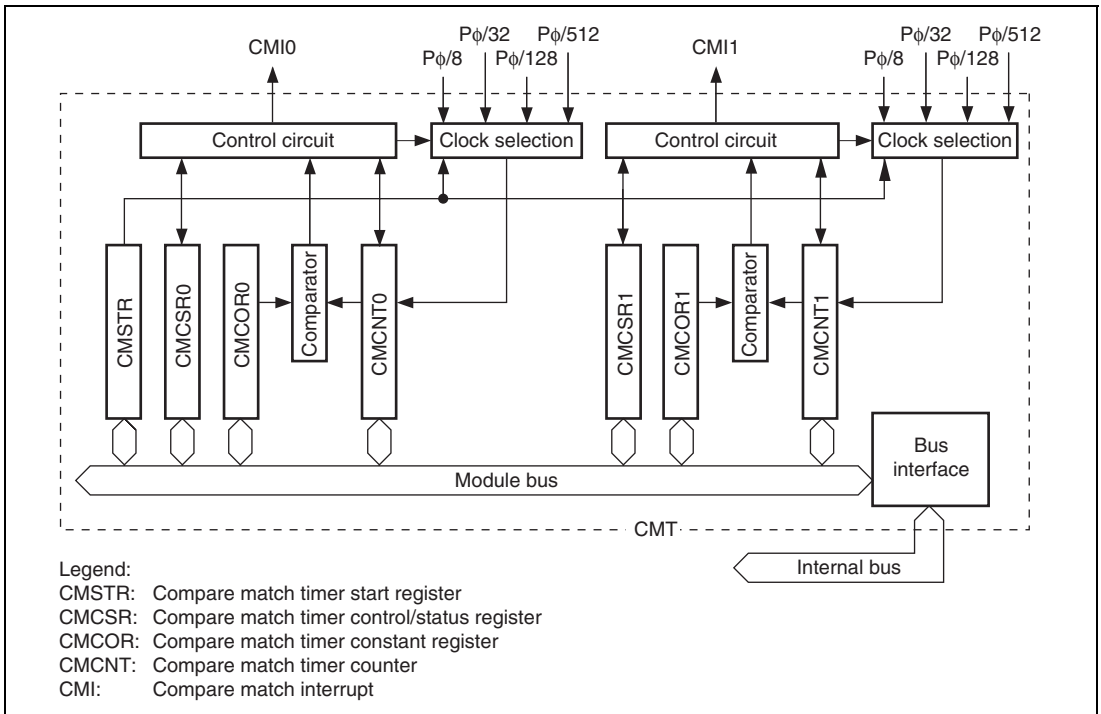
Figure 12.1 CMT Block Diagram
