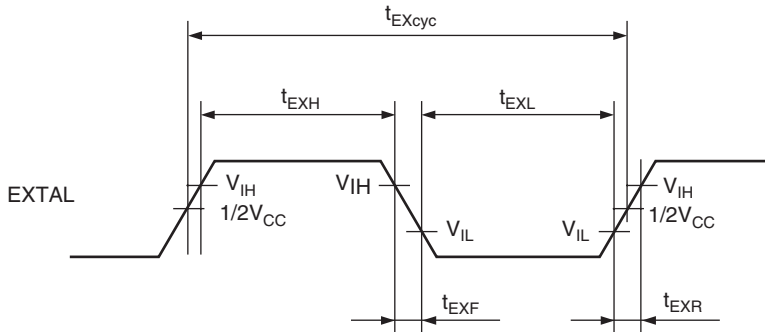
Figure 19.3 EXTAL Clock Input Timing
