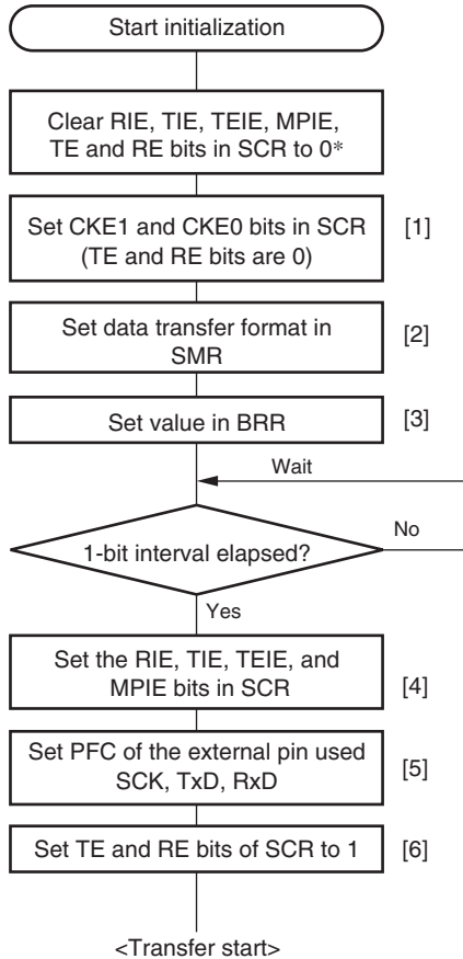
Figure 10.15 Sample SCI Initialization Flowchart
