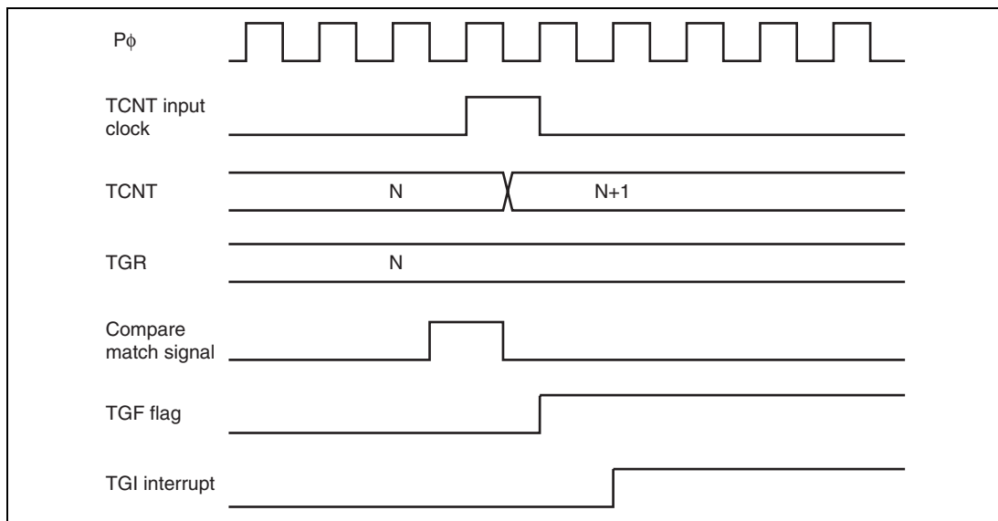
Figure 8.64 TGI Interrupt Timing (Compare Match)
