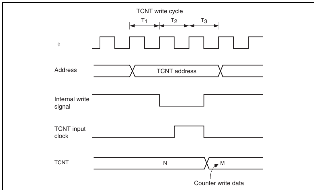
Figure 9.8 Contention between TCNT Write and Increment
