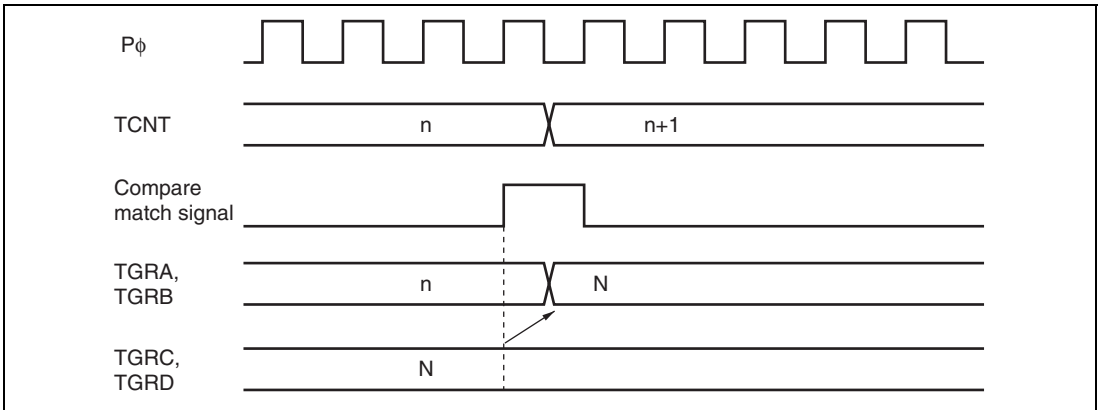
Figure 8.62 Buffer Operation Timing (Compare Match)
