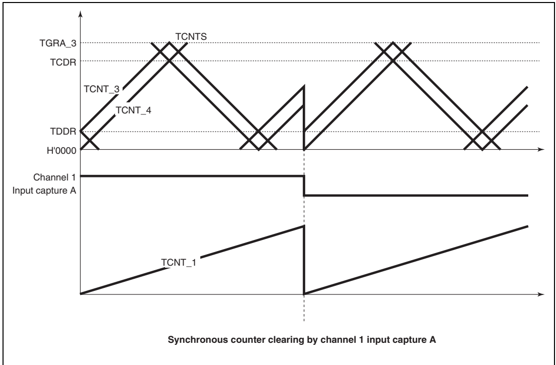
Figure 8.49 Counter Clearing Synchronized with Another Channel
