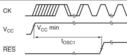
Figure 19.4 Oscillation Settling Time
