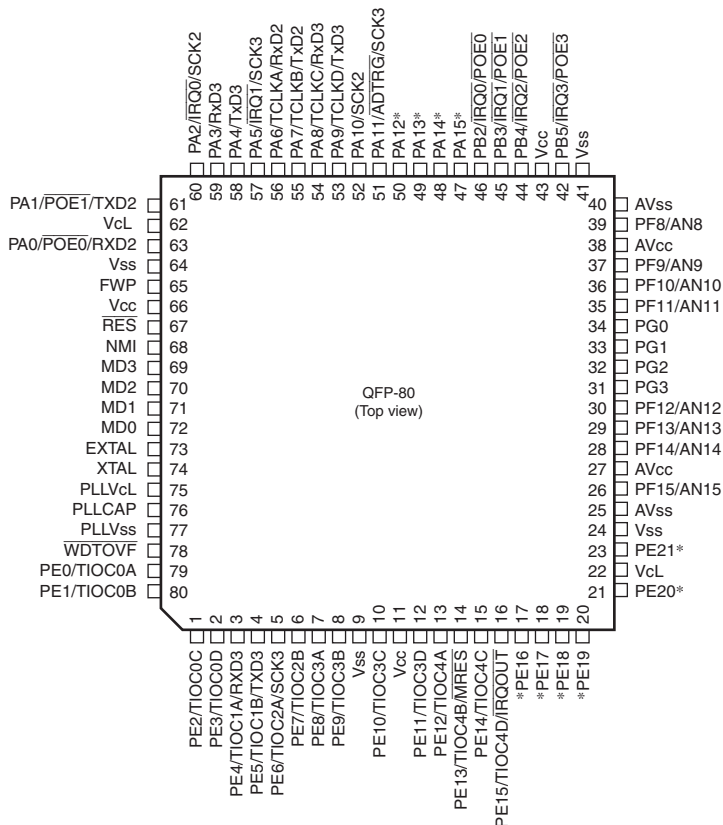
Figure 1.2 SH7101 Pin Arrangement
