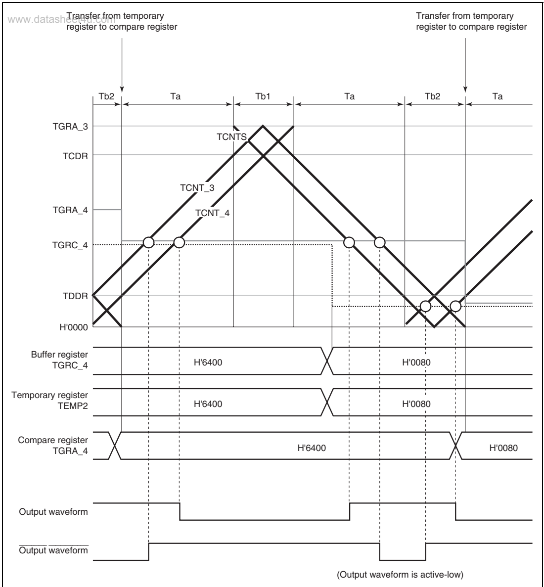
Figure 8.35 Example of Complementary PWM Mode Operation
