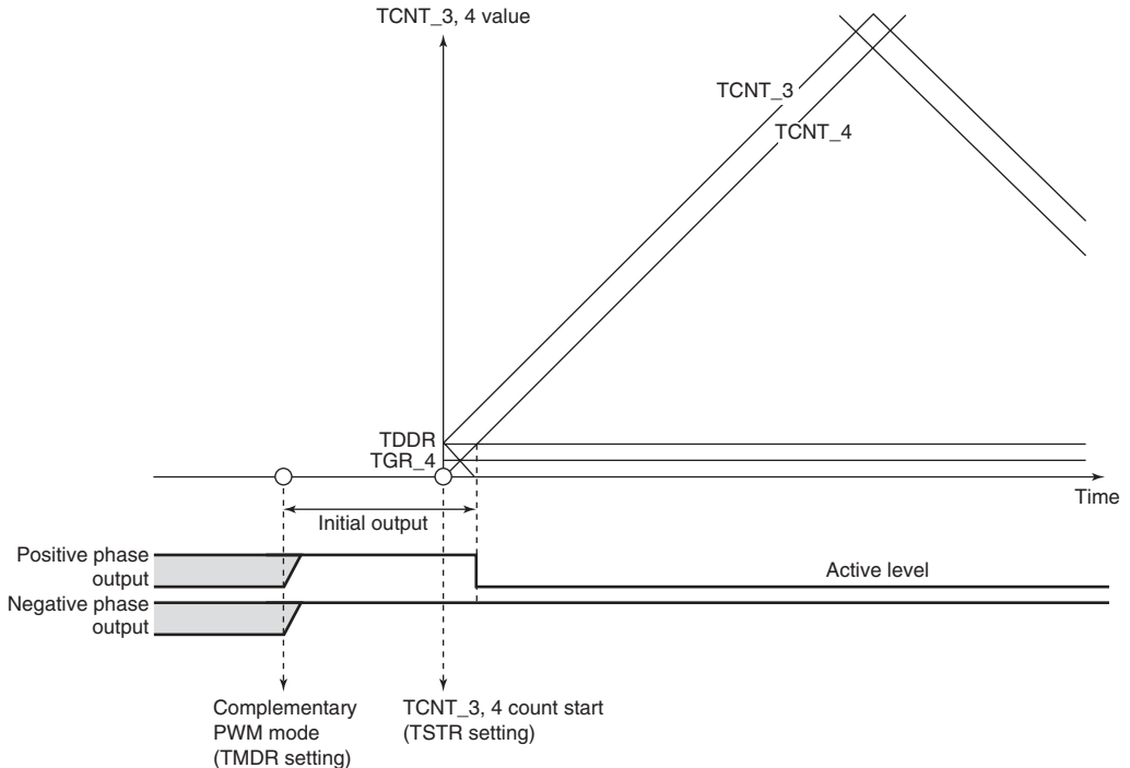
Figure 8.39 Example of Initial Output in Complementary PWM Mode (2)
