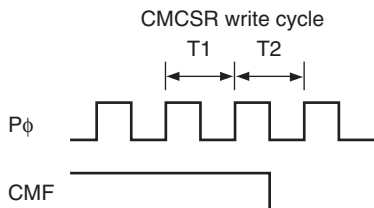
Figure 12.5 Timing of CMF Clear by CPU
