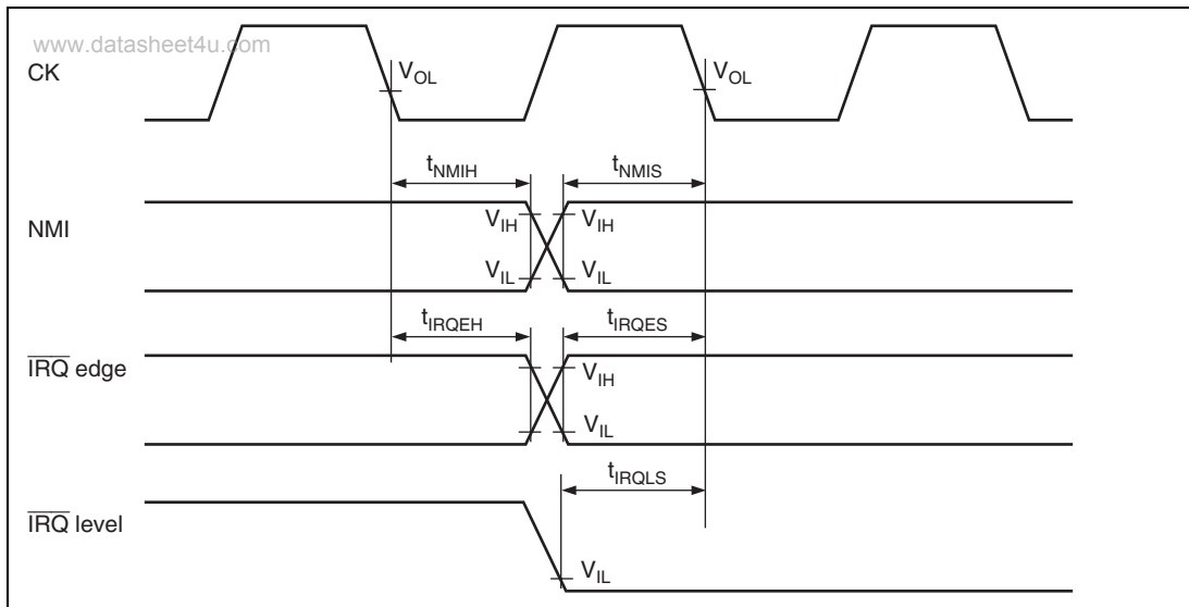
Figure 19.7 Interrupt Signal Input Timing
