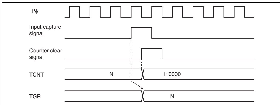
Figure 8.61 Counter Clear Timing (Input Capture)
