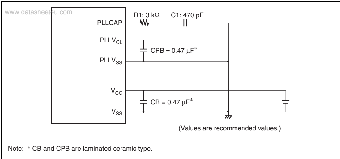
Figure 4.6 Recommended External Circuitry around PLL
