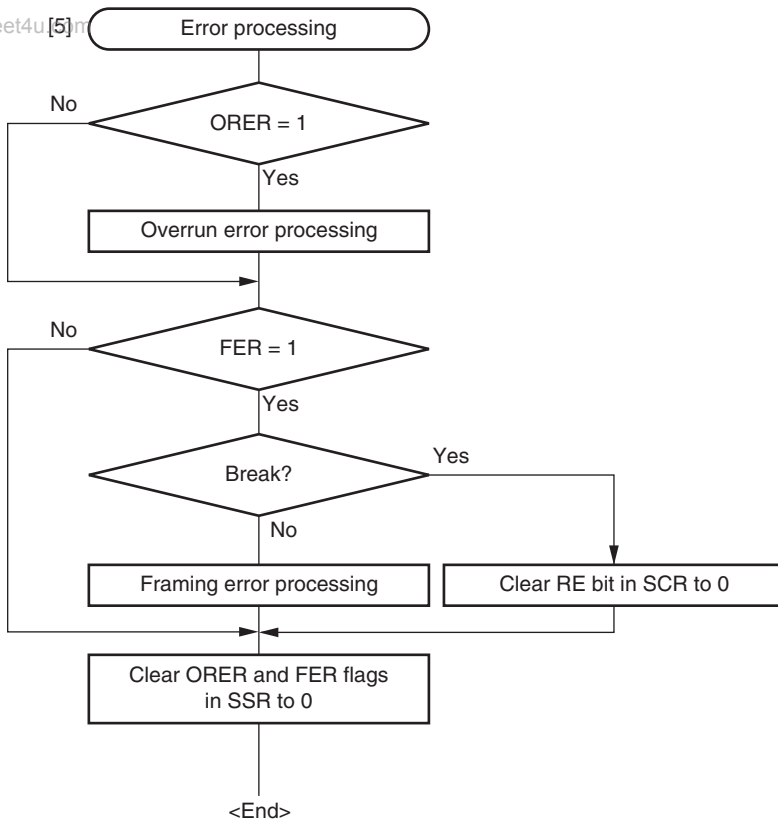
Figure 10.13 Sample Multiprocessor Serial Reception Flowchart (2)
