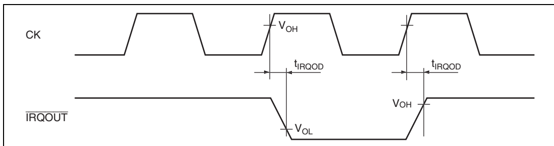
Figure 19.8 Interrupt Signal Output Timing
