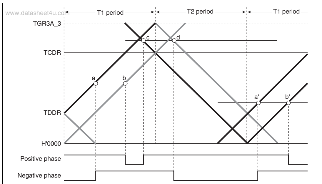
Figure 8.40 Example of Complementary PWM Mode Waveform Output (1)
