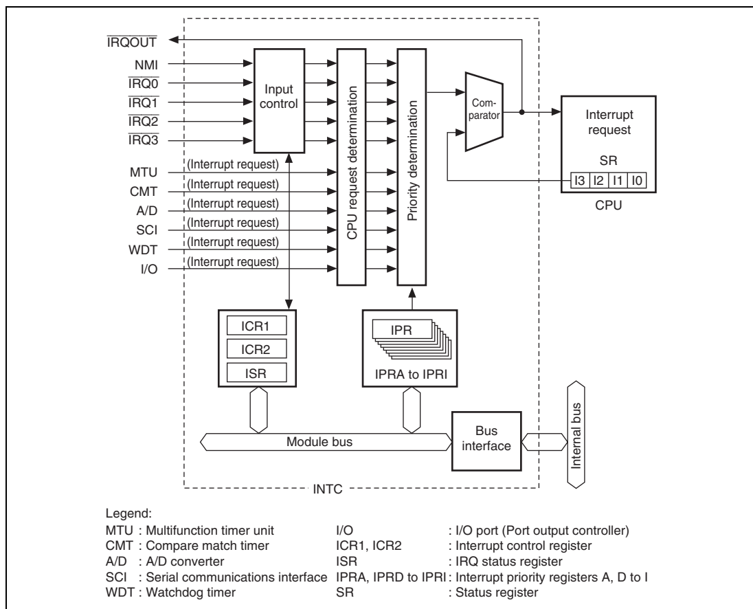
Figure 6.1 INTC Block Diagram
