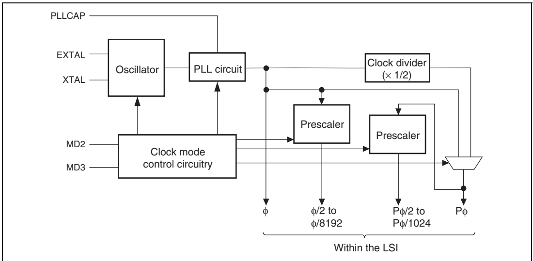
Figure 4.1 Block Diagram of Clock Pulse Generator
