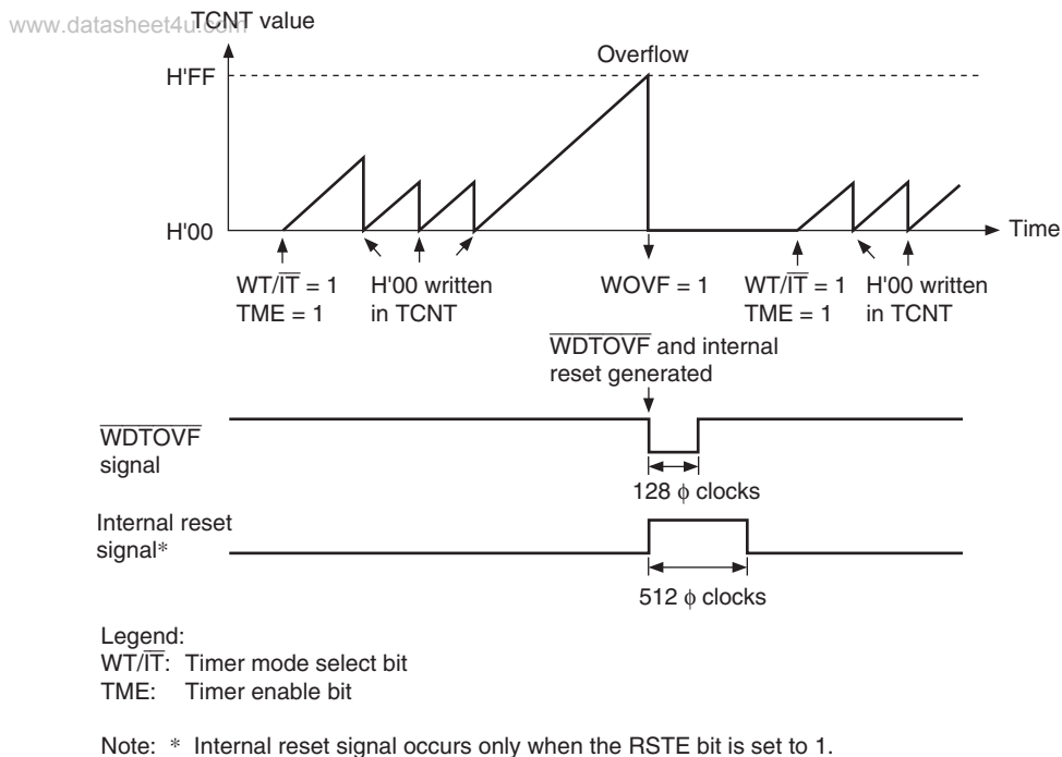
Figure 9.2 Operation in Watchdog Timer Mode
