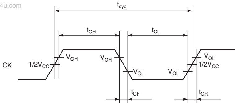
Figure 19.2 System Clock Timing
