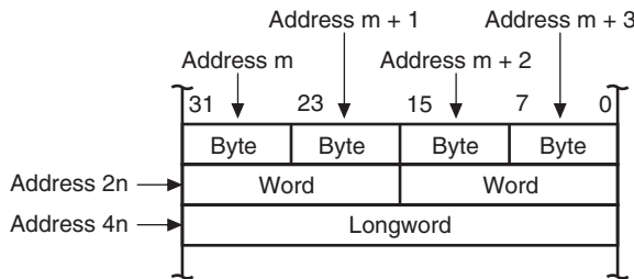
Figure 2.3 Data Formats in Memory
