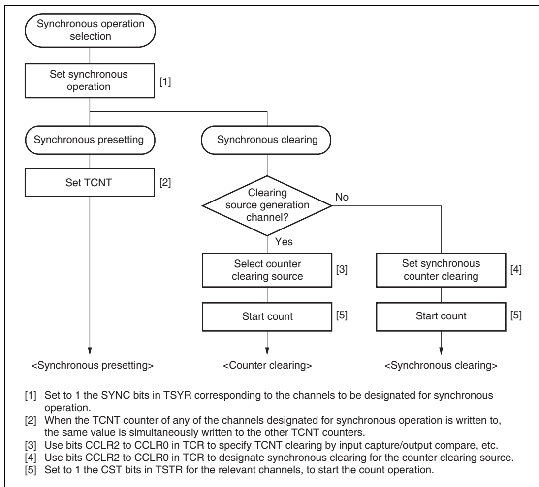
Figure 8.11 Example of Synchronous Operation Setting Procedure
