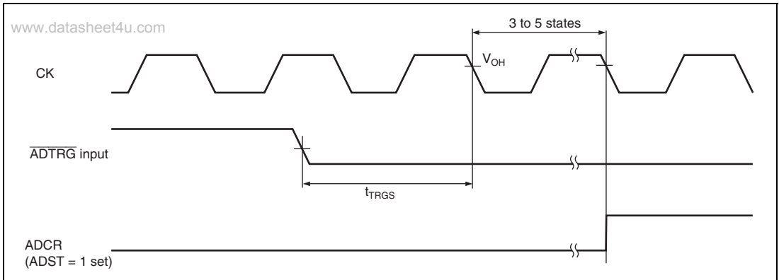
Figure 19.16 External Trigger Input Timing
