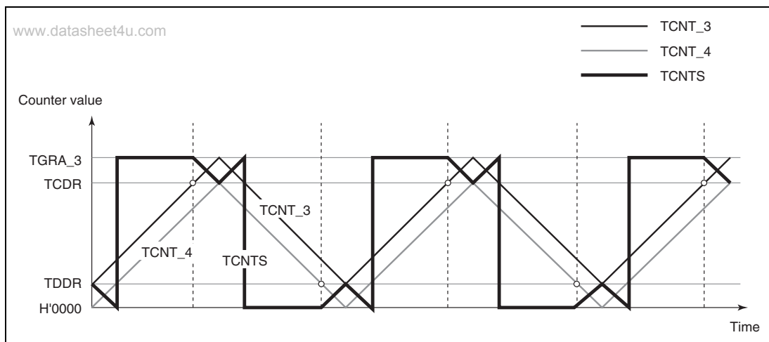
Figure 8.34 Complementary PWM Mode Counter Operation
