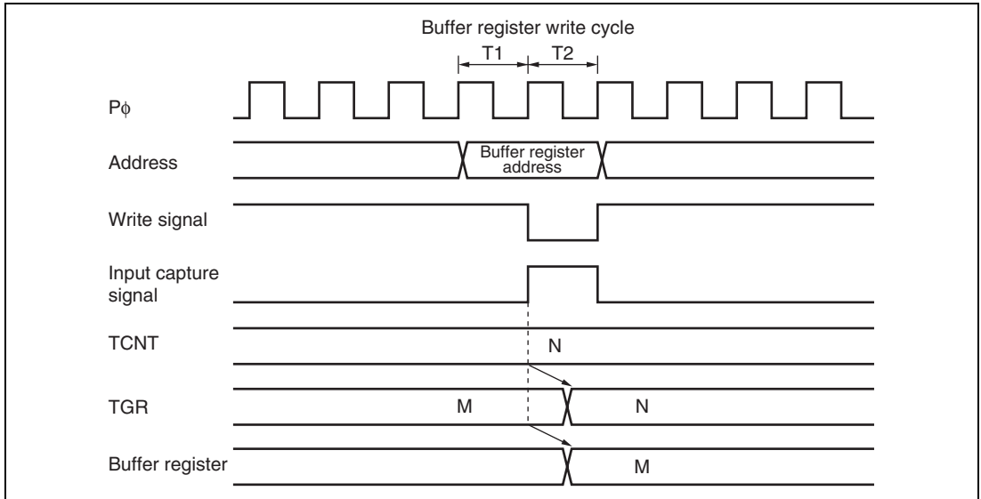
Figure 8.77 Contention between Buffer Register Write and Input Capture
