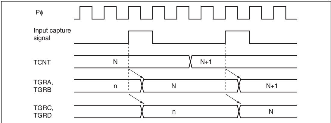
Figure 8.63 Buffer Operation Timing (Input Capture)
