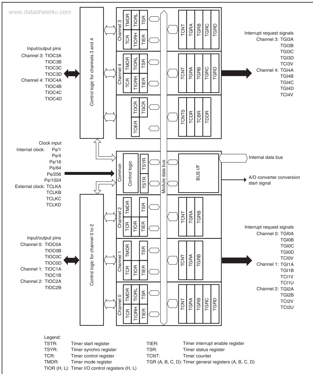
Figure 8.1 Block Diagram of MTU
