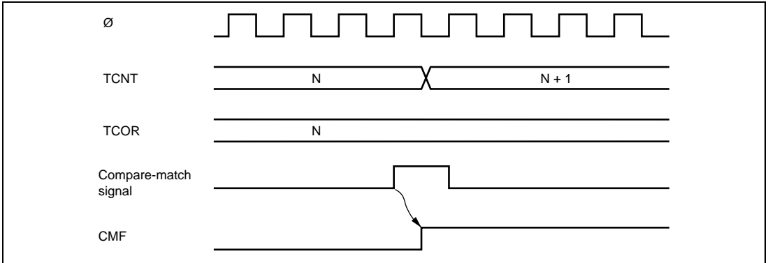
Figure 12.6 Timing of CMF Setting at Compare-Match
