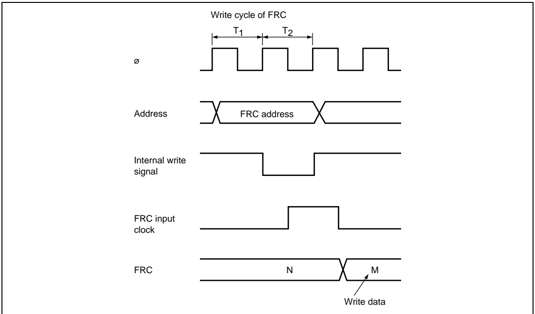
Figure 11.18 FRC Write-Increment Conflict
