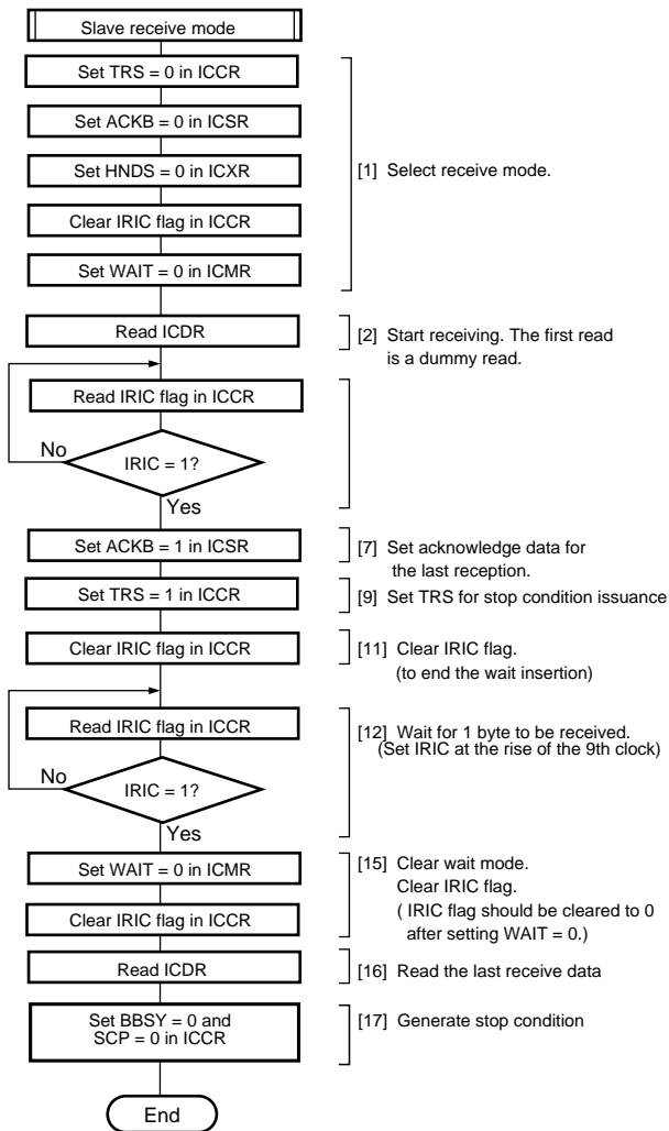
Figure 16.15 Sample Flowchart for Operations in Master Receive Mode (receiving a single byte) (WAIT = 1)
