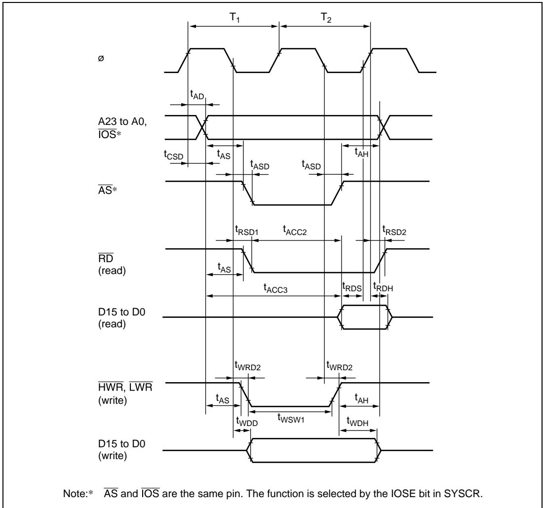
Figure 28.11 Basic Bus Timing (Two-State Access)
