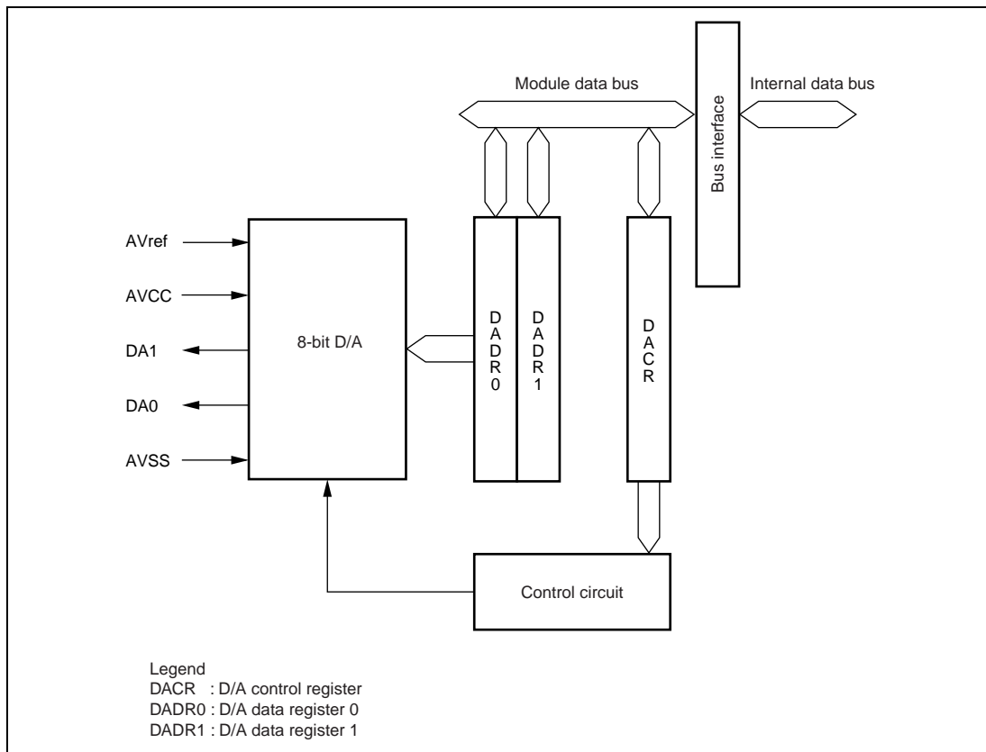
Figure 20.1 Block Diagram of D/A Converter
