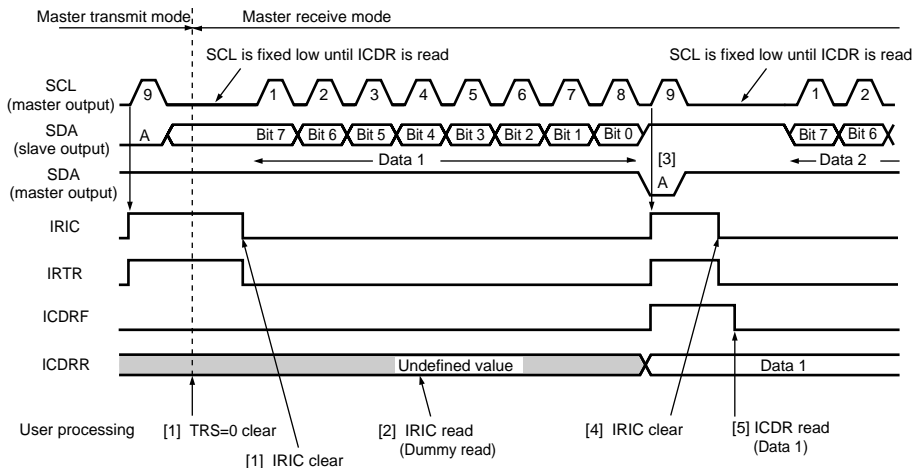
Figure 16.12 Example of Operation Timing in Master Receive Mode (MLS = WAIT = 0, HNDS = 1)
