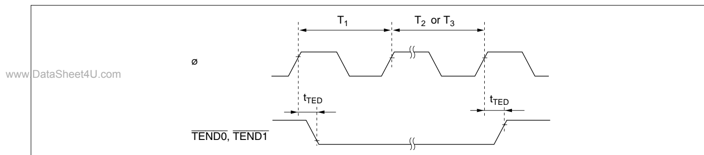
Figure 22-20 DMAC \overline{TEND} Output Timing
