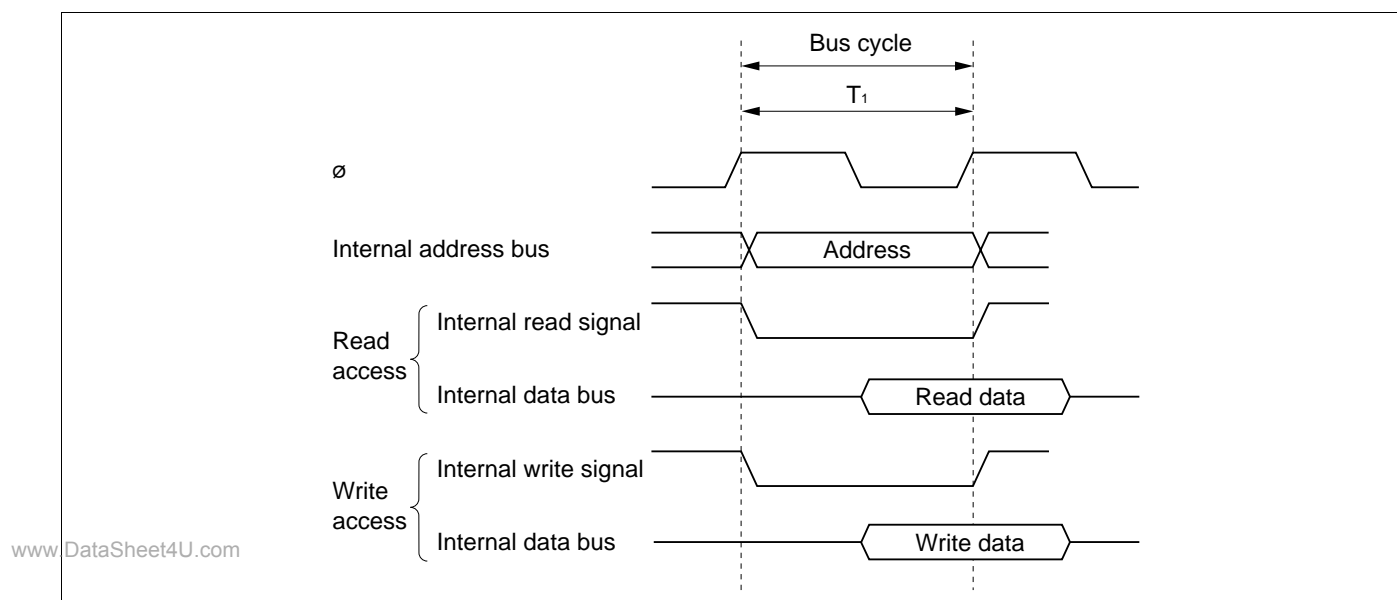
Figure 2-14 On-Chip Memory Access Cycle
