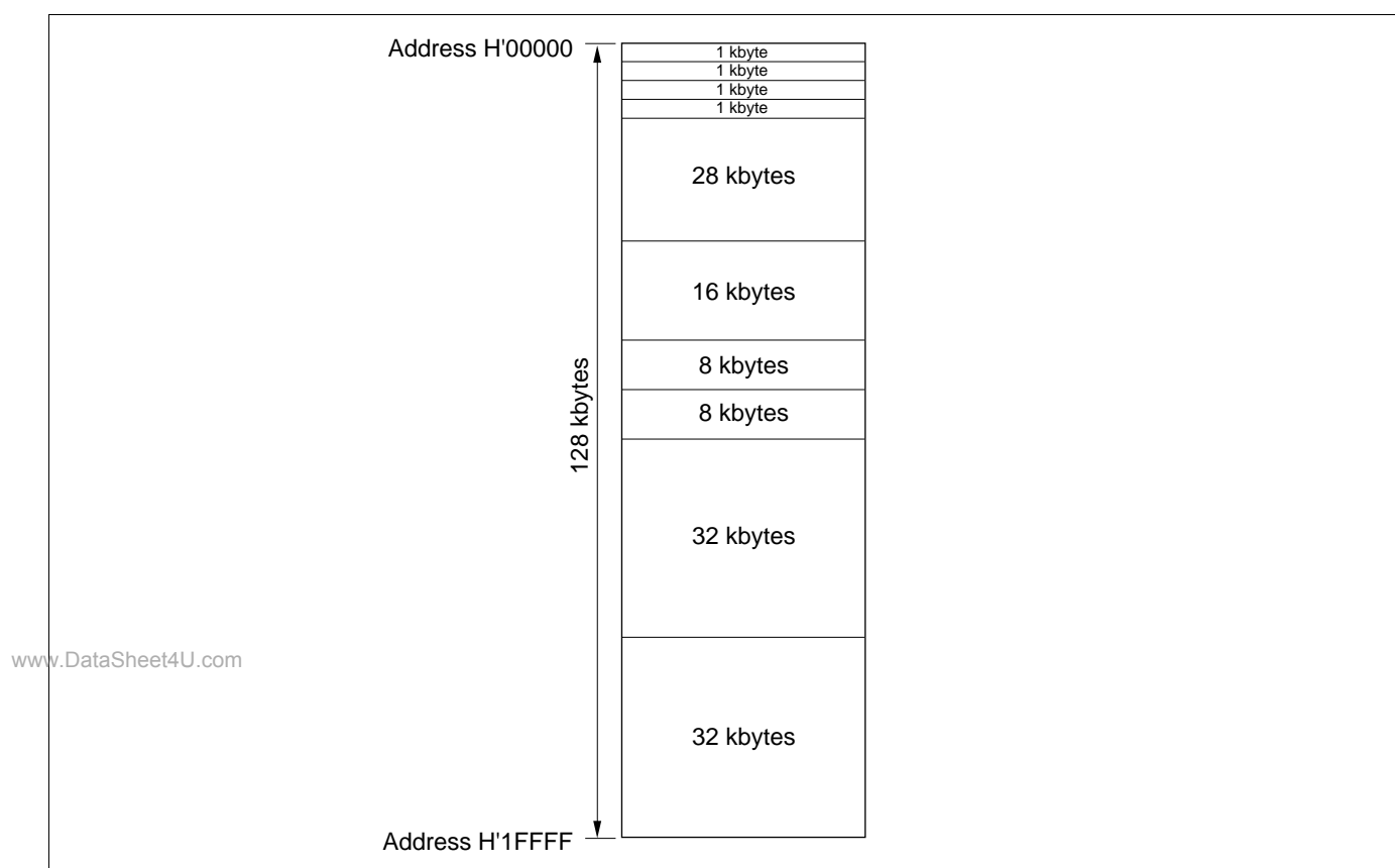
Figure 19-13 Flash Memory Block Configuration
