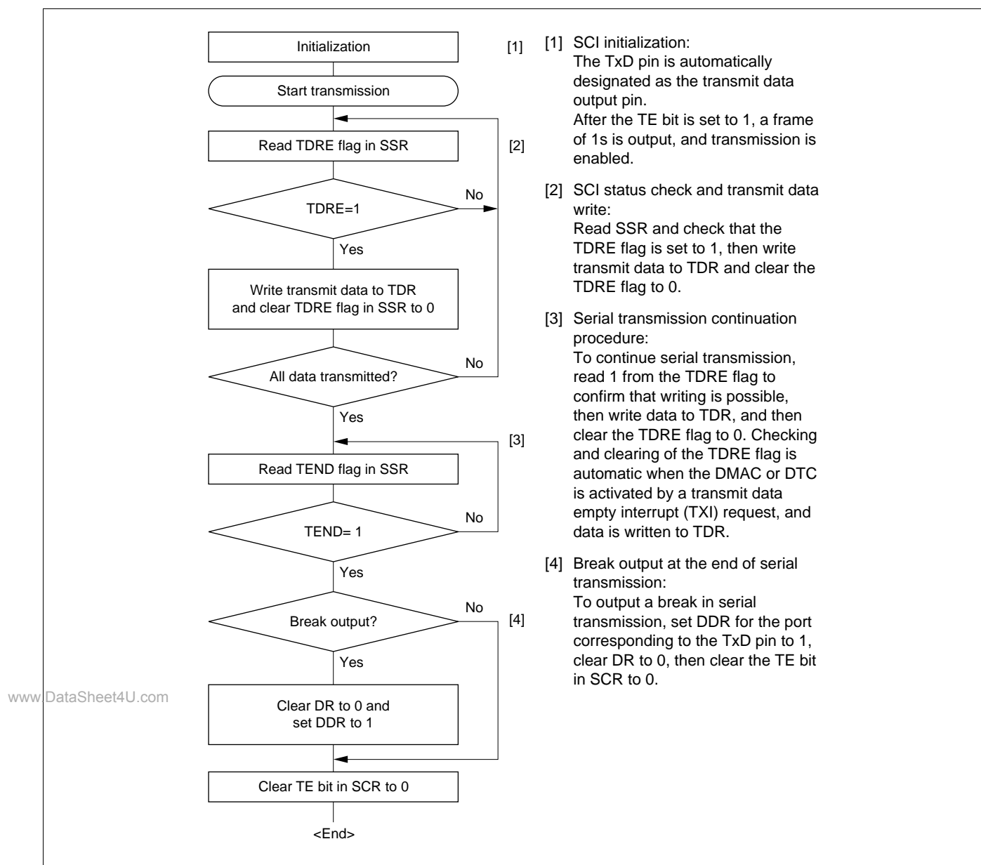
Figure 14-5 Sample Serial Transmission Flowchart
