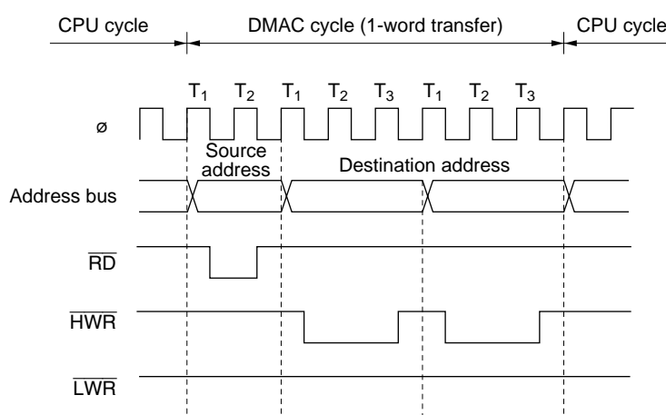
Figure 7-18 Example of DMA Transfer Bus Timing
