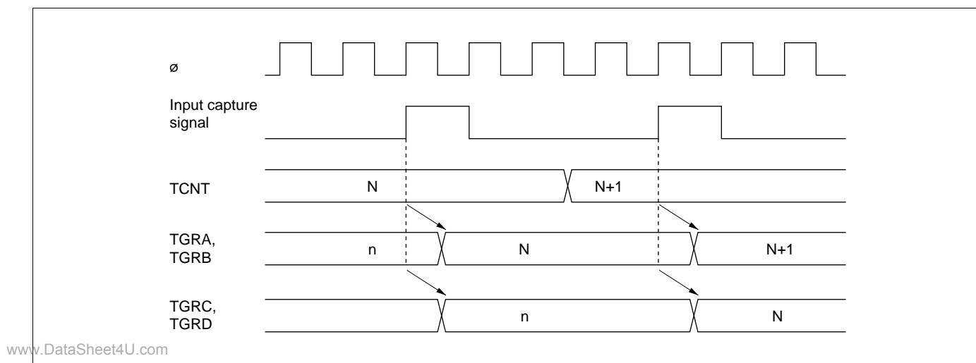
Figure 10-41 Buffer Operation Timing (Input Capture)
