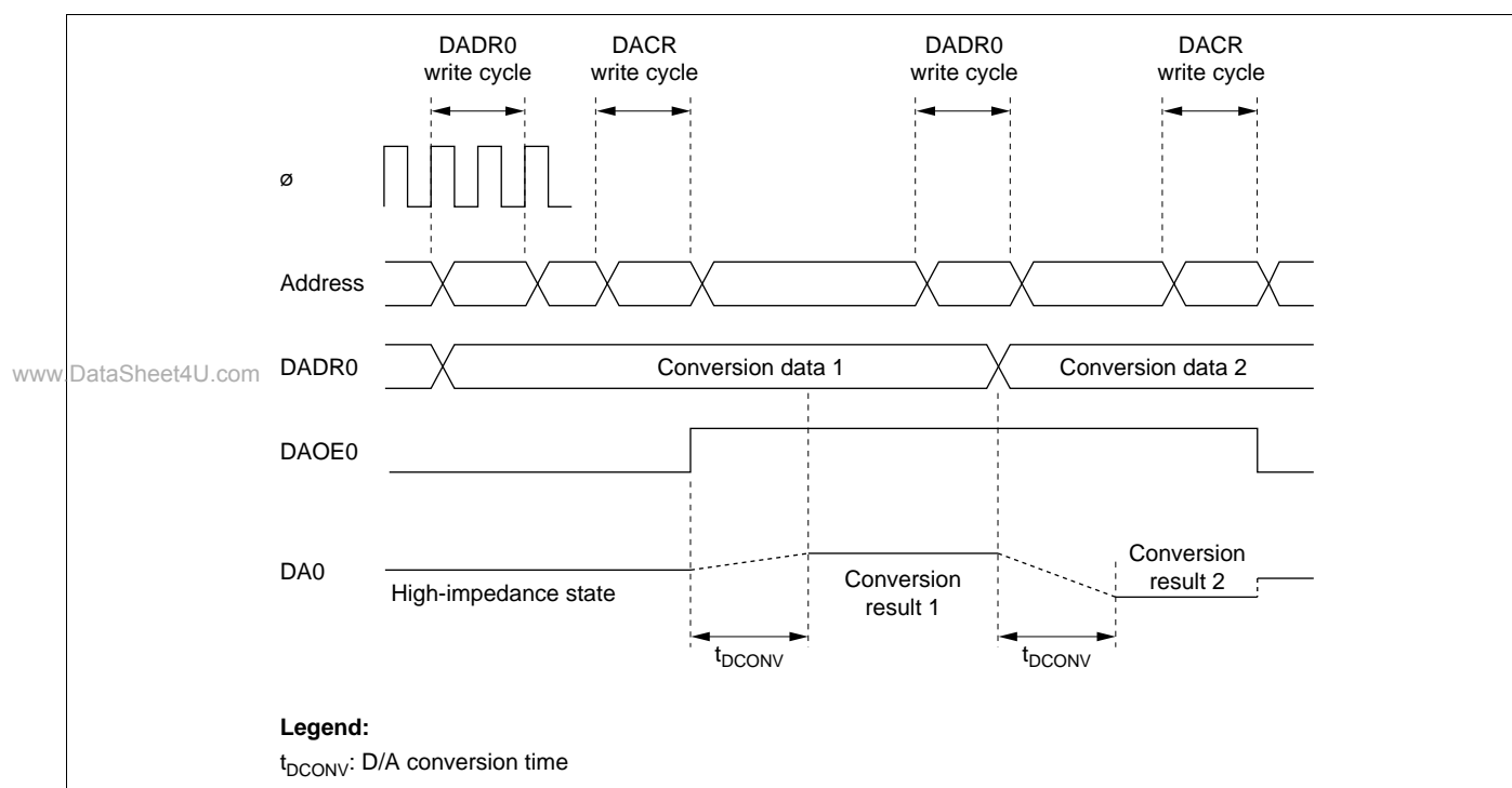
Figure 17-2 Example of D/A Converter Operation
