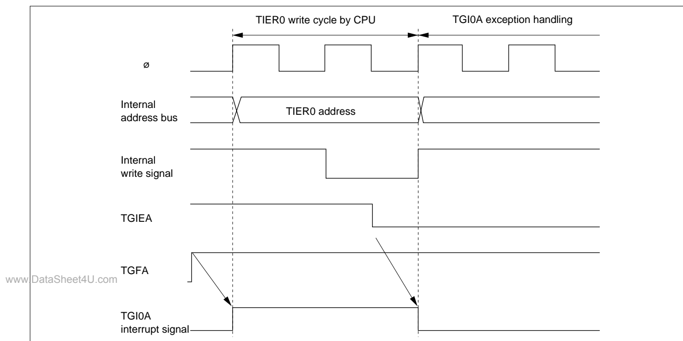
Figure 5-8 Contention between Interrupt Generation and Disabling
