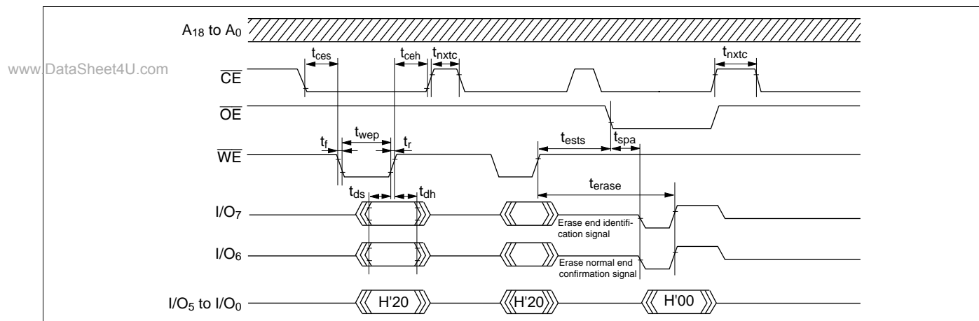
Figure 19-60 Auto-Erase Mode Timing Waveforms
