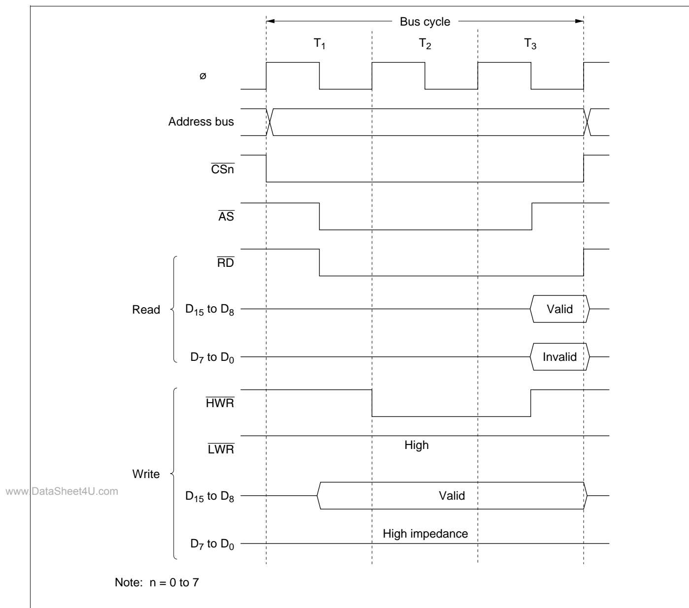
Figure 6-7 Bus Timing for 8-Bit 3-State Access Space
