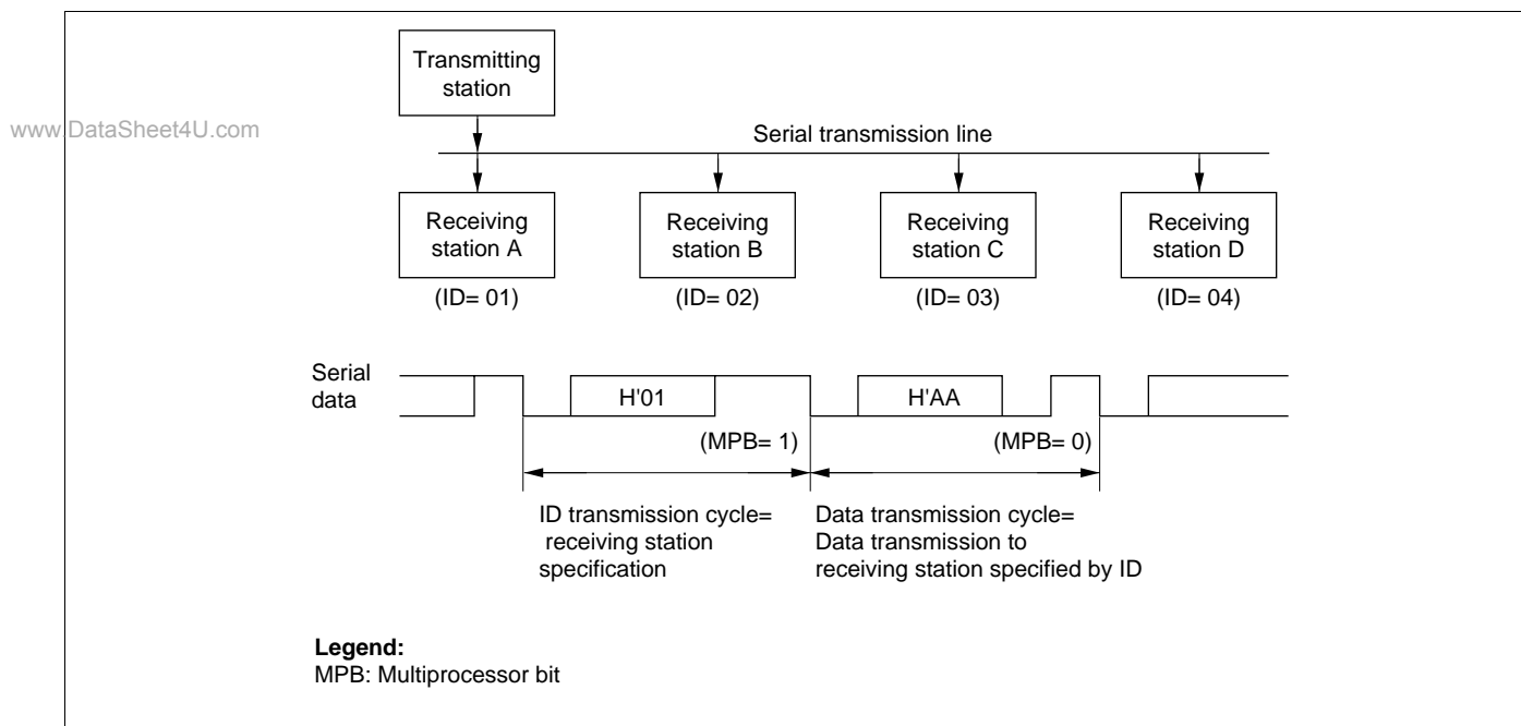
Figure 14-9 Example of Inter-Processor Communication Using Multiprocessor Format (Transmission of Data H'AA to Receiving Station A)
