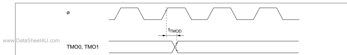
Figure 22-90 8-Bit Timer Output Timing
