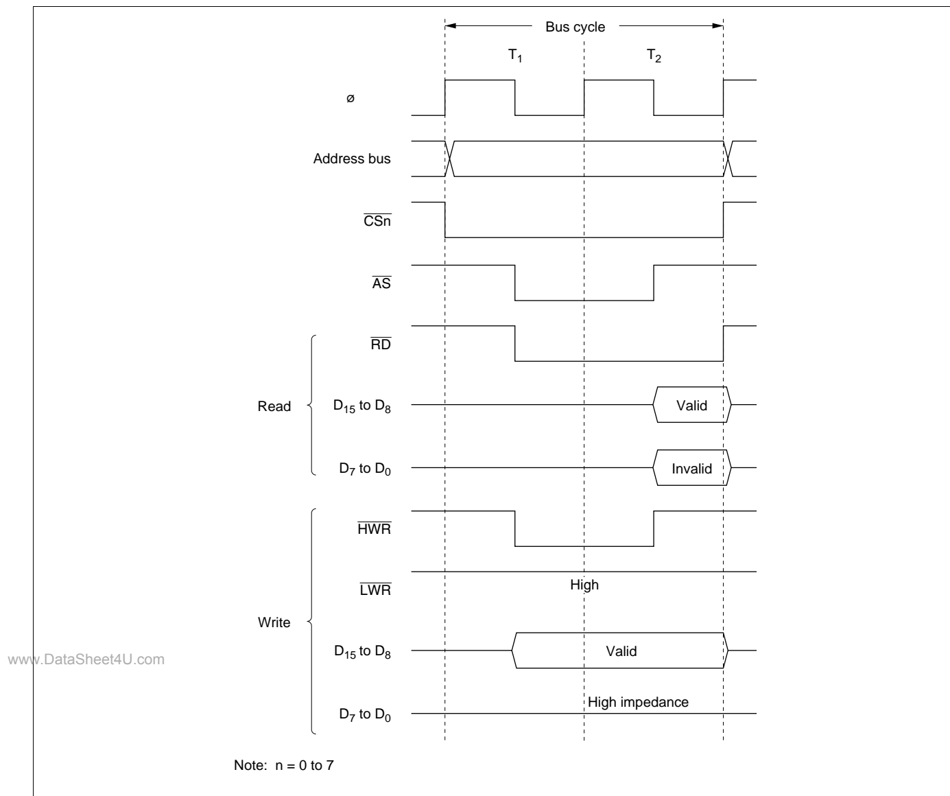
Figure 6-8 Bus Timing for 16-Bit 2-State Access Space (1) (Even Address Byte Access)
