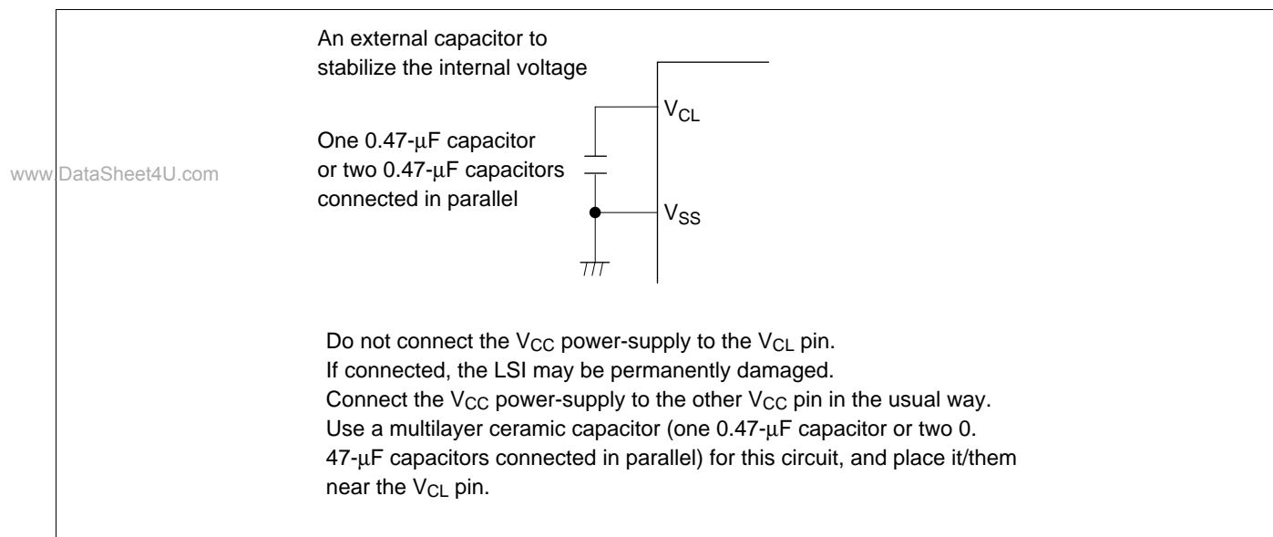
Figure 22-64 V_{CL} Capacitor Connection Method
