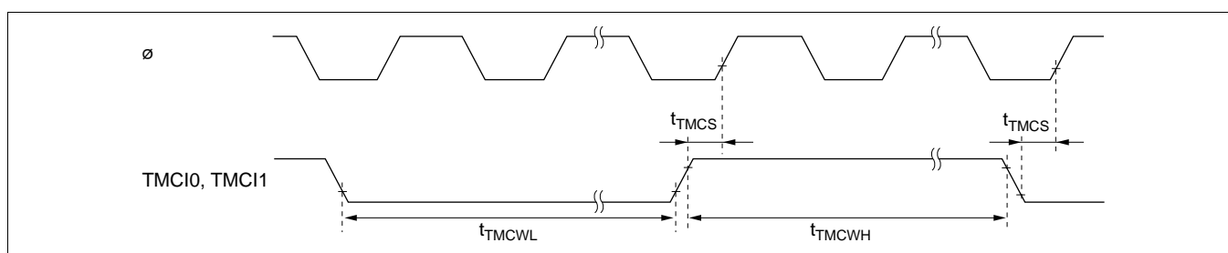
Figure 22-27 8-Bit Timer Clock Input Timing
