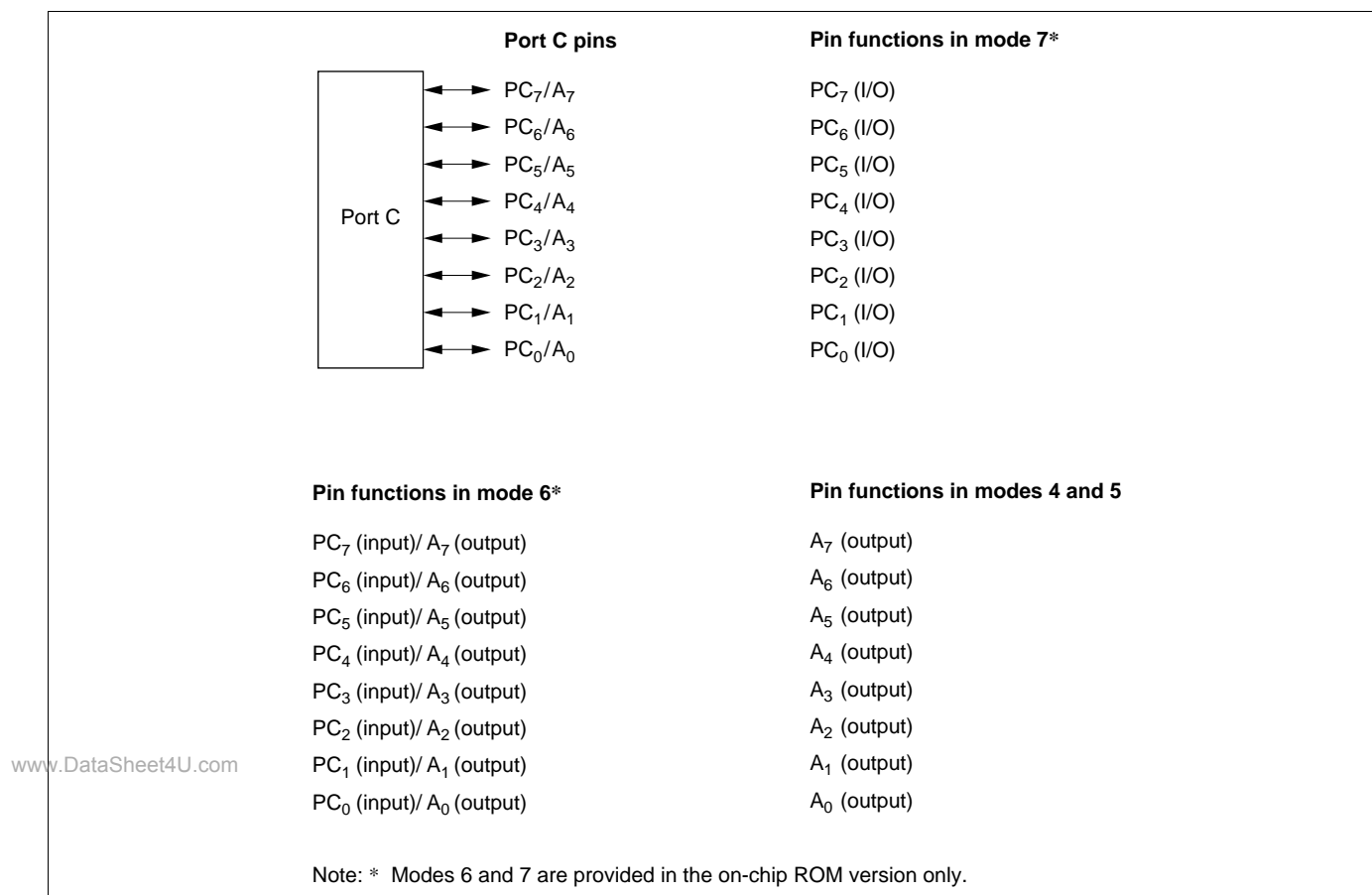
Figure 9-15 Port C Pin Functions
