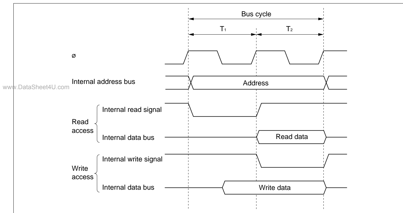
Figure 2-16 On-Chip Supporting Module Access Cycle
