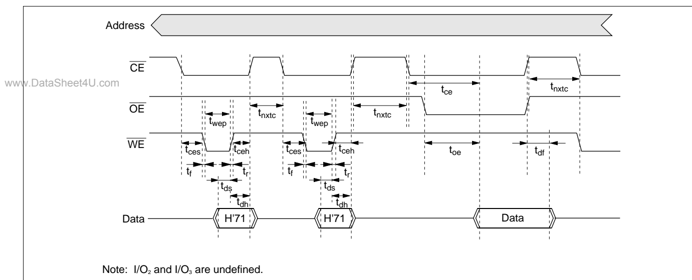
Figure 19-31 Status Read Mode Timing Waveforms
