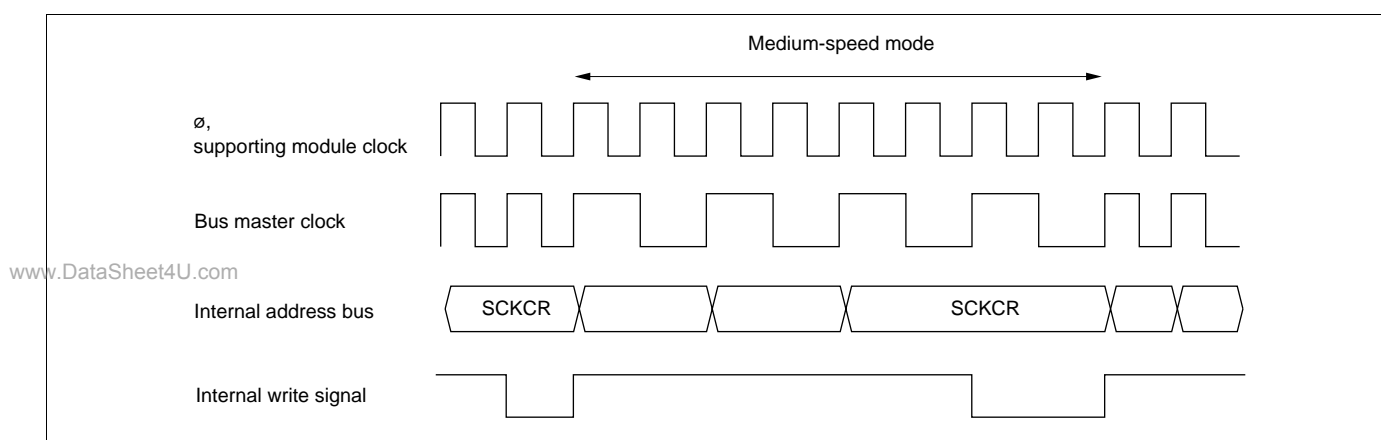
Figure 21-1 Medium-Speed Mode Transition and Clearance Timing
