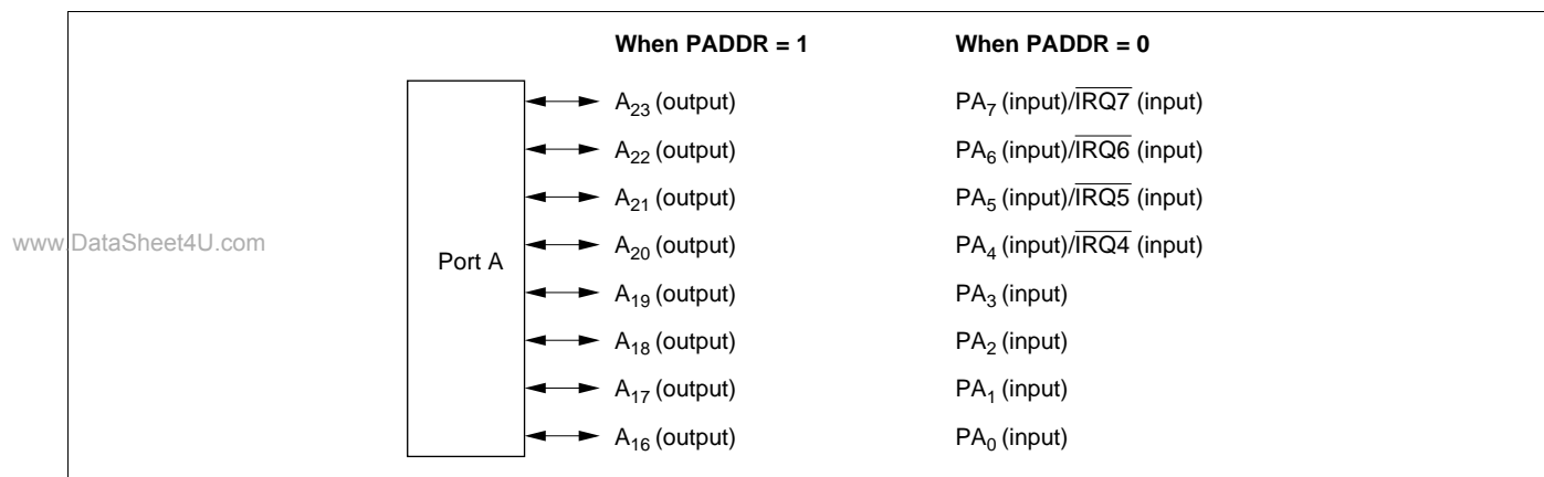
Figure 9-10 Port A Pin Functions (Modes 4 and 5)
