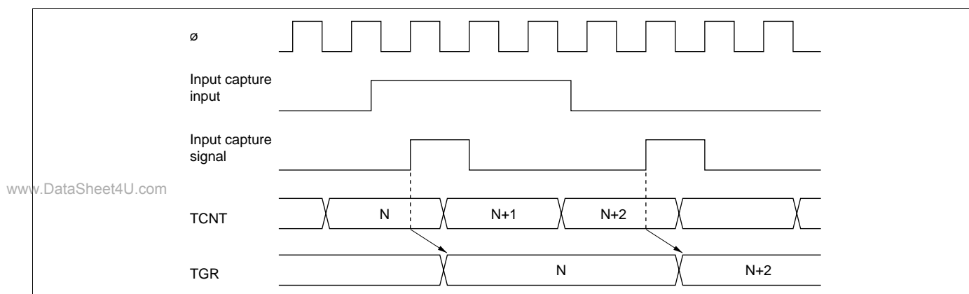
Figure 10-37 Input Capture Input Signal Timing
