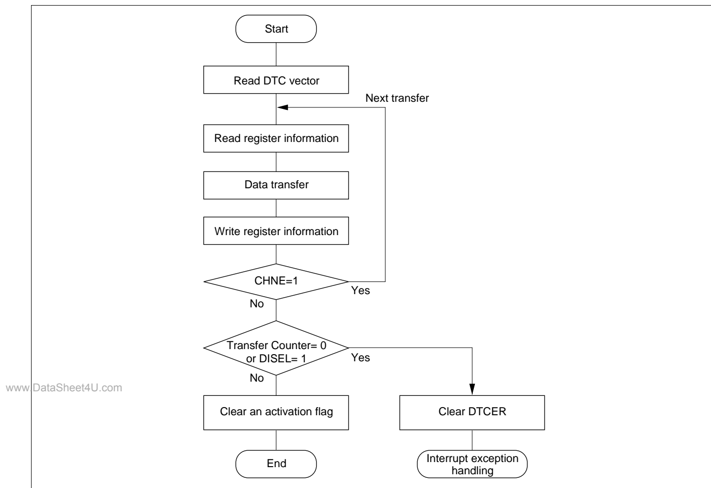
Figure 8-2 Flowchart of DTC Operation
