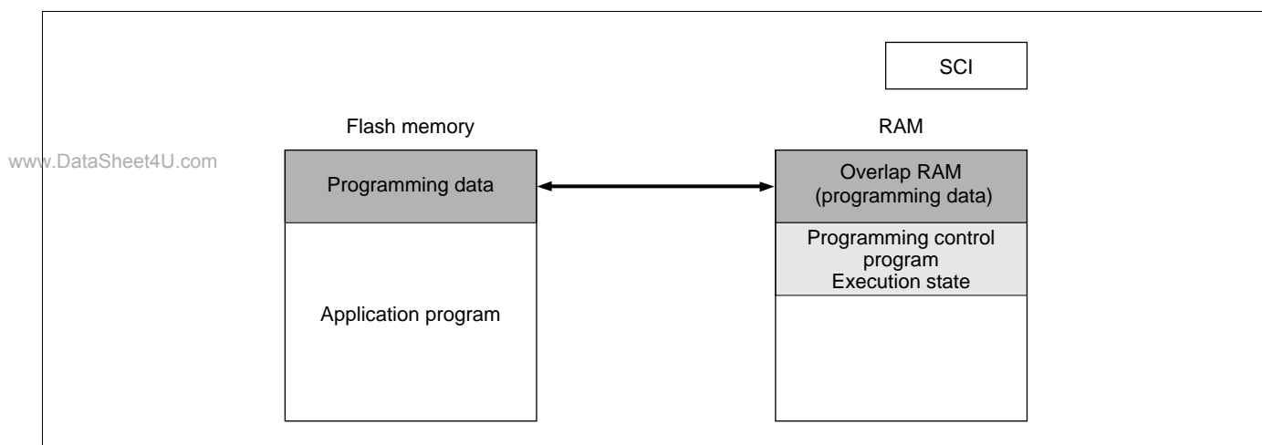
Figure 19-41 Writing Overlap RAM Data in User Program Mode
