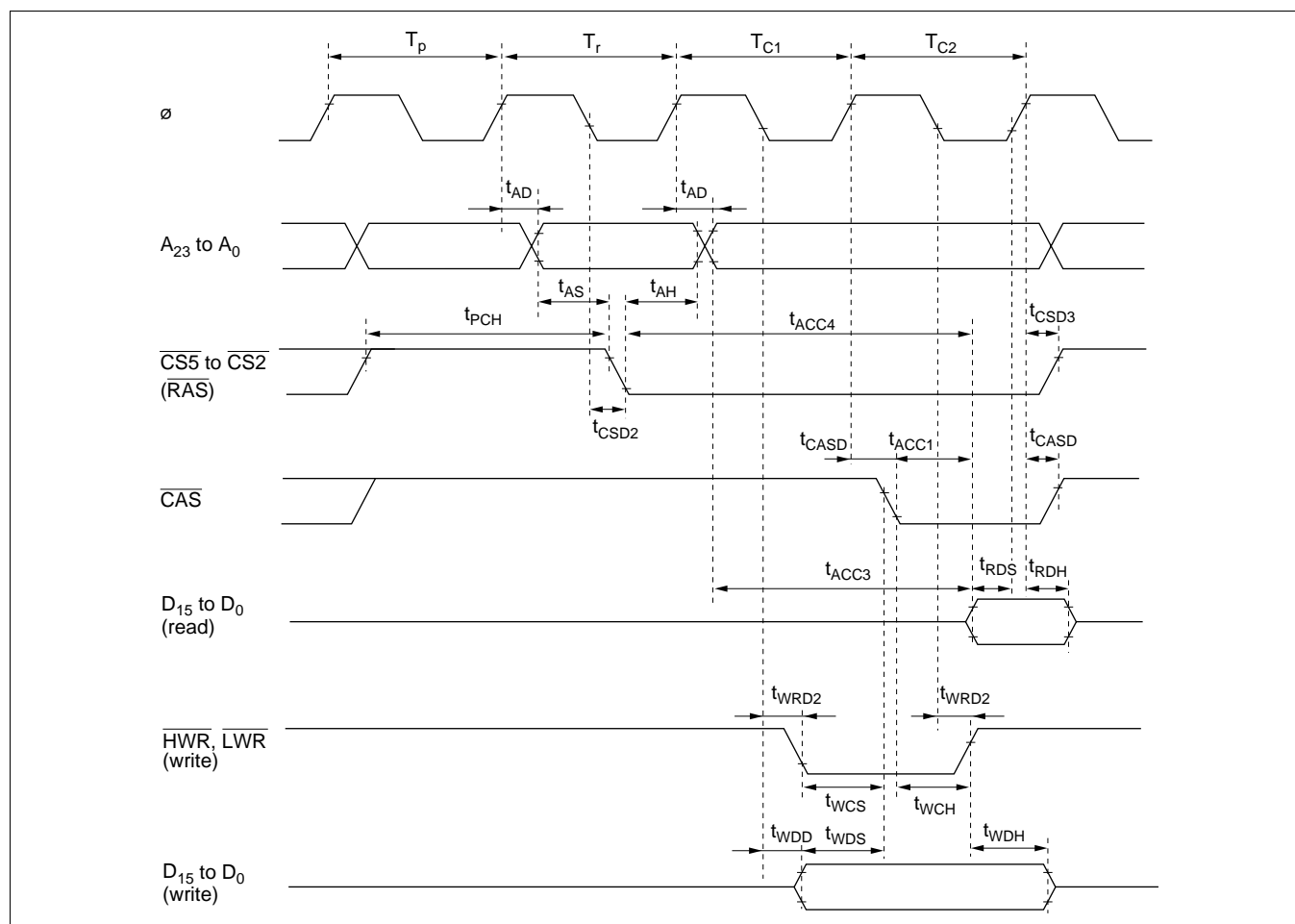
Figure 22-11 DRAM Bus Timing
