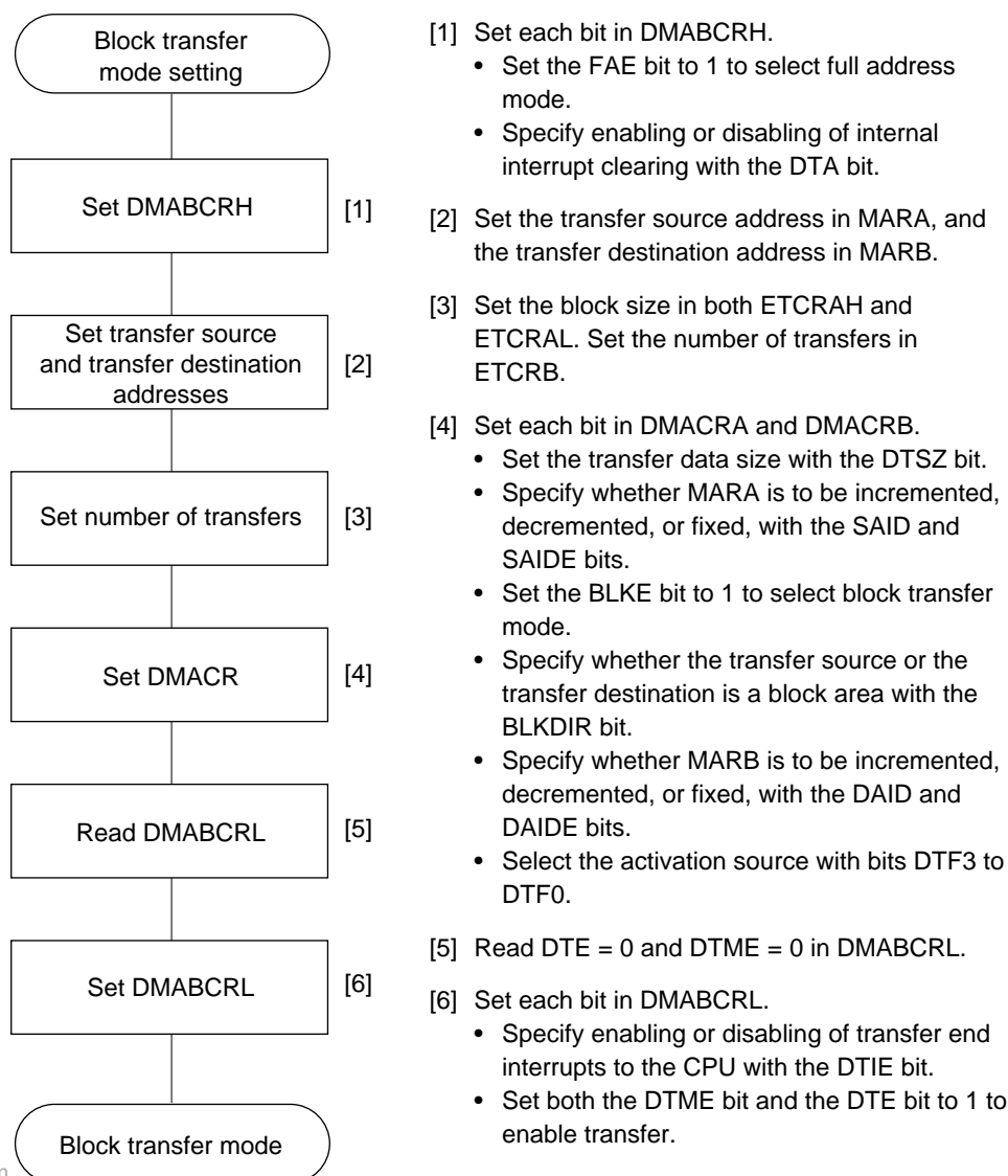
Figure 7-16 Example of Block Transfer Mode Setting Procedure
