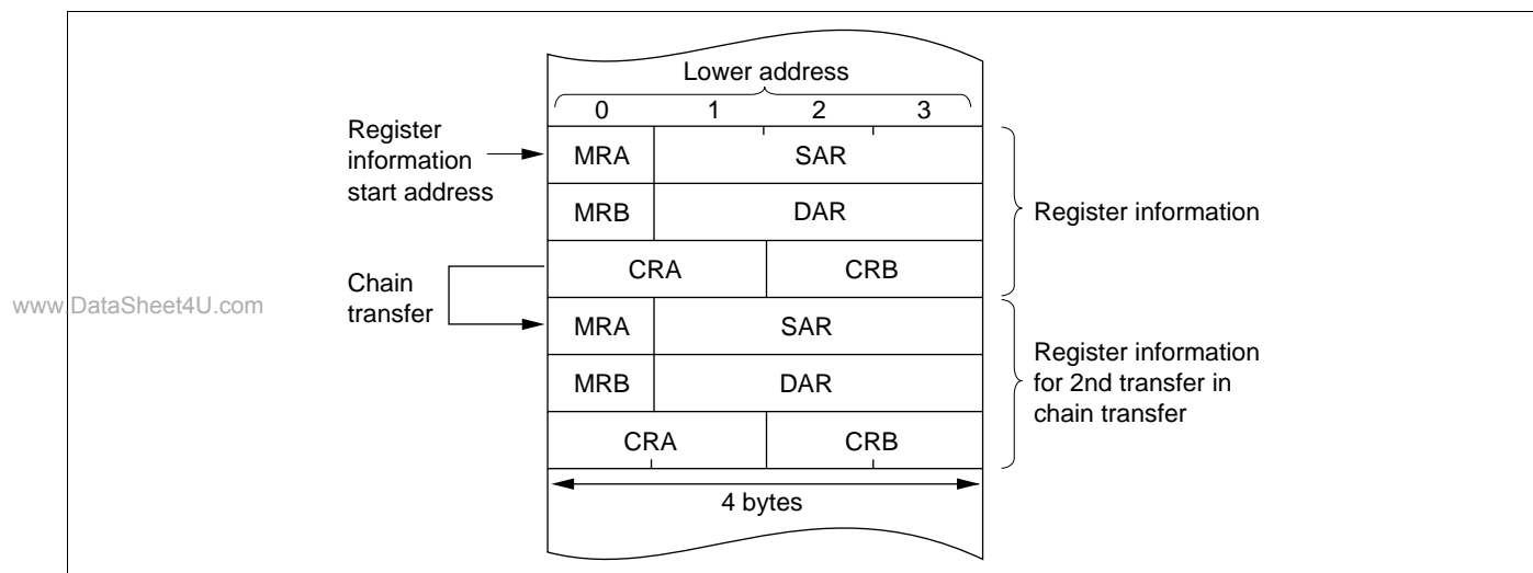
Figure 8-5 Location of Register Information in Address Space
