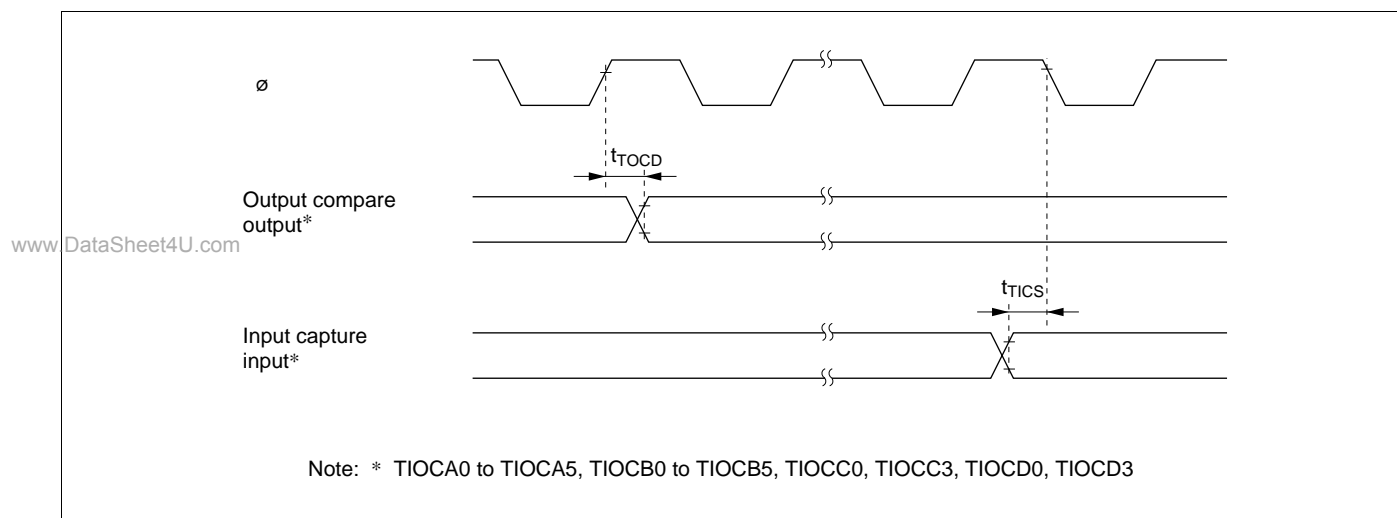
Figure 22-24 TPU Input/Output Timing
