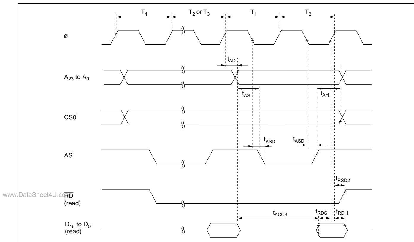
Figure 22-14 Burst ROM Access Timing (Two-State Access)
