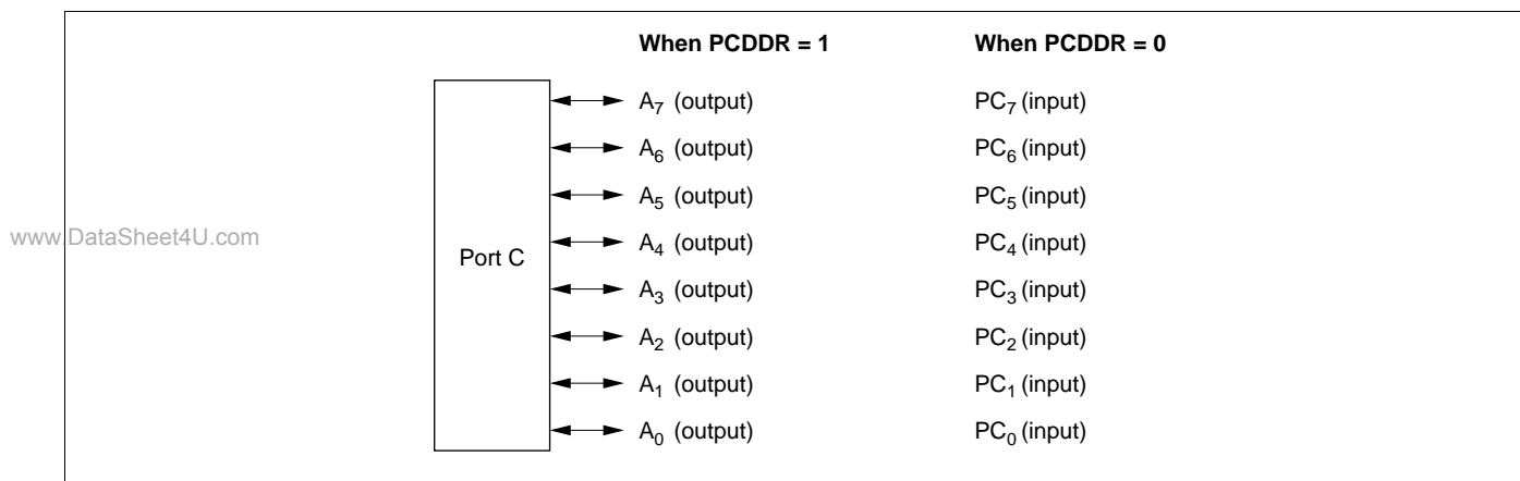
Figure 9-17 Port C Pin Functions (Mode 6)
