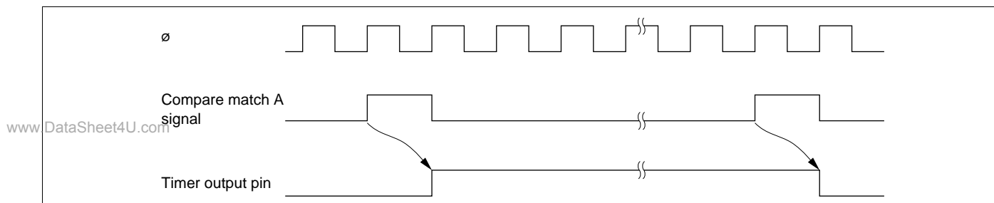
Figure 12-5 Timing of Timer Output
