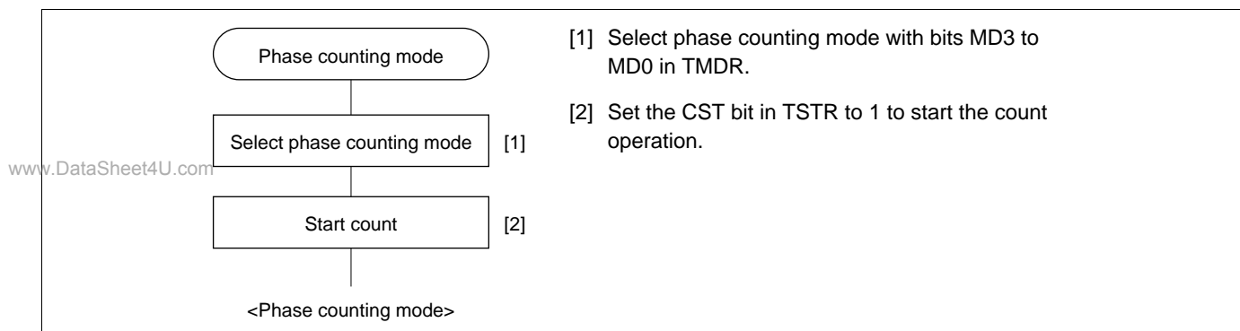
Figure 10-28 Example of Phase Counting Mode Setting Procedure
