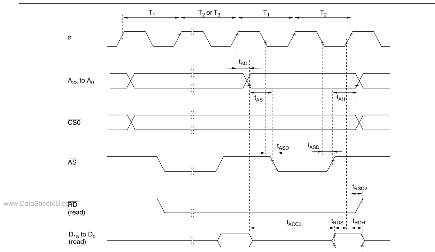
Figure 22-46 Burst ROM Access Timing (Two-State Access)
