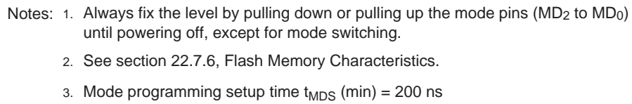
Figure 19-33 Powering On/Off Timing (Boot Mode)
