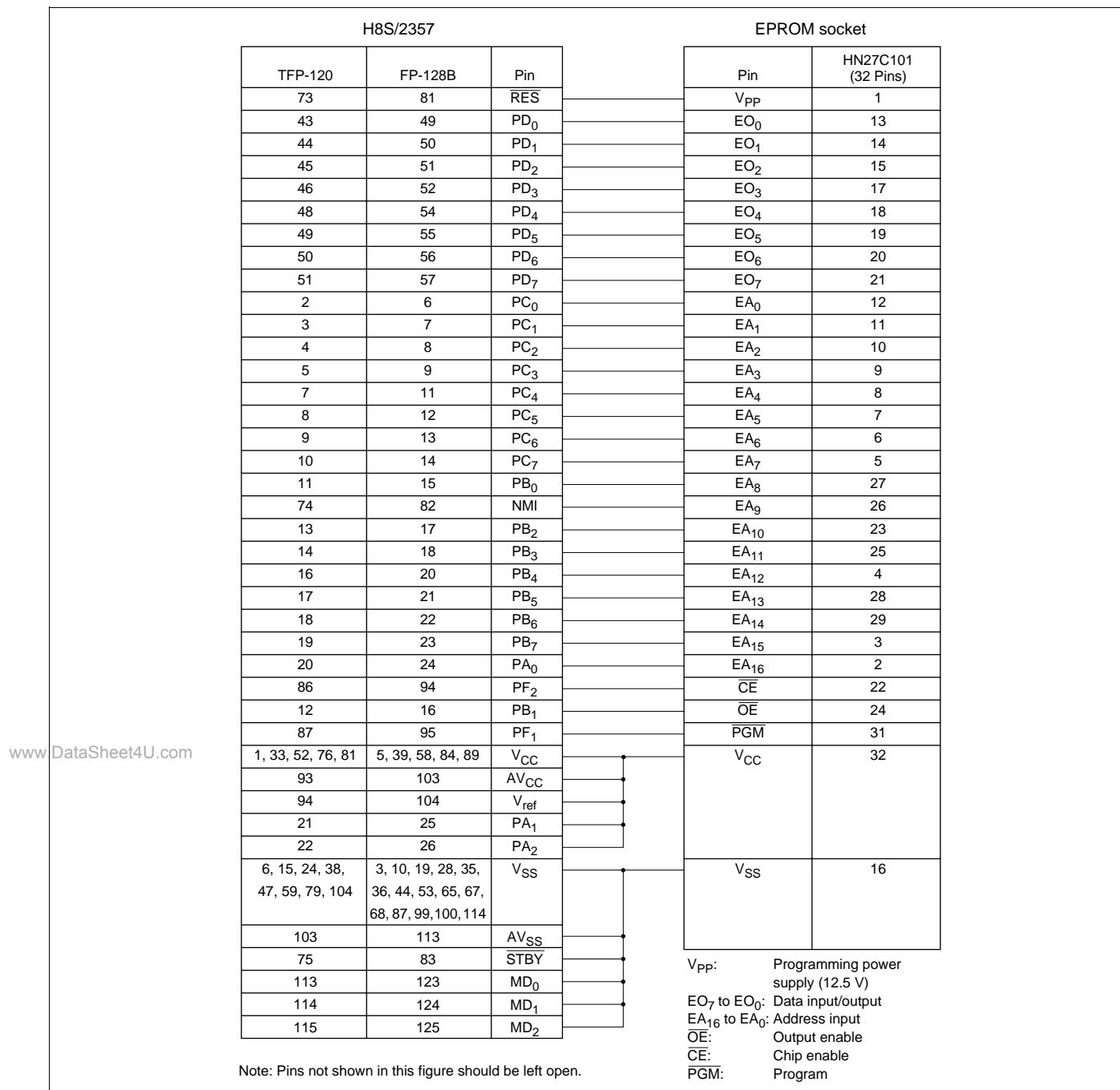
Figure 19-2 Wiring of 120/128B-Pin Socket Adapter
