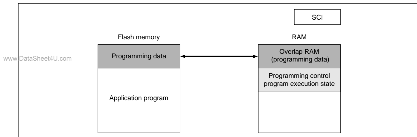
Figure 19-12 Writing Overlap Data in User Program Mode
