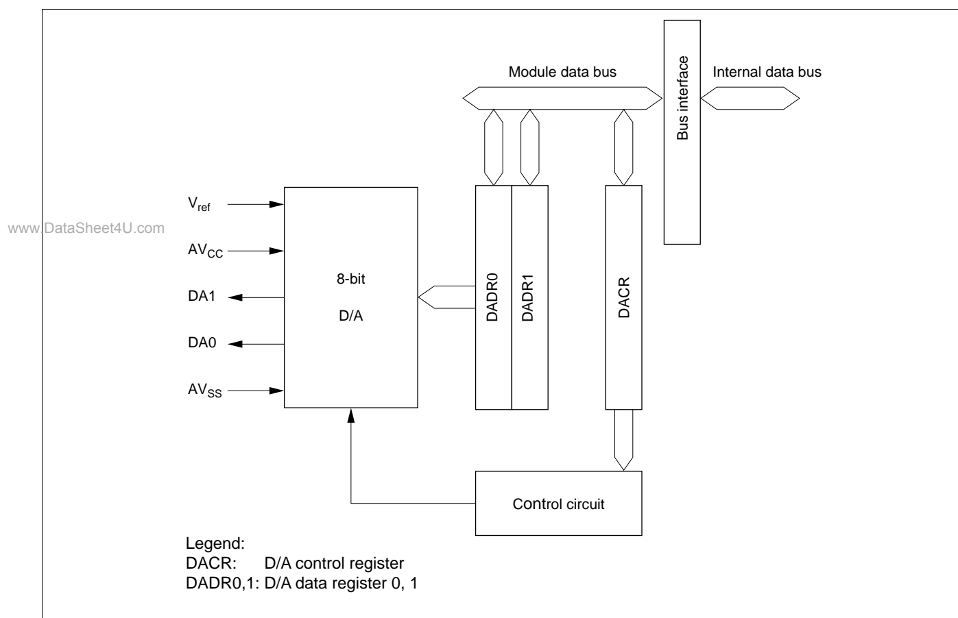
Figure 17-1 Block Diagram of D/A Converter
