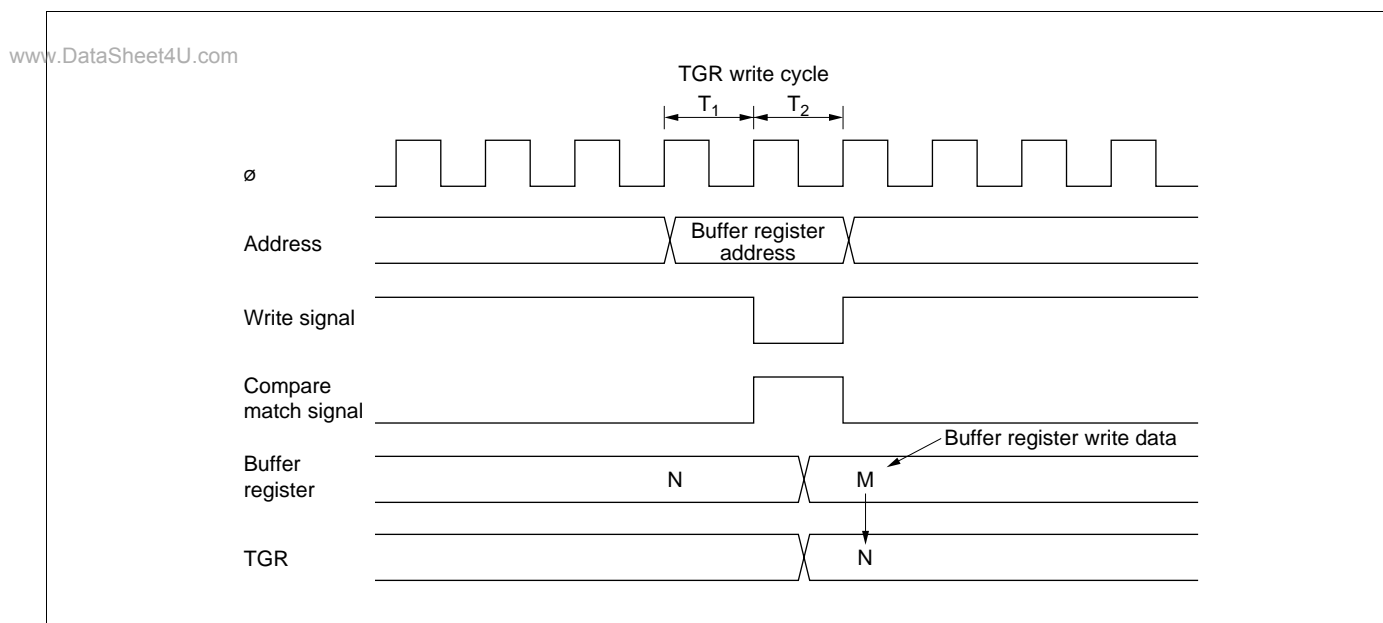
Figure 10-52 Contention between Buffer Register Write and Compare Match
