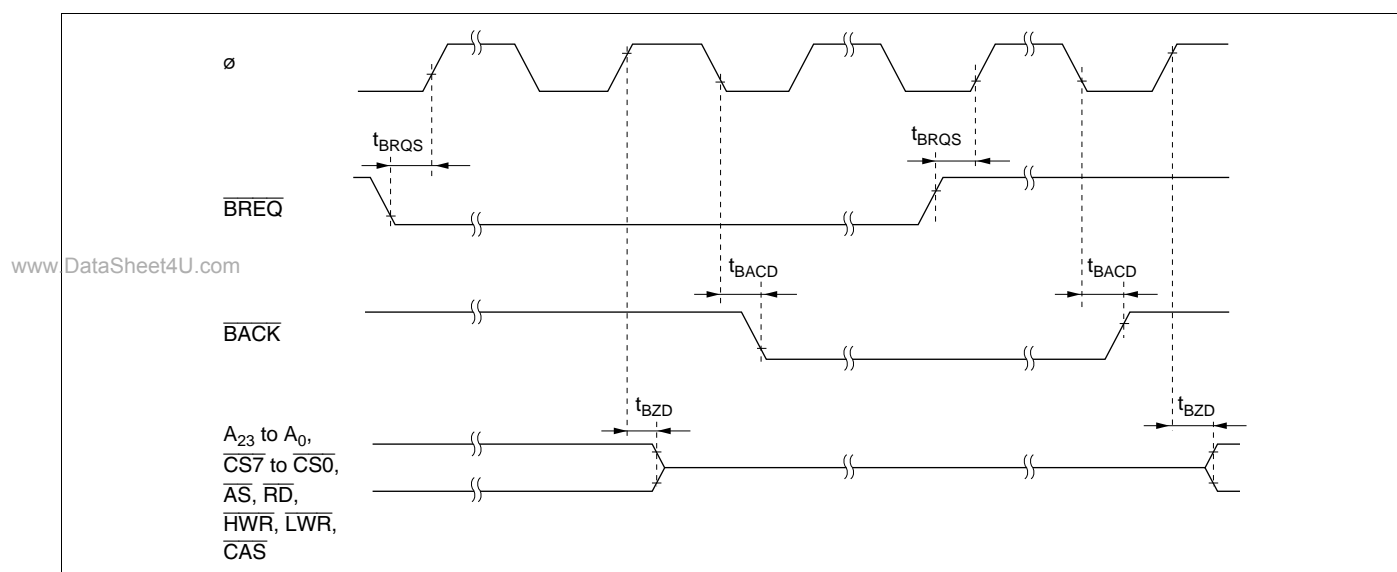
Figure 22-80 External Bus Release Timing
