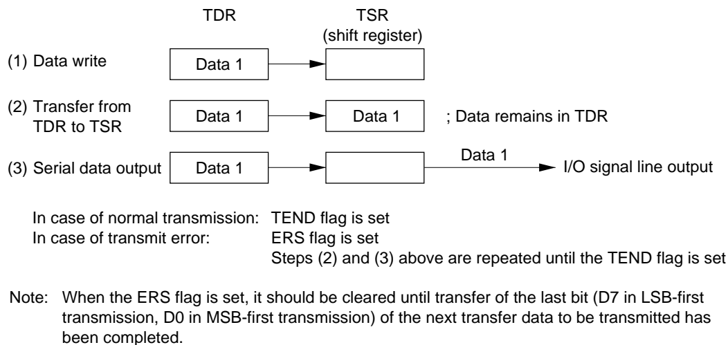
Figure 15-5 Relation Between Transmit Operation and Internal Registers
