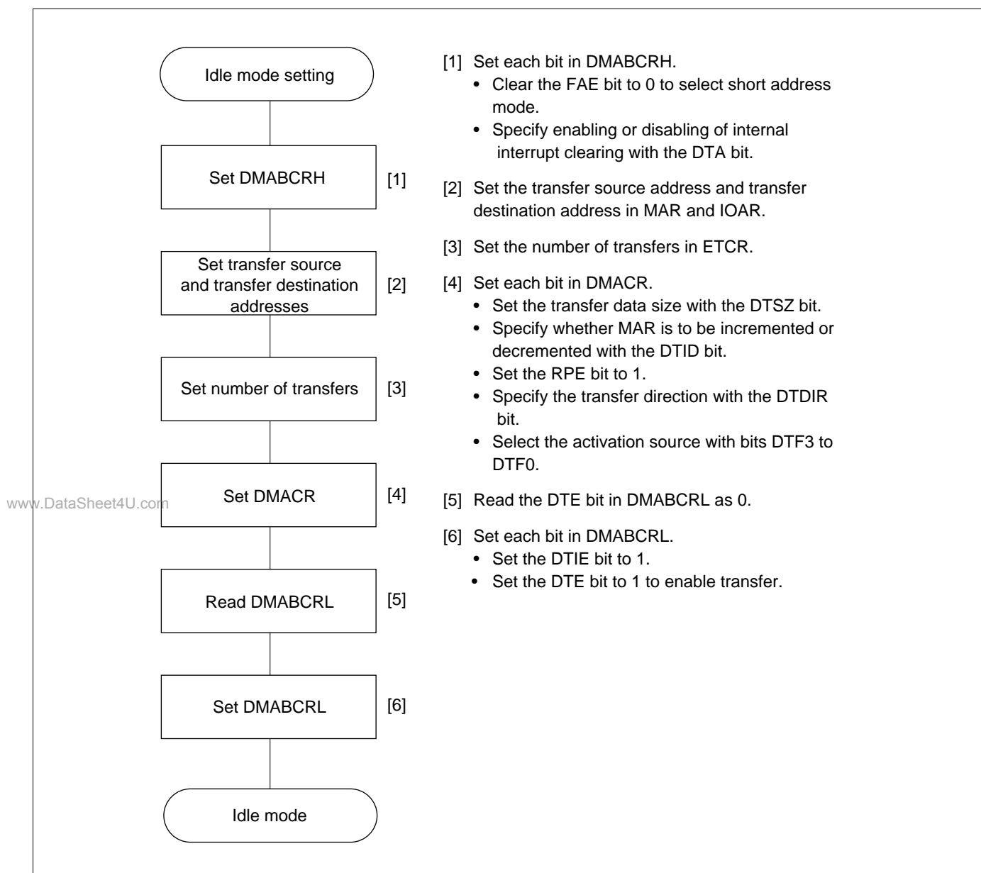
Figure 7-6 Example of Idle Mode Setting Procedure
