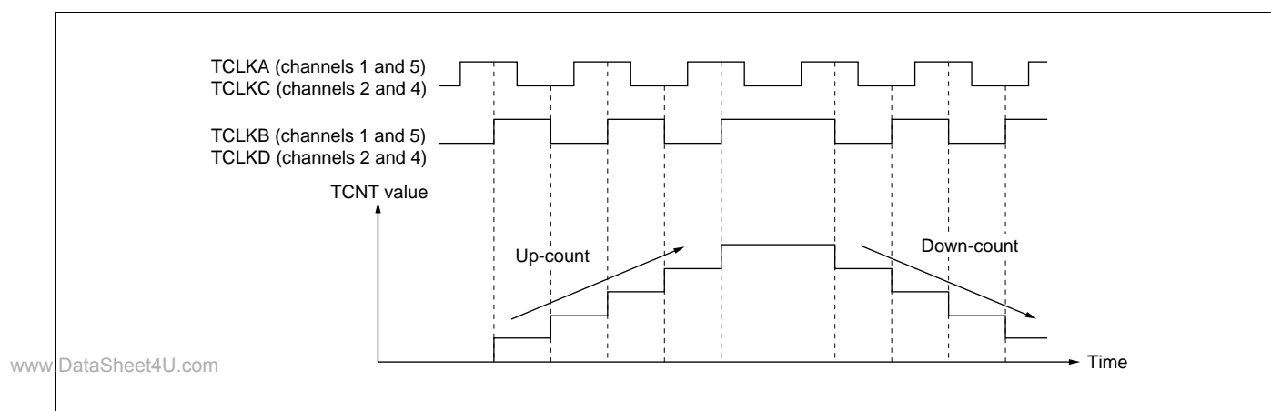
Figure 10-32 Example of Phase Counting Mode 4 Operation
