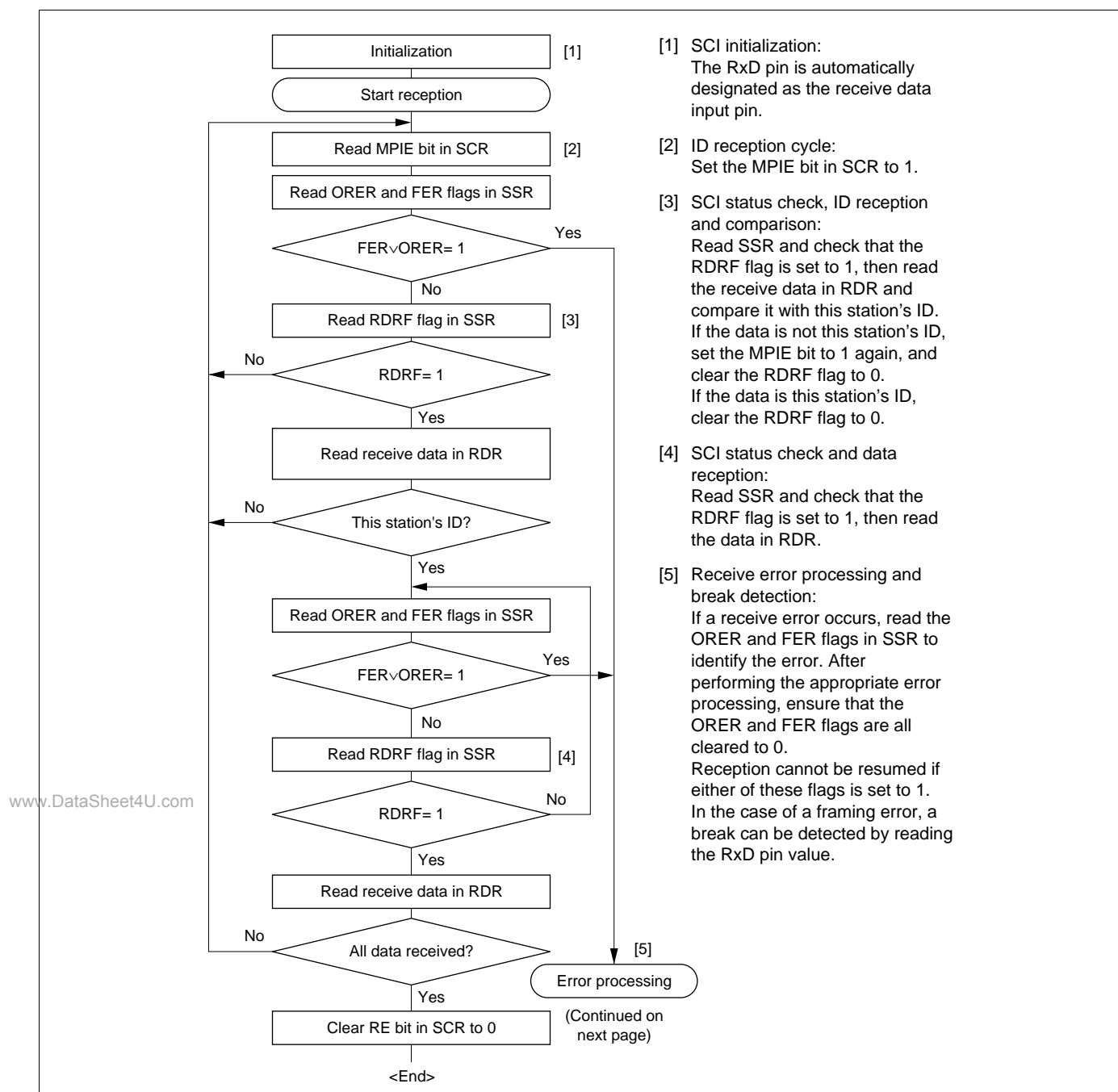
Figure 14-12 Sample Multiprocessor Serial Reception Flowchart
