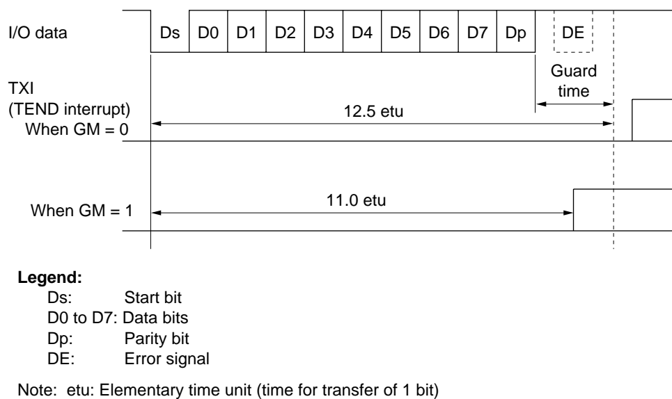
Figure 15-6 TEND Flag Generation Timing in Transmission Operation
