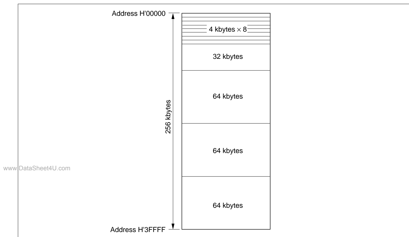
Figure 19-42 Flash Memory Block Configuration
