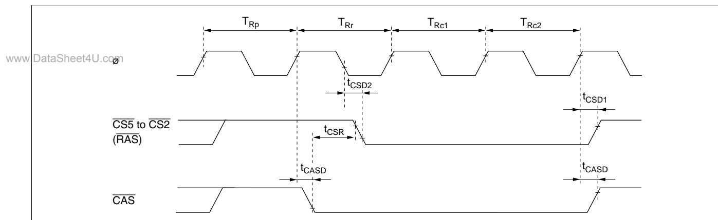
Figure 22-76 CAS-Before-RAS Refresh Timing
