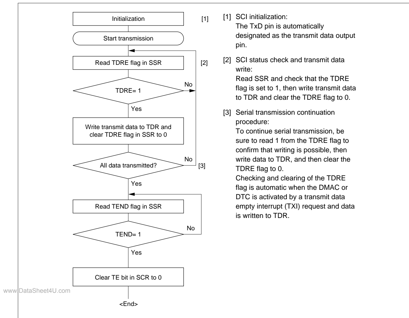
Figure 14-16 Sample Serial Transmission Flowchart
