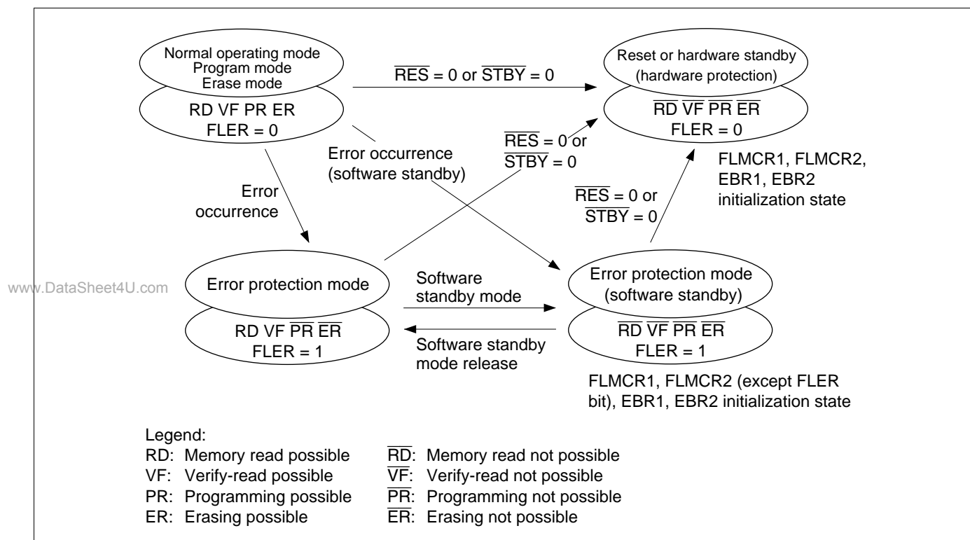
Figure 19-50 Flash Memory State Transitions
