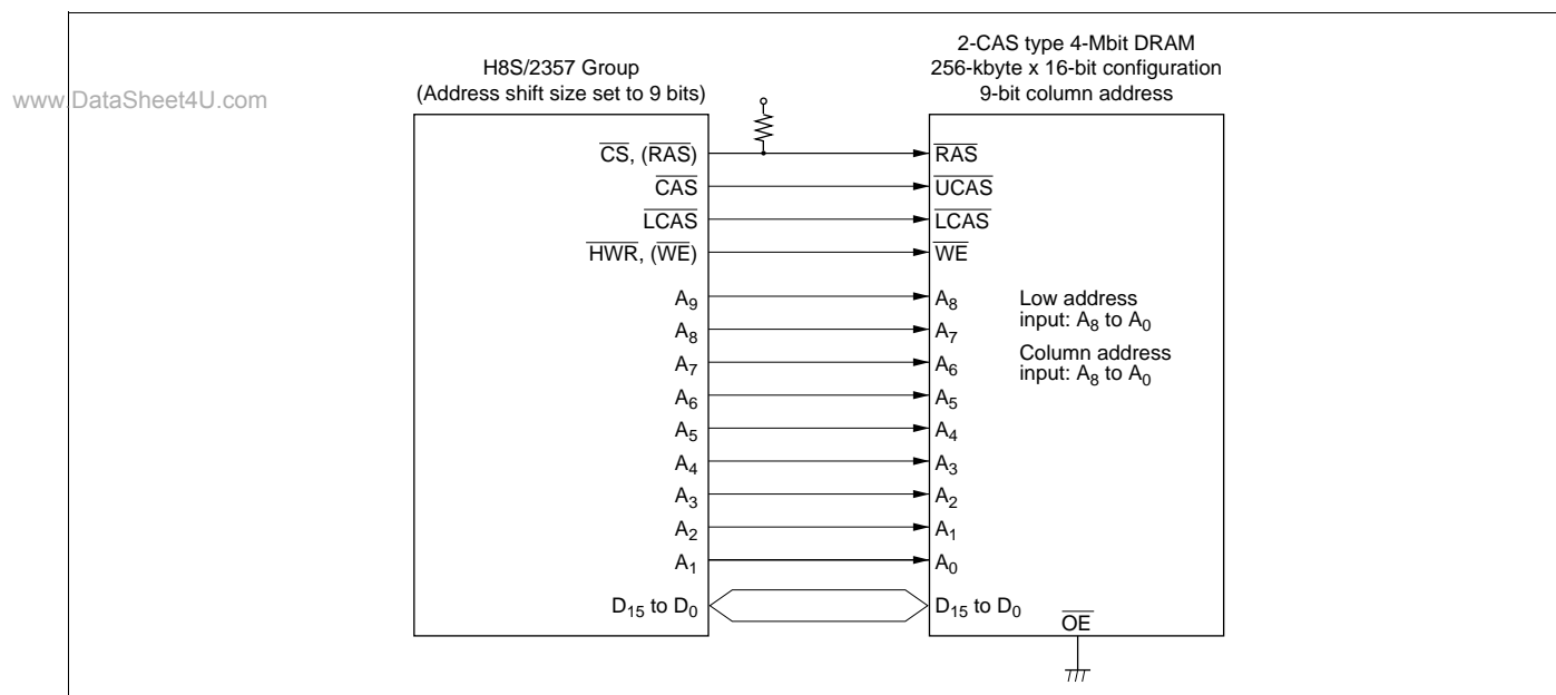
Figure 6-19 Example of 2-CAS System Connection
