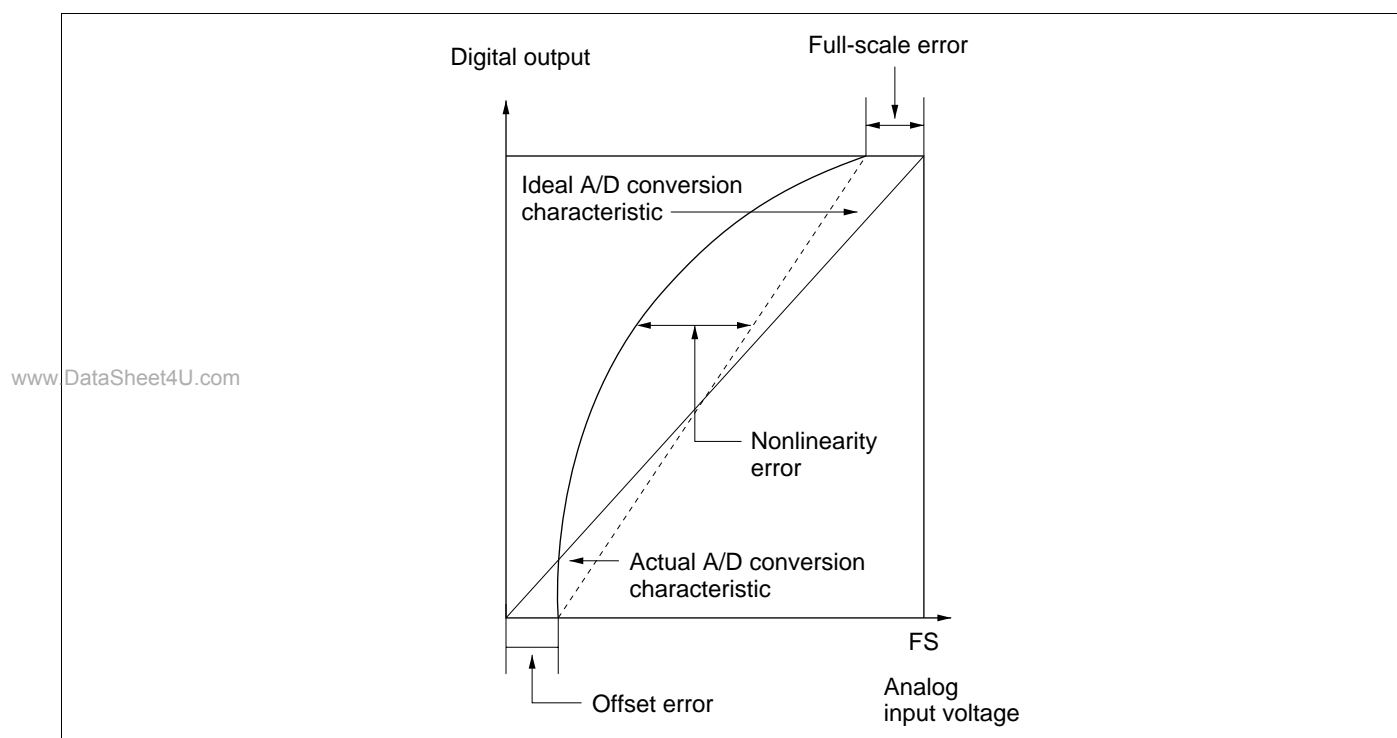
Figure 16-9 A/D Conversion Precision Definitions (2)
