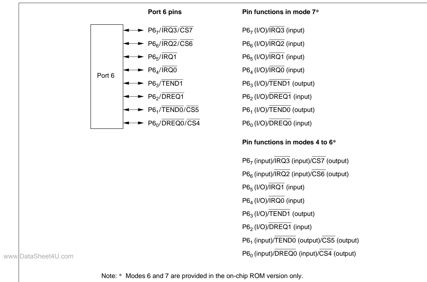
Figure 9-6 Port 6 Pin Functions
