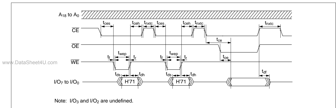
Figure 19-61 Status Read Mode Timing Waveforms
