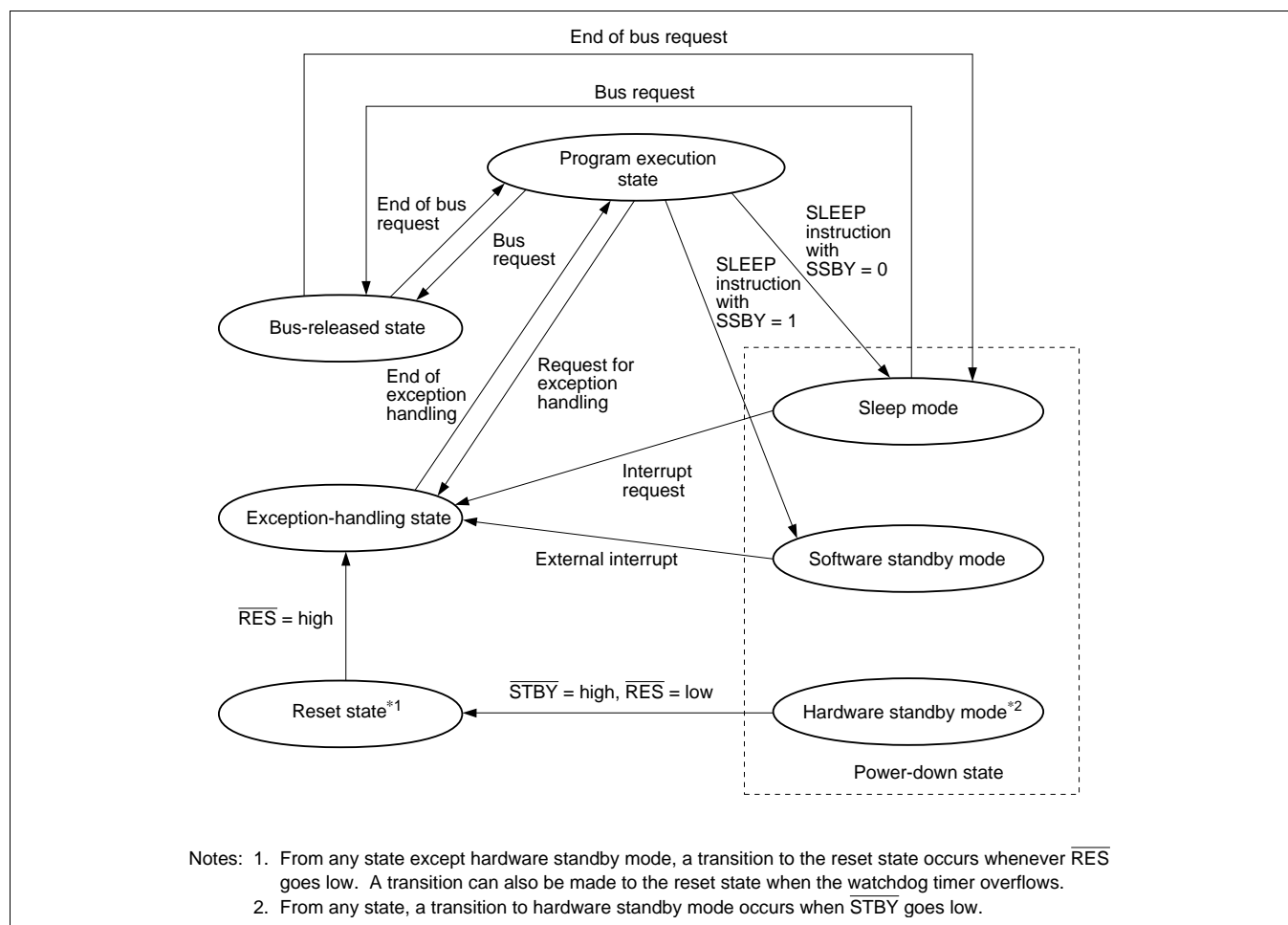
Figure 2-12 State Transitions
