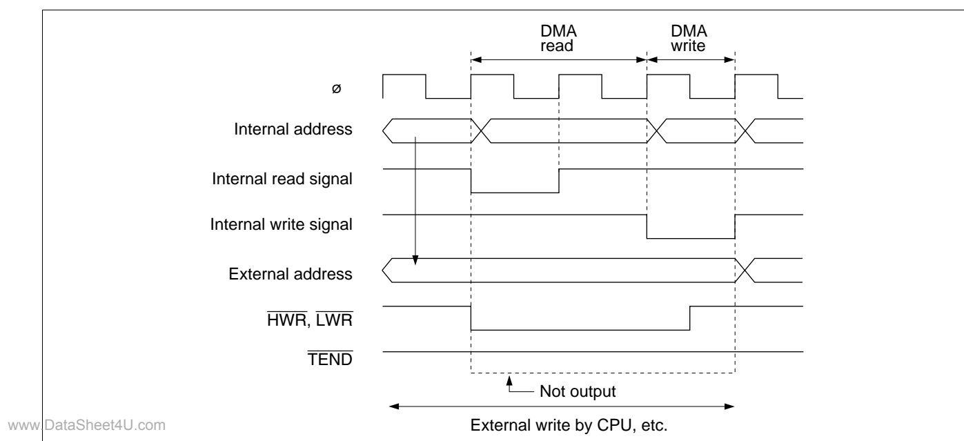
Figure 7-42 Example in Which Low Level is Not Output at \overline{\text{TEND}} Pin
