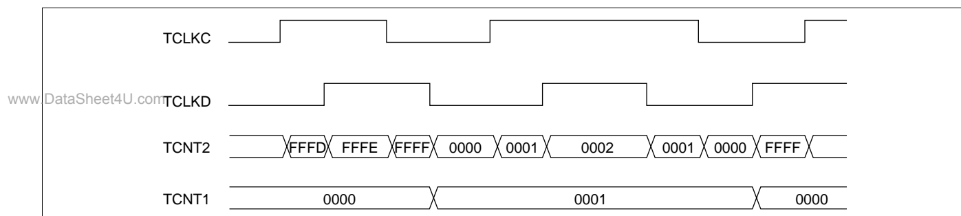
Figure 10-23 Example of Cascaded Operation (2)
