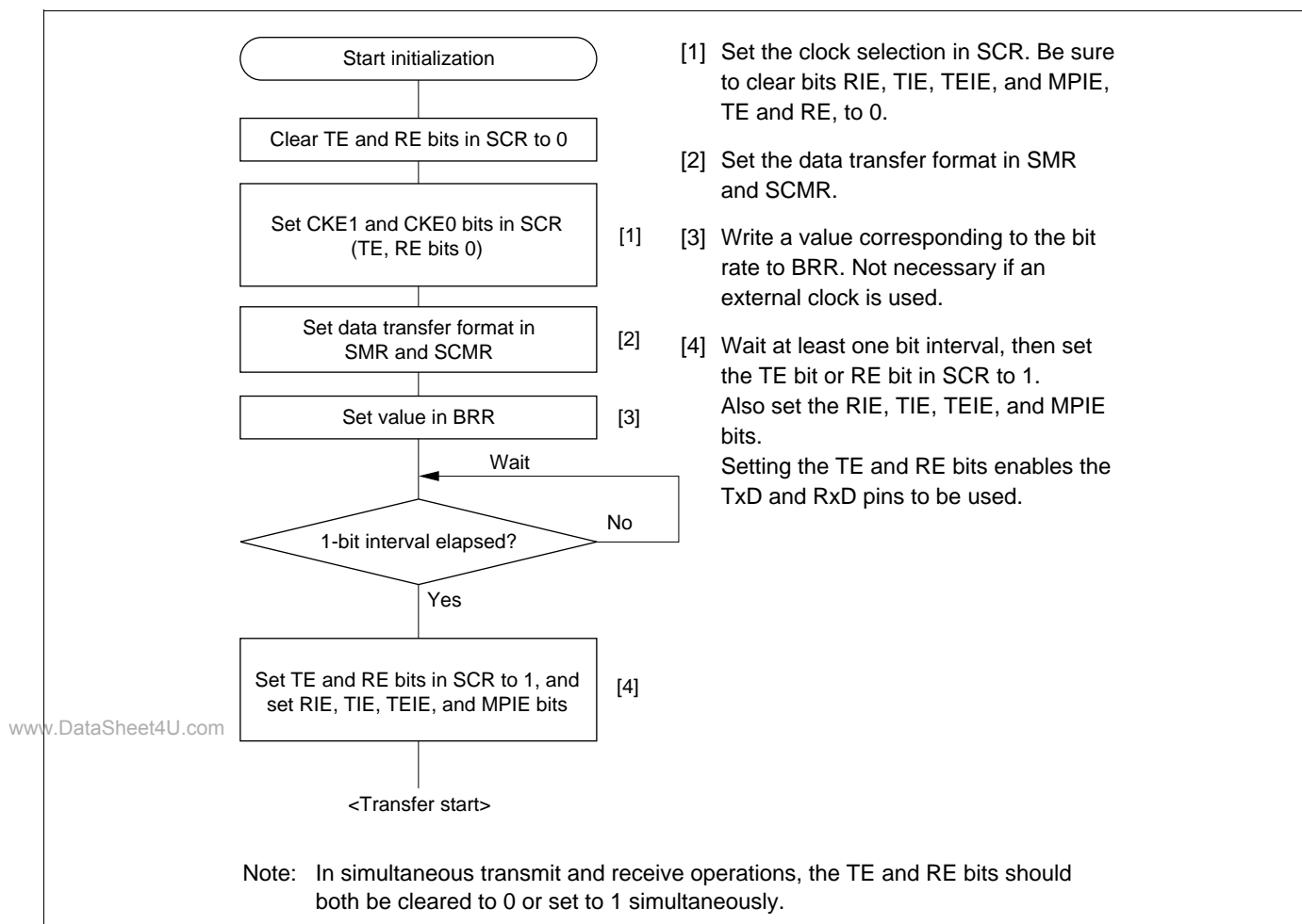
Figure 14-15 Sample SCI Initialization Flowchart
