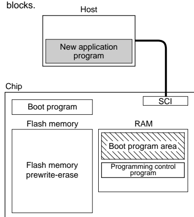
Figure 19-38 Boot Mode
