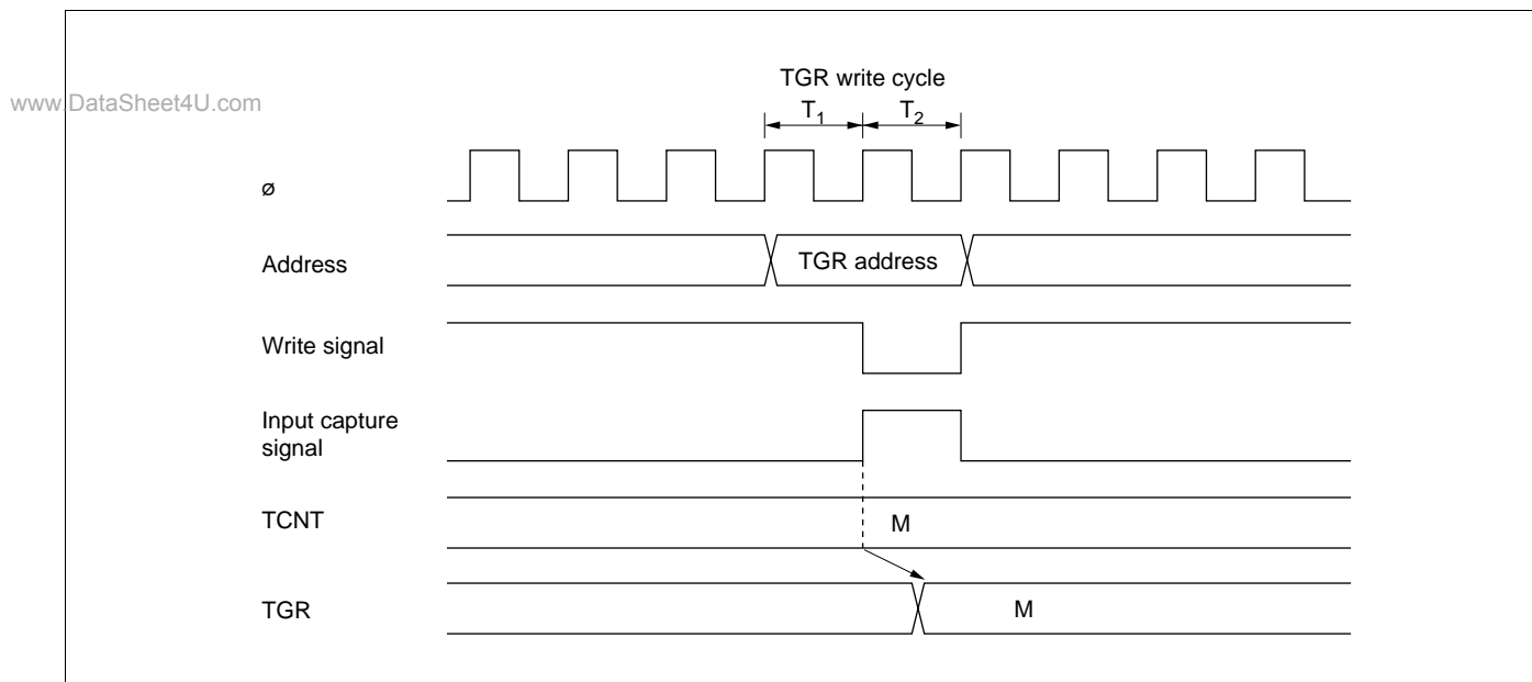
Figure 10-54 Contention between TGR Write and Input Capture
