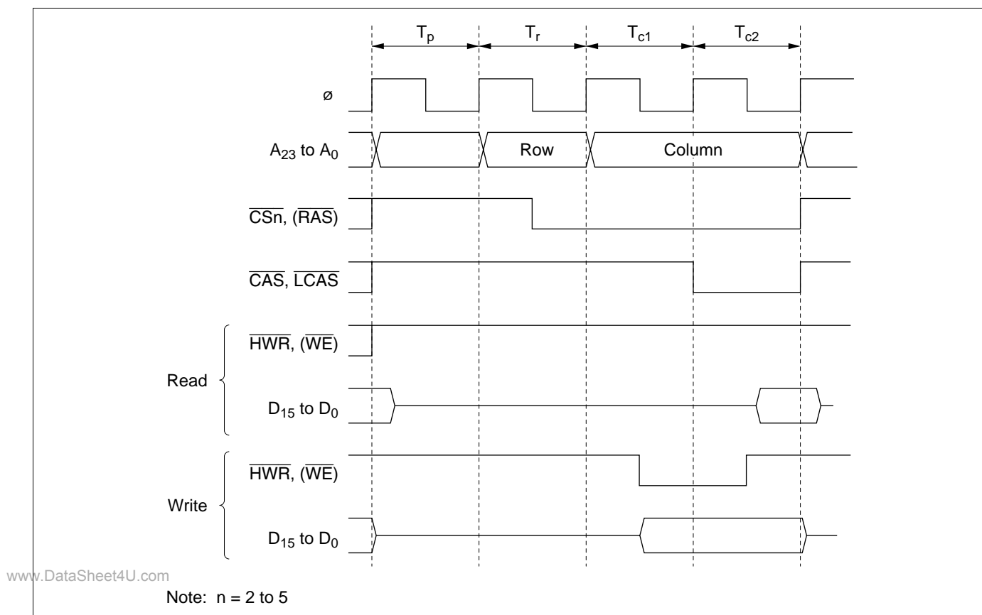
Figure 6-15 Basic Access Timing
