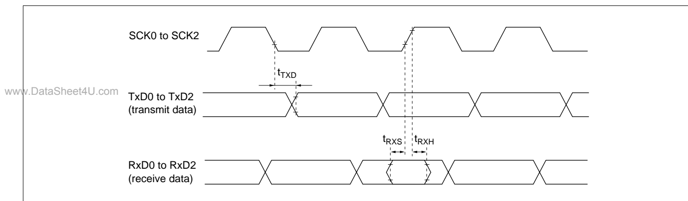
Figure 22-95 SCI Input/Output Timing (Clock Synchronous Mode)
