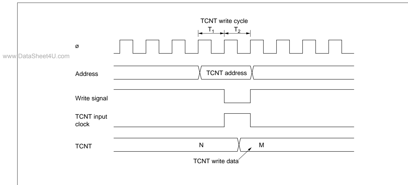
Figure 10-50 Contention between TCNT Write and Increment Operations
