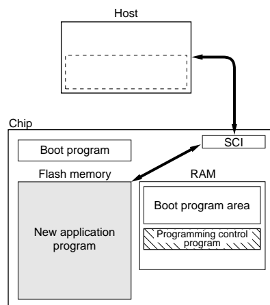
Figure 19-38 Boot Mode
