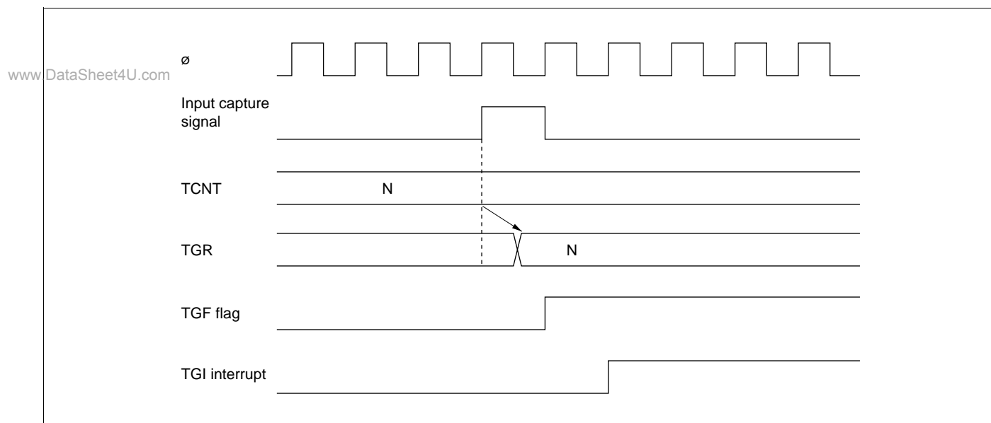
Figure 10-43 TGI Interrupt Timing (Input Capture)
