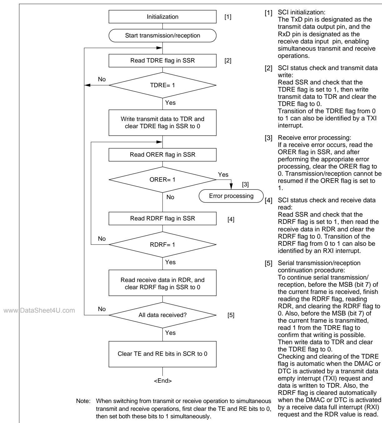
Figure 14-20 Sample Flowchart of Simultaneous Serial Transmit and Receive Operations
