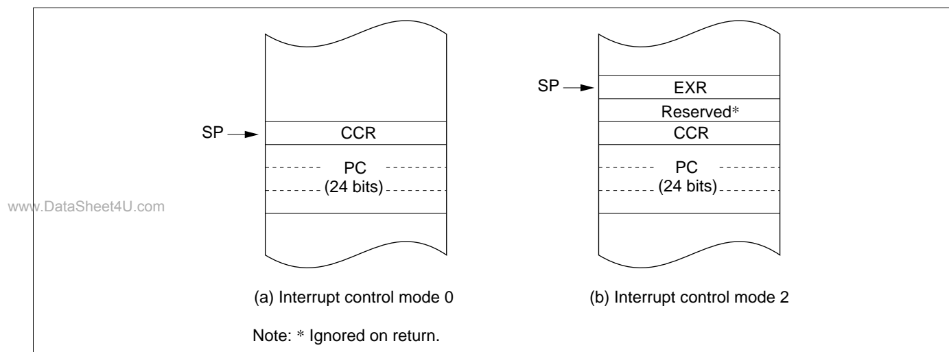
Figure 4-4 Stack Status after Exception Handling (Advanced Modes)
