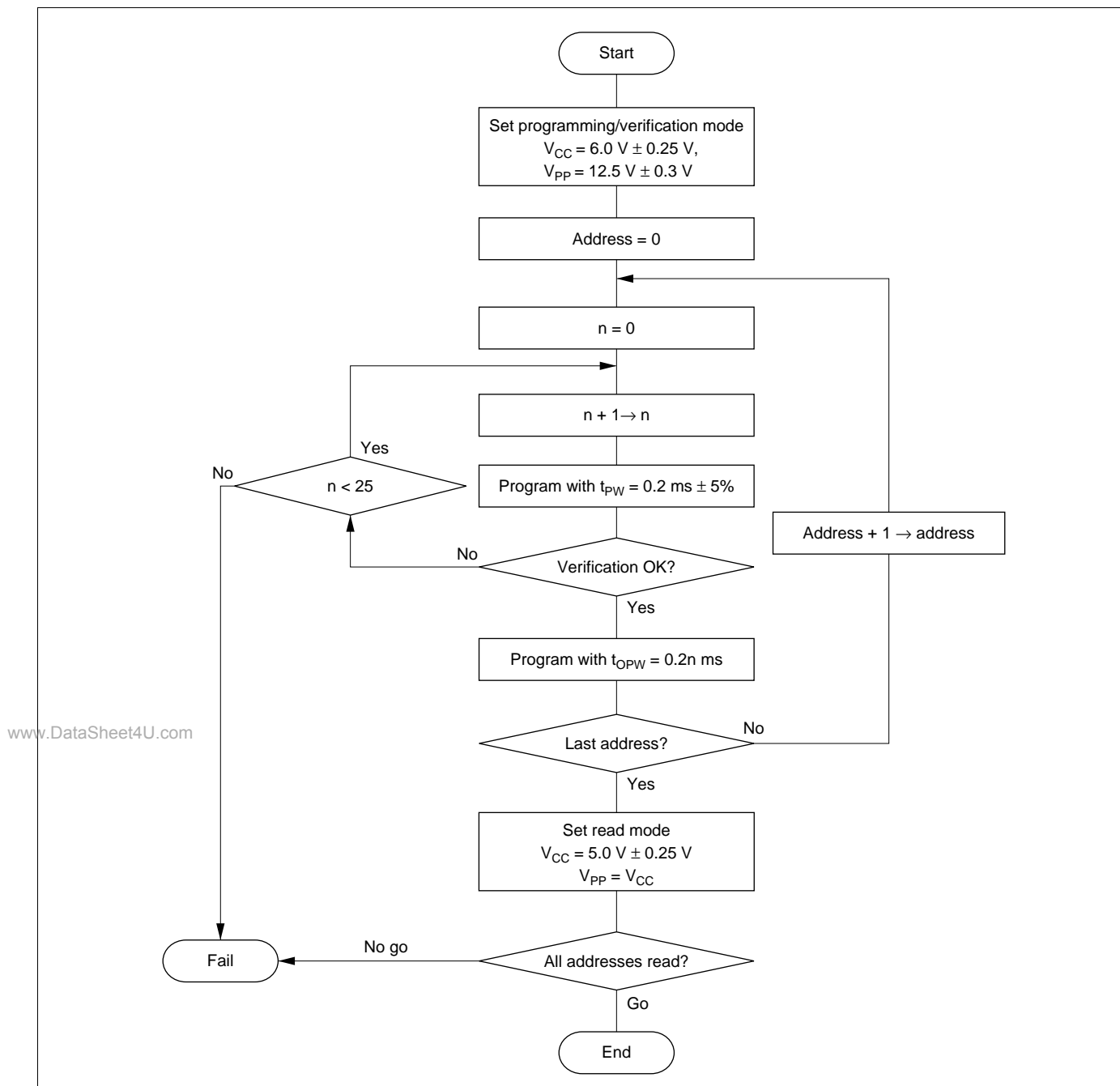
Figure 19-4 High-Speed Programming Flowchart
