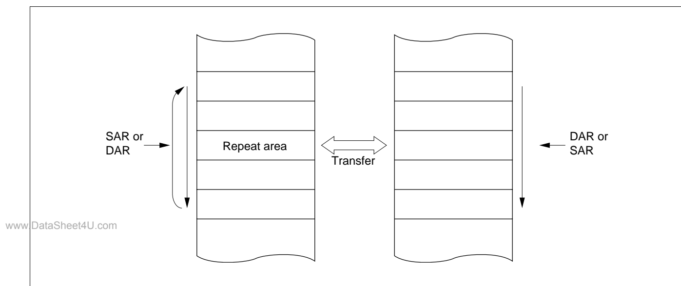
Figure 8-7 Memory Mapping in Repeat Mode
