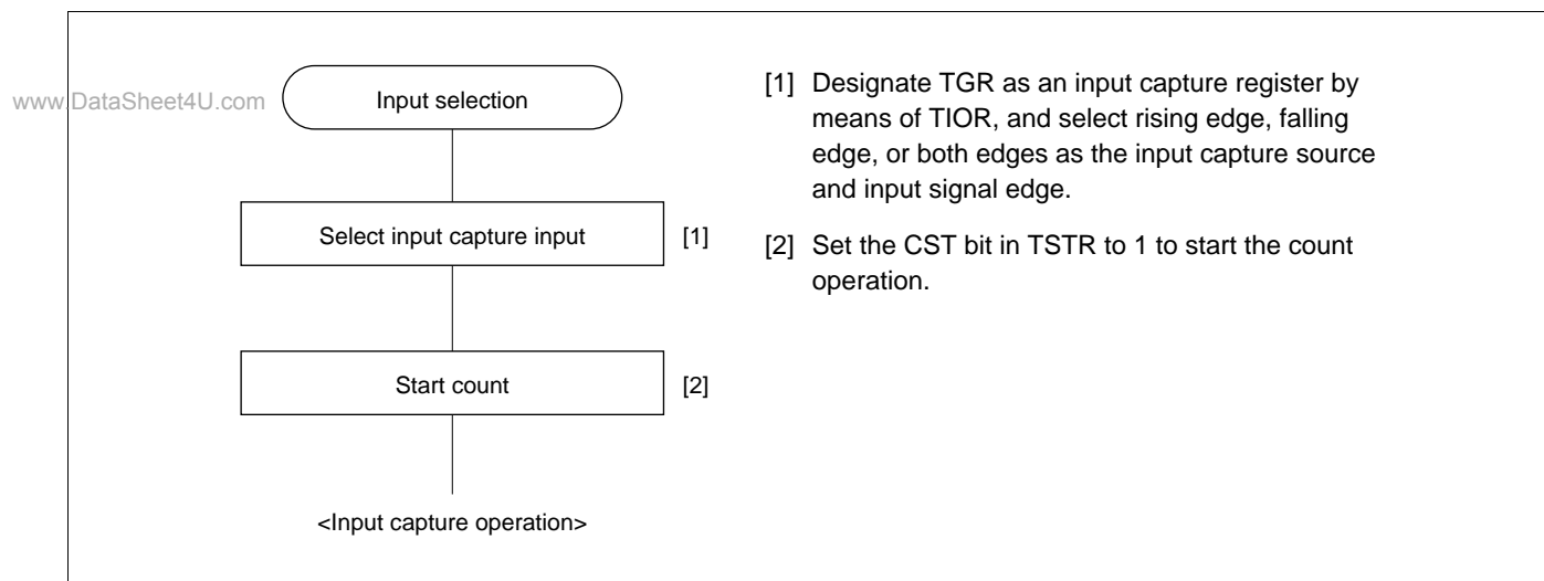
Figure 10-12 Example of Input Capture Operation Setting Procedure
