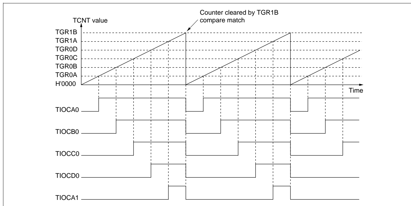
Figure 10-26 Example of PWM Mode Operation (2)
