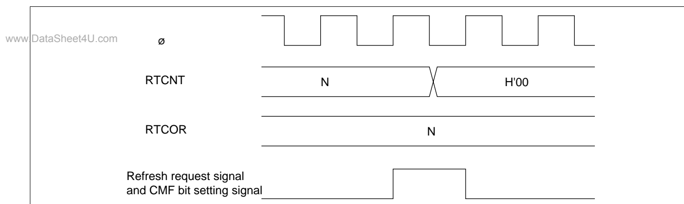
Figure 6-24 Compare Match Timing
