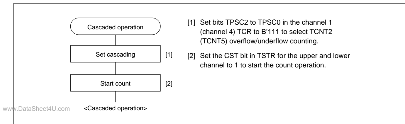
Figure 10-21 Cascaded Operation Setting Procedure
