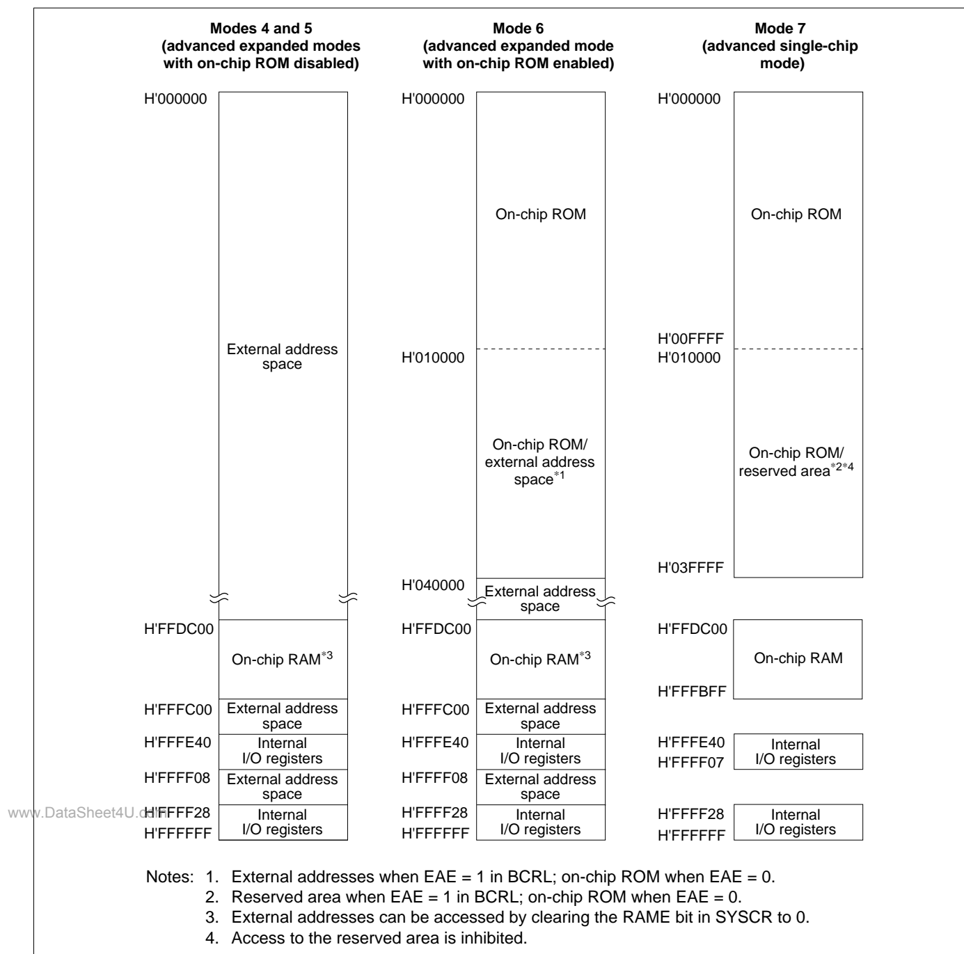
Figure 3-5 Memory Map in Each Operating Mode (H8S/2398) (2)
