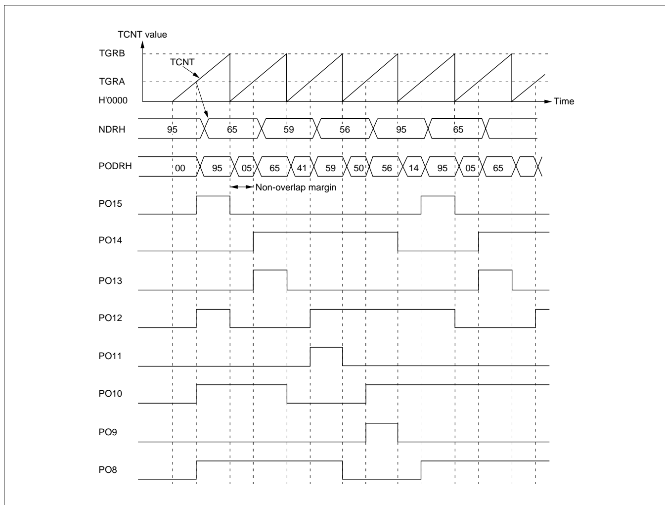
www.DataSheet4U.com Figure 11-7 Non-Overlapping Pulse Output Example (Four-Phase Complementary)
