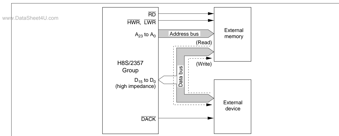
Figure 7-17 Data Bus in Single Address Mode
