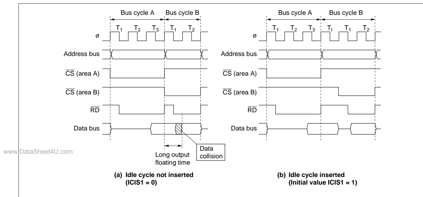
Figure 6-31 Example of Idle Cycle Operation (1)
