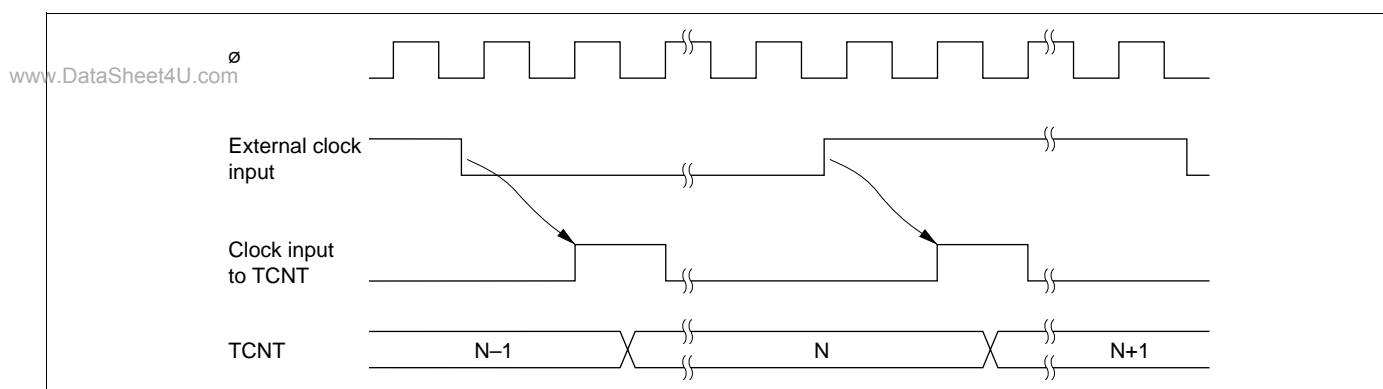
Figure 12-3 Count Timing for External Clock Input
