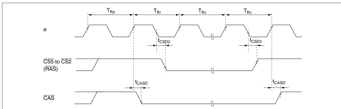
Figure 22-77 Self-Refresh Timing
