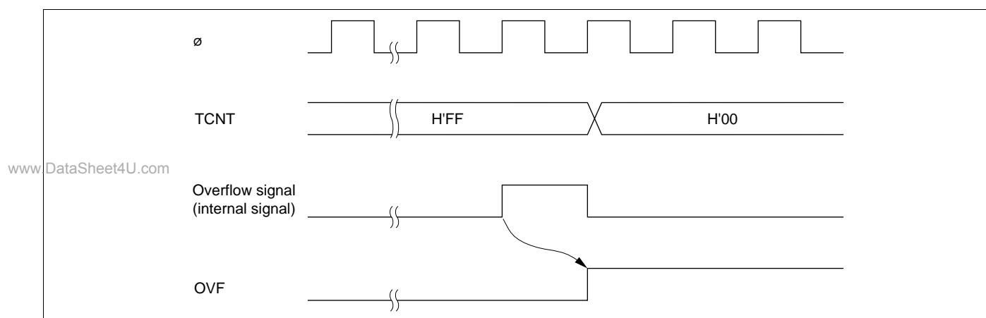
Figure 13-6 Timing of Setting of OVF
