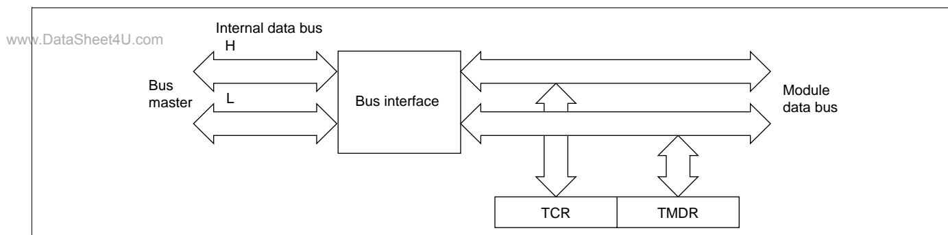
Figure 10-5 8-Bit Register Access Operation [Bus Master ↔ TCR and TMDR (16 Bits)]
