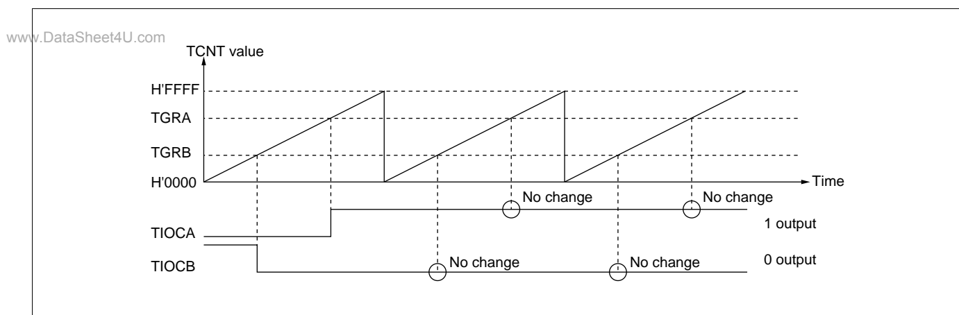
Figure 10-10 Example of 0 Output/1 Output Operation
