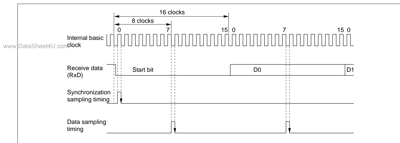
Figure 14-21 Receive Data Sampling Timing in Asynchronous Mode
