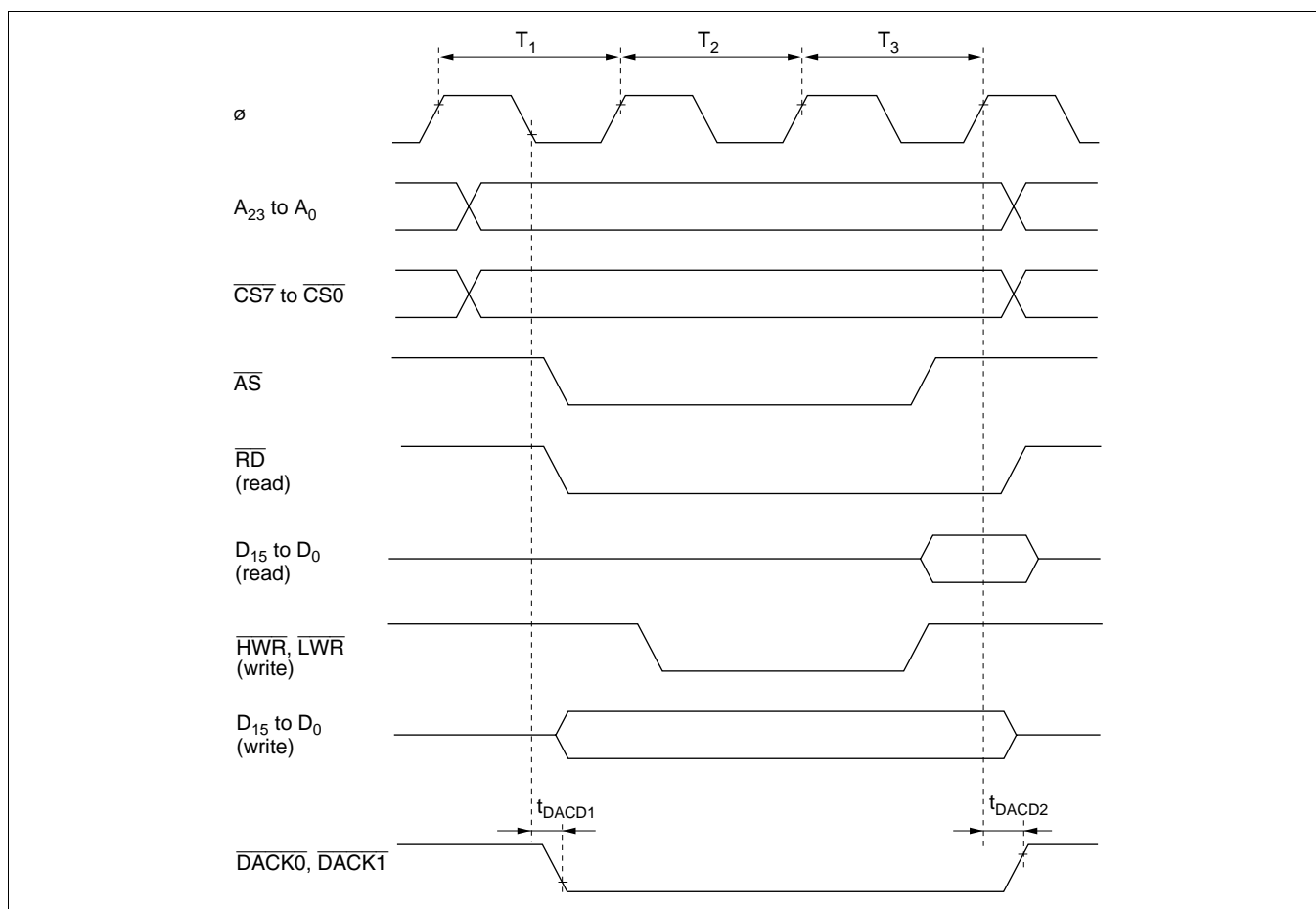
Figure 22-83 DMAC Single Address Transfer Timing (Three-State Access)
