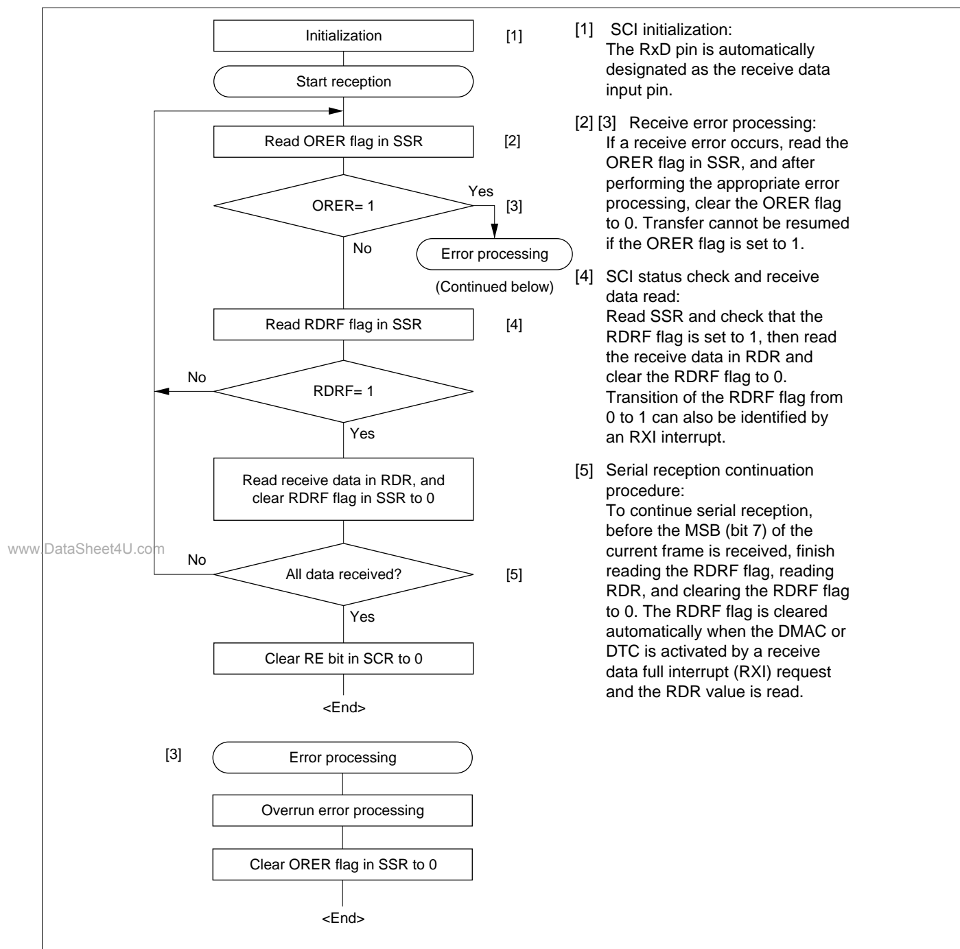
Figure 14-18 Sample Serial Reception Flowchart
