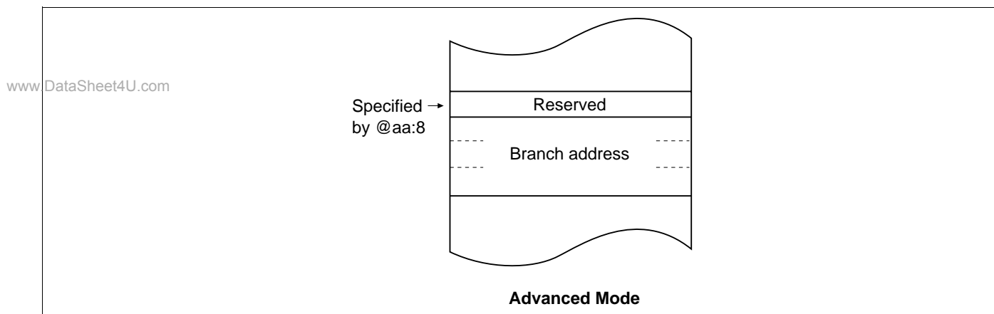
Figure 2-10 Branch Address Specification in Memory Indirect Mode
