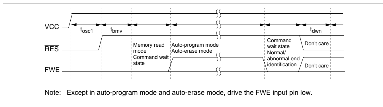
Figure 19-32 Oscillation Stabilization Time, Programmer Mode Setup Time, and Power Supply Fall Sequence
