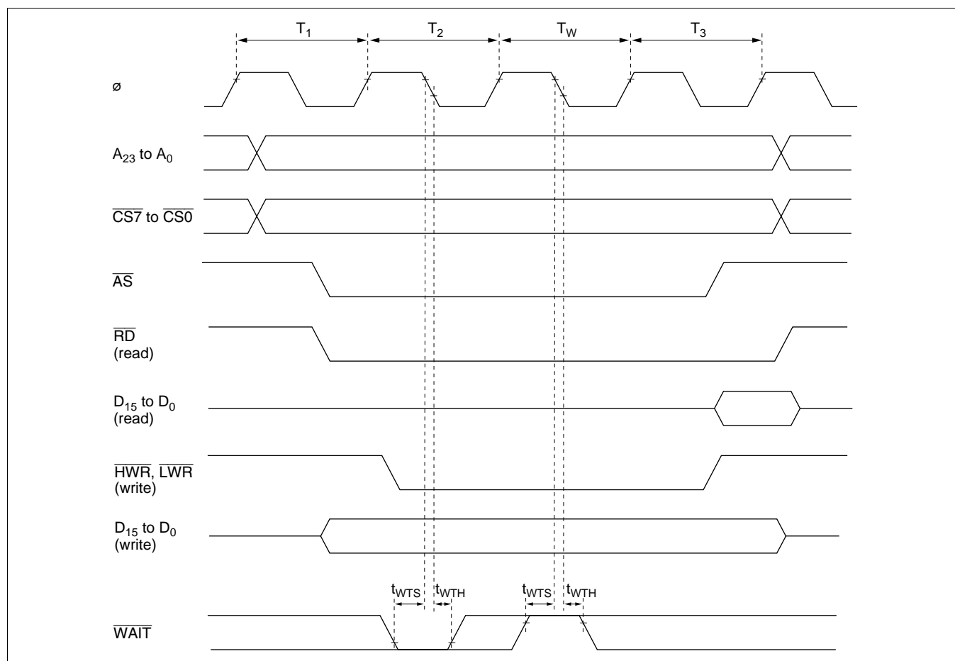
Figure 22-74 Basic Bus Timing (Three-State Access with One Wait State)
