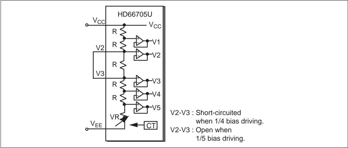
Figure 35 Contrast Adjuster
