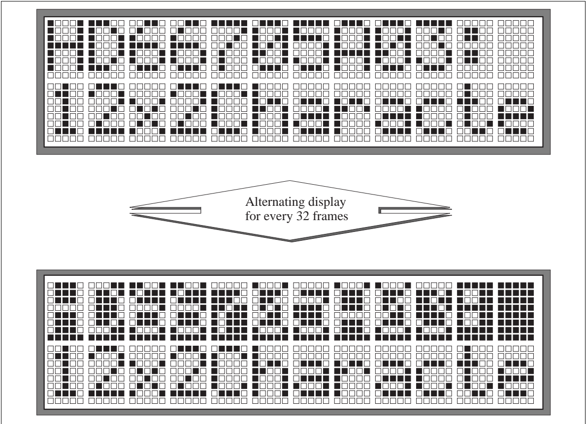
Figure 40 Example of Black-White Inverting Blink Cursor (LC = 1; B/W = 1)
