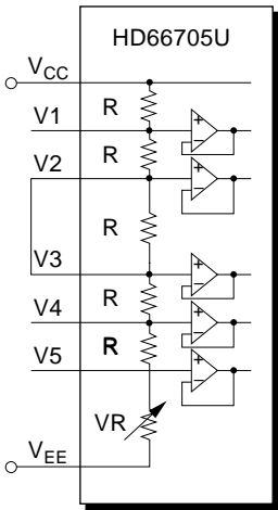
Figure 15 Contrast Adjuster
