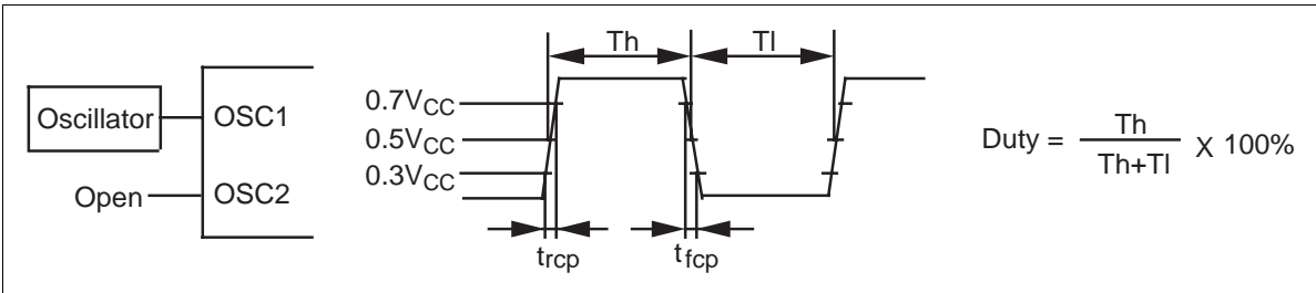
Figure 48 External Clock Supply
