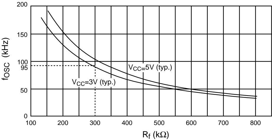
Figure 49 Internal Oscillation
