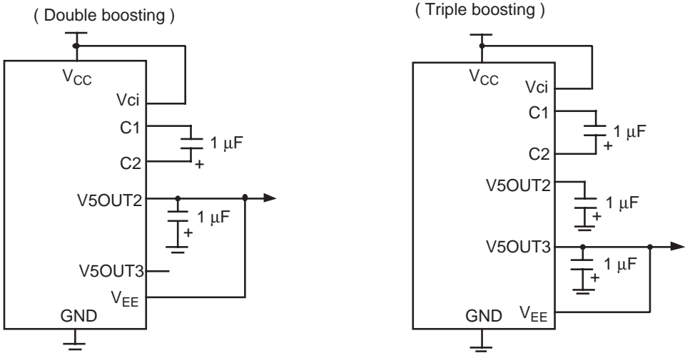
Figure 50 Booster
