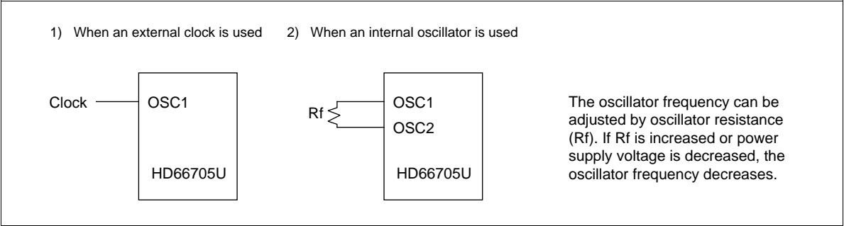
Figure 28 Oscillator Circuit
