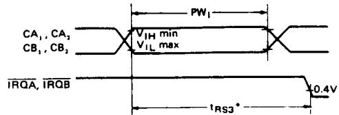
Figure 8 Interrupt Pulse Width and \overline{IRQ} Response
