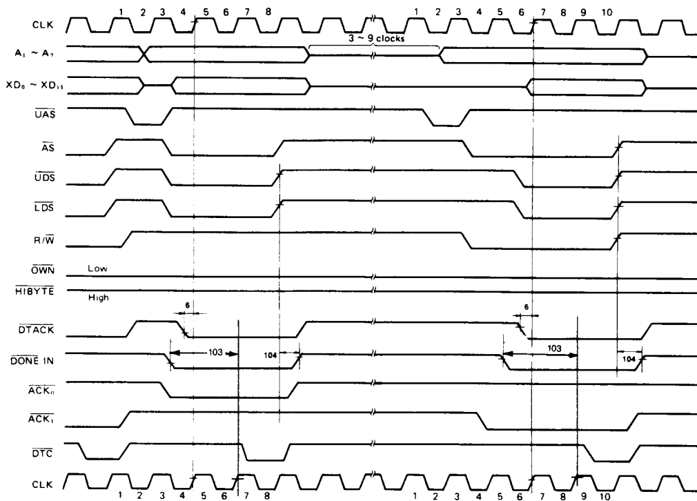
Figure 8 AC Electrical Waveforms – \overline{D0NE} Input
