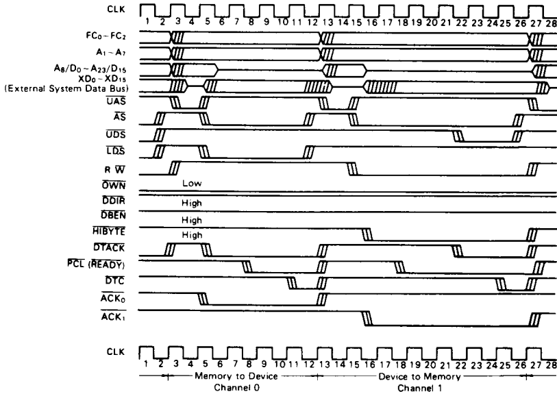
Figure 35 Single Addressing Mode with 8-Bit Devices as Source and Destination with PCL Used as a READY Input (Read-Write Cycles)
