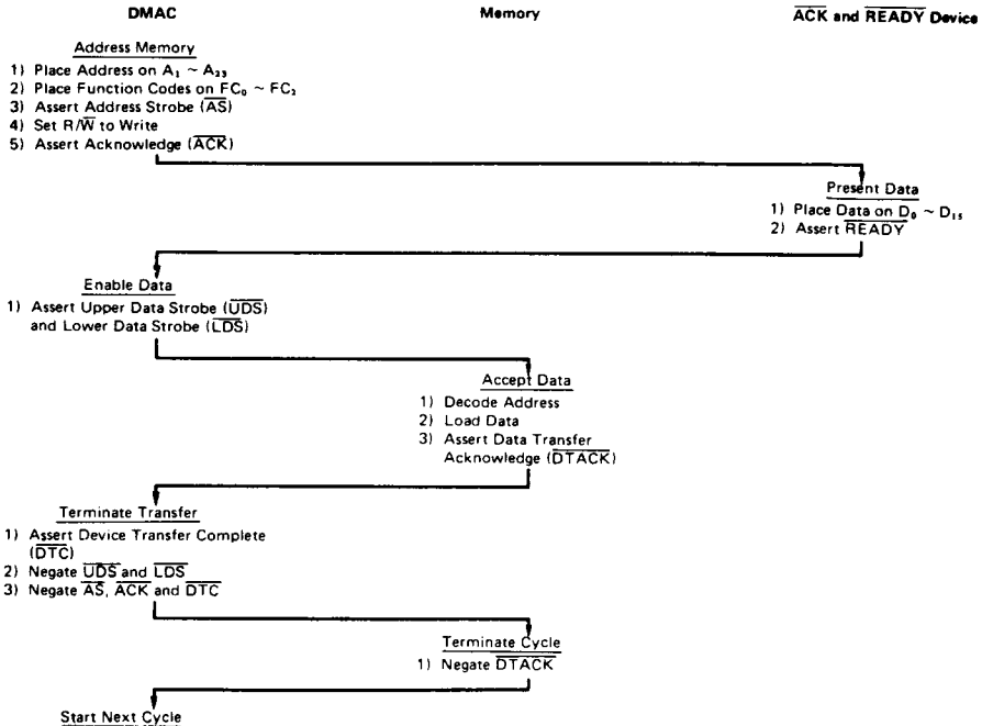
Figure 34 Word from Device with ACK and READY to Memory
