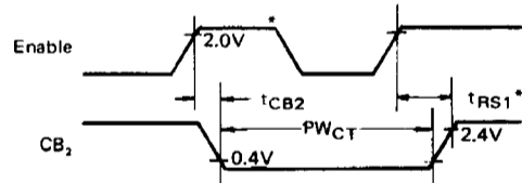
Figure 6 CB 2 Delay Time (Write Mode; CRB5=CRB3=1, CRB4=0)
