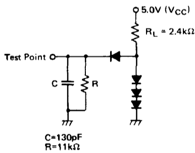
Figure 14 Bus Timing Test Loads
