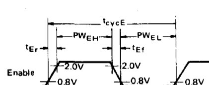
Figure 11 Enable Signal Characteristics
