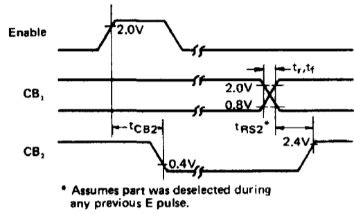
Figure 7 CB 2 Delay Time (Write Mode; CRB5=1, CRB3=CRB4=0)
