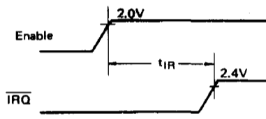
Figure 9 \overline{IRQ} Release Time
