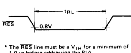
Figure 10 \overline{RES} Low Time
