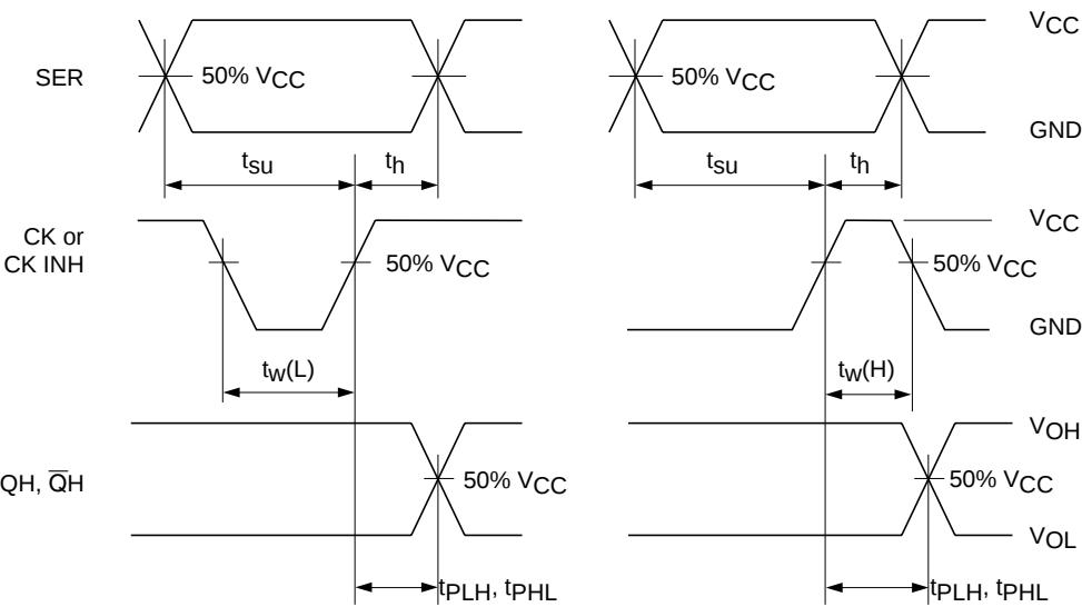
Waveform – 2
