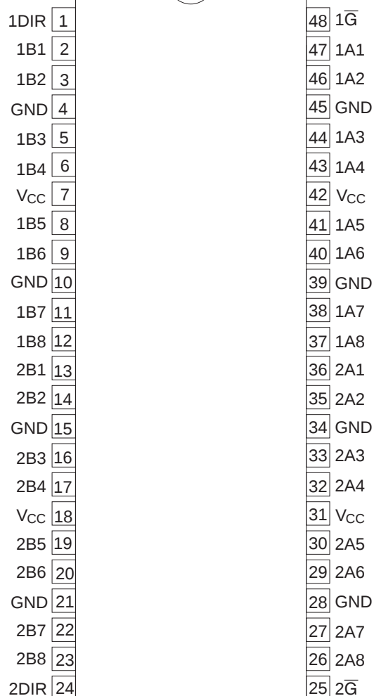
(Top view)
