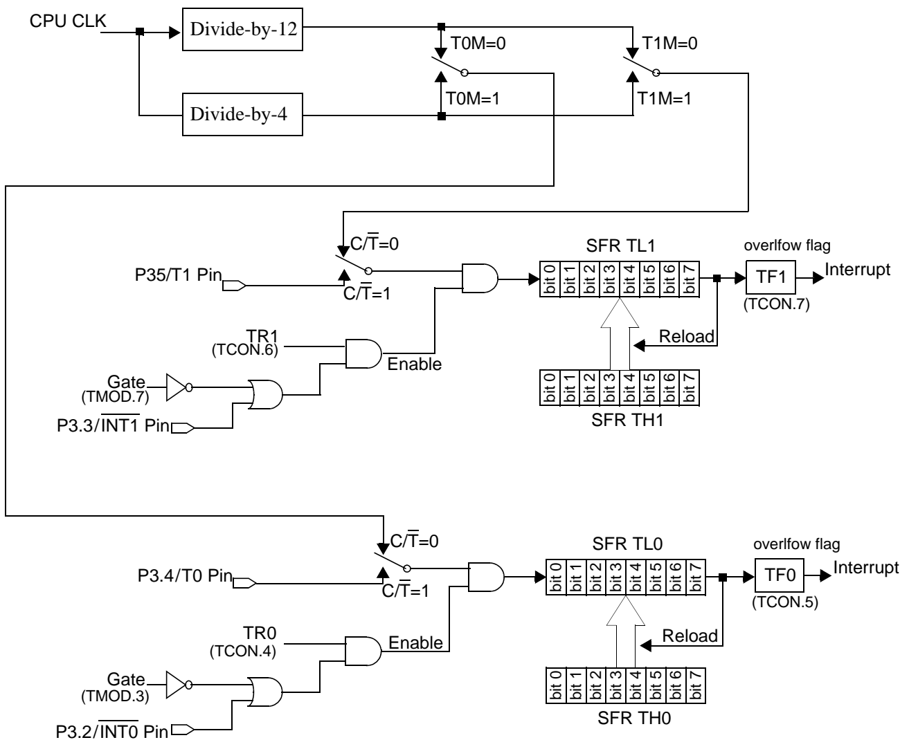
Fig.14 Mode 2 operation of Timer 0, Timer 1.
