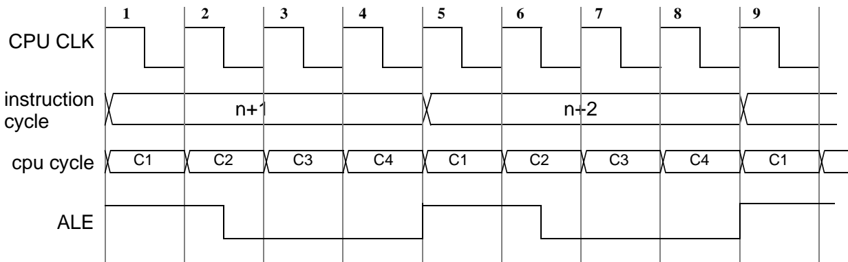
Fig.8 CPU instruction cycle.
