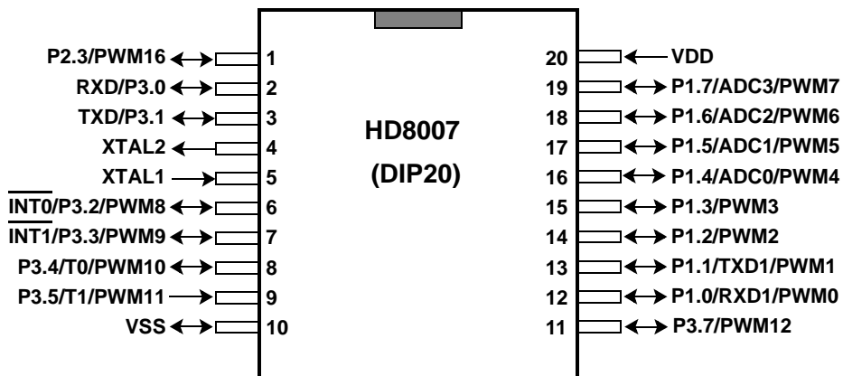
Fig.3 Pin configuration of DIP20 package.
