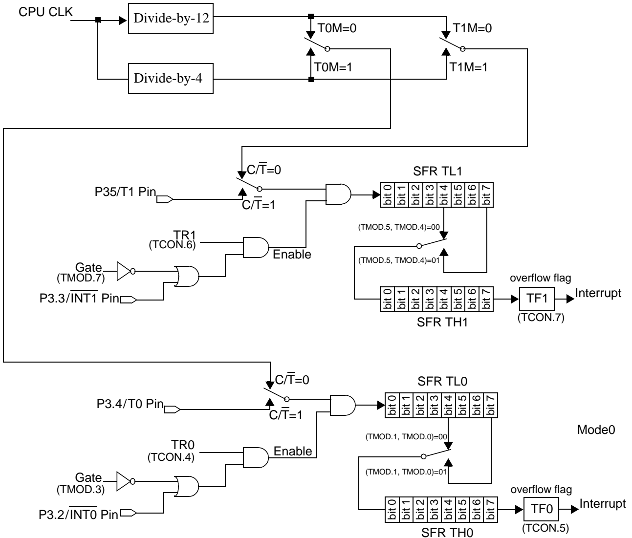
Fig.13 Mode 0 (13-bit timer/counter) and Mode 1 (16-bit timer/counter)
