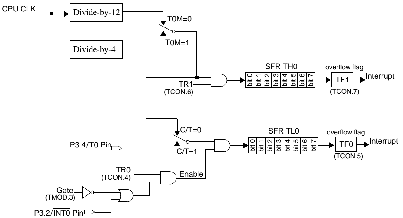
Fig.15 Mode 3 operation of Timer 0, Timer 1
