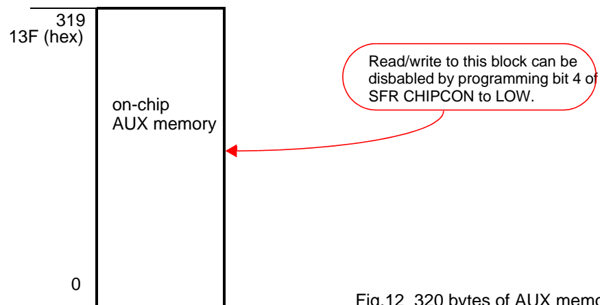
Fig.12 320 bytes of AUX memory
