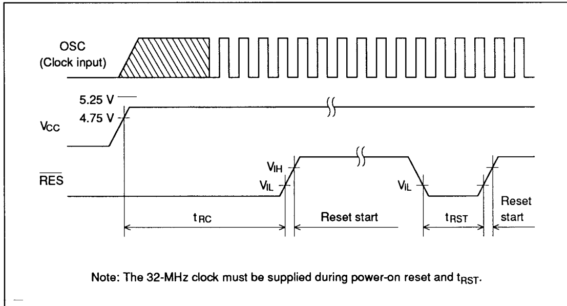
Figure 2 Reset Timing
