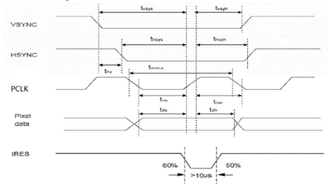
Figure 12. 1 Pixel Timing
