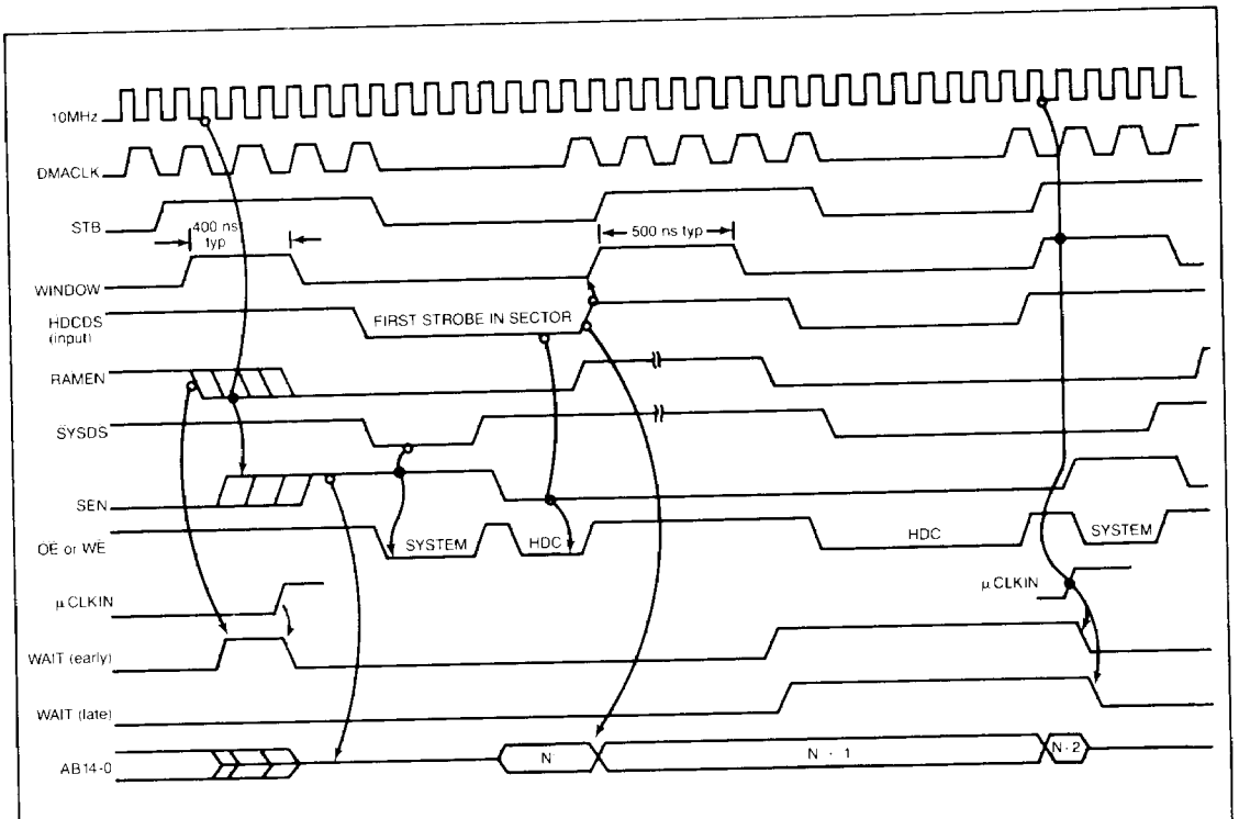
FIGURE A-PROCESSOR + HDC9224 CONTENTION TIMING FOR HARD DISK
