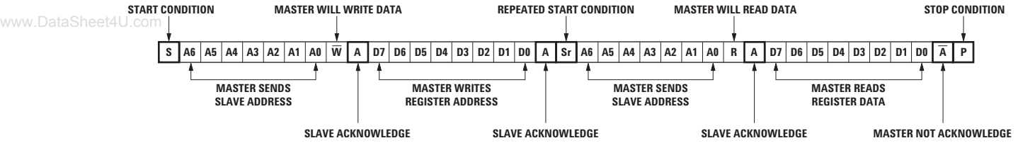
Figure 9. Register Byte Read Protocol.
