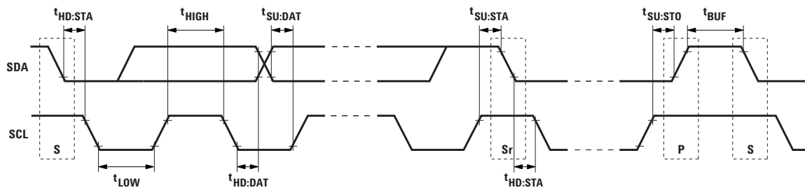
Figure 1. I 2 C bus timing waveforms.
