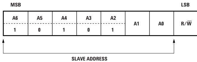
Figure 7. Slave addressing.
