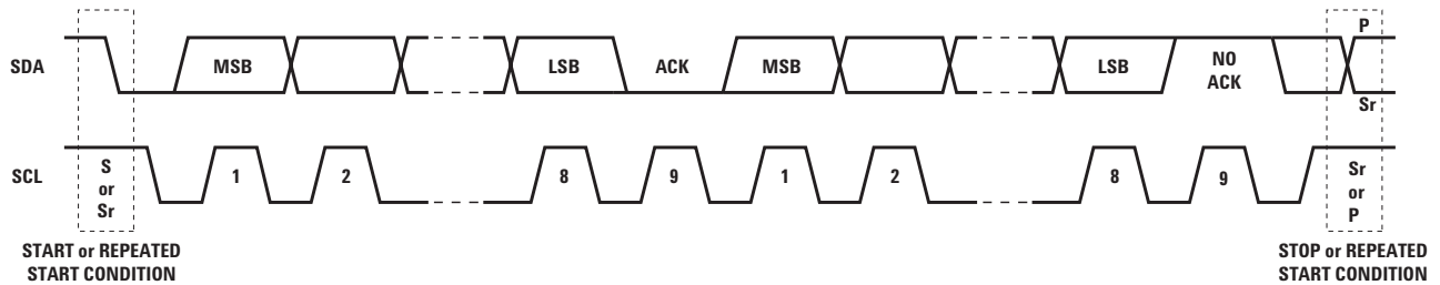
Figure 4. Data byte transfer.
