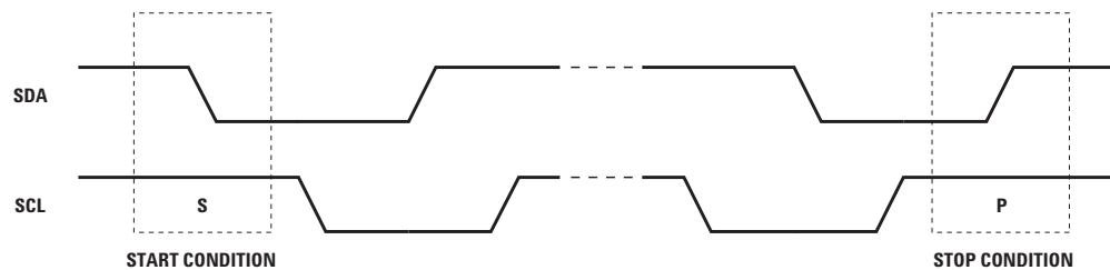
Figure 2. START/STOP condition.
