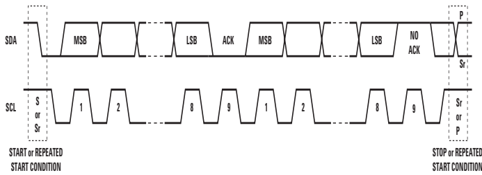
Figure 3. Data bit transfer.
