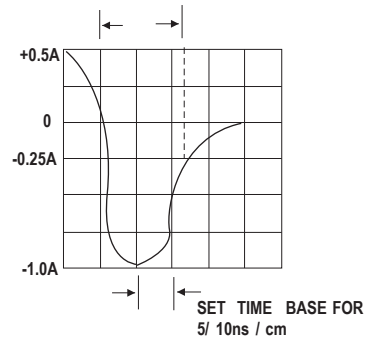
FIG . 3 -TYPICAL REVERSE CHARACTERISTICS
