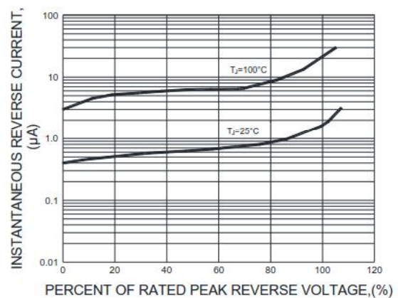
FIG.3-TYPICAL REVERSE CHARACTERISTICS
