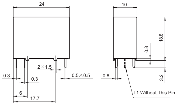
Outline Dimensions
