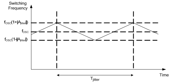
Figure 3: Frequency Jittering
