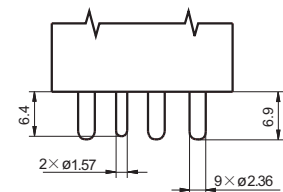
Terminal style 2 (Solder pin)
