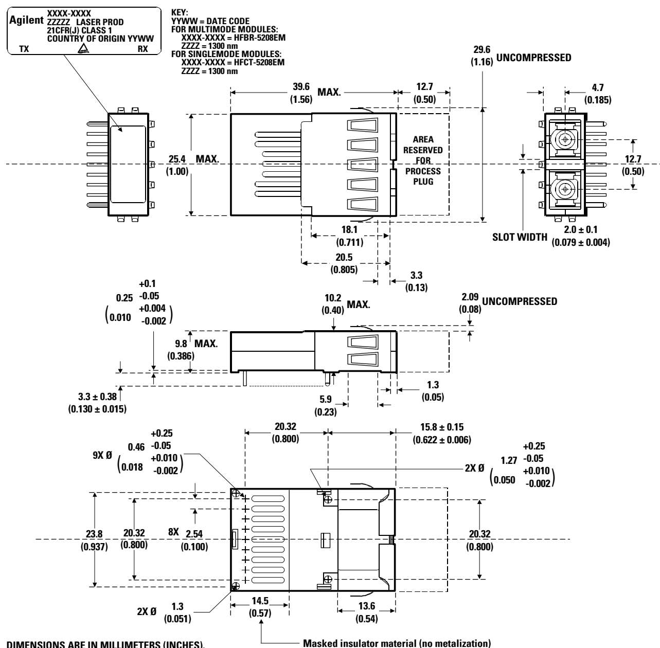
Figure 8. Package Outline for HFBR/HFCT-5208EM
