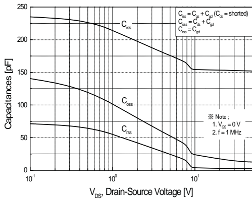
Figure 5. Capacitance Characteristics
