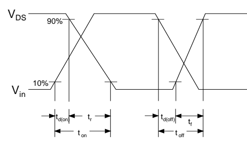
Fig 13. Resistive Switching Test Circuit & Waveforms
