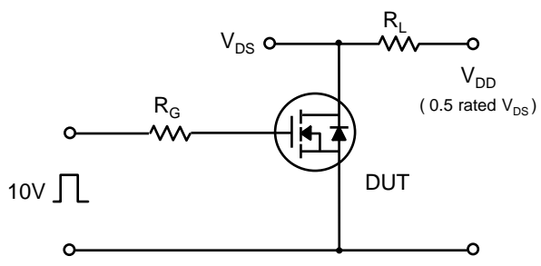
Fig 13. Resistive Switching Test Circuit & Waveforms
