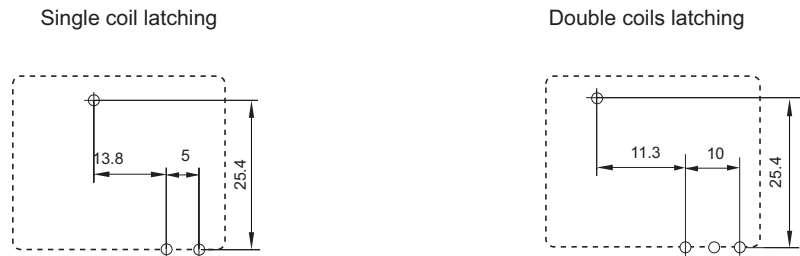
Wiring Diagram (Bottom view)
