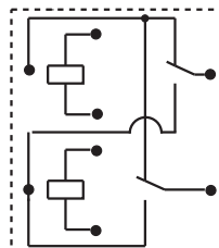
2 Form C (Twin(H-bridge) relay)
