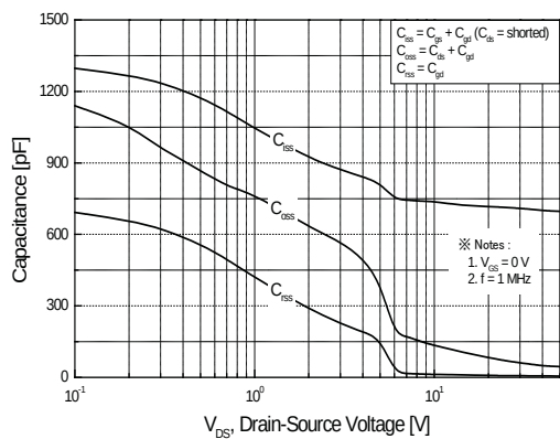
Figure 5. Capacitance Characteristics
