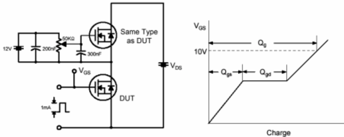
Fig 13. Switching Time Test Circuit &amp; Waveforms
