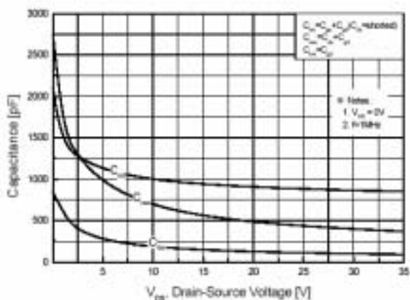
Fig 5. Capacitance Characteristics
