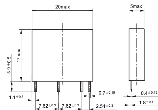
Outline Dimensions
