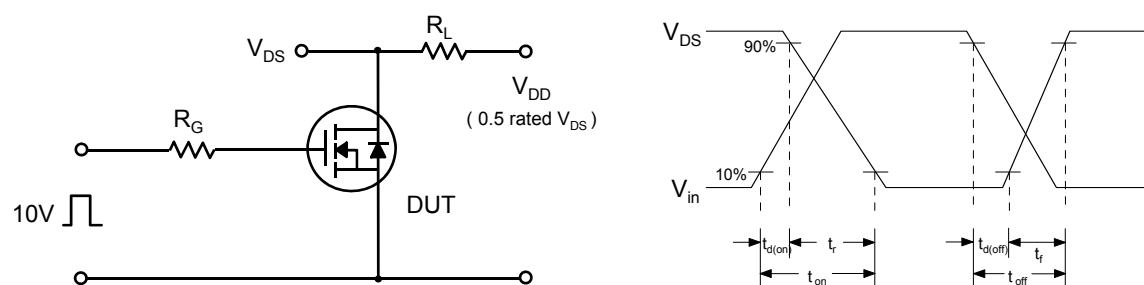
Fig 13. Resistive Switching Test Circuit &amp; Waveforms
