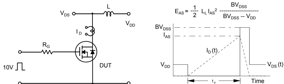
Fig 14. Unclamped Inductive Switching Test Circuit &amp; Waveforms
