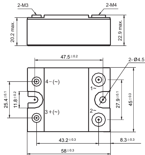
Outline Dimensions
