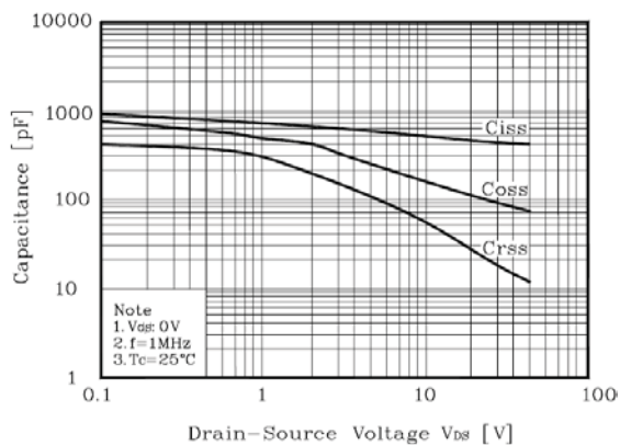
Figure 5. Capacitance Characteristics
