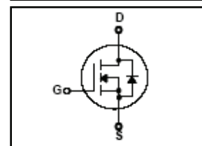
HFD6N70U
